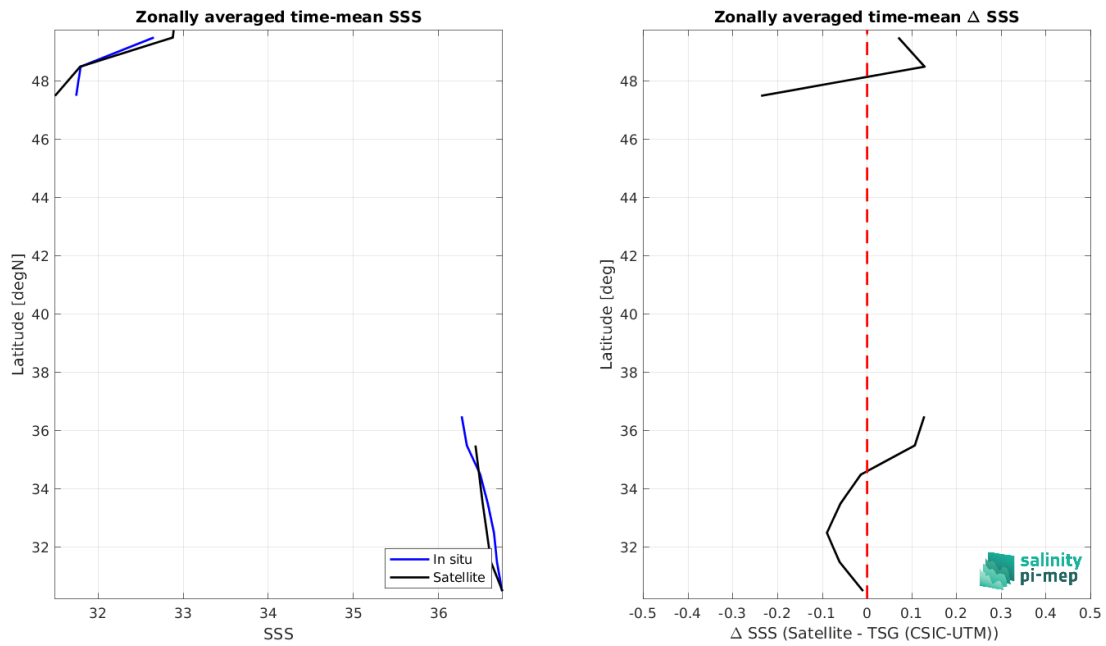
Figure 9: Left panel: Zonal mean SSS from ISAS v7 - Monthly (Ifremer-LOPS-CMEMS) satellite product (black) and from TSG (CSIC-UTM) (blue). Right panel: Zonal mean of \Delta SSS (Satellite - TSG (CSIC-UTM)) for all the collected Pi-MEP match-up pairs estimated over the full satellite product period.
