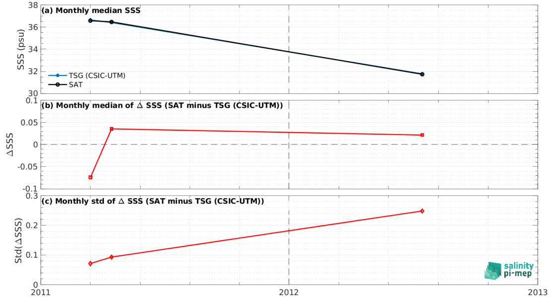
Figure 8: Time series of the monthly median SSS (top), median of \Delta\text{SSS} (Satellite - TSG (CSIC-UTM)) and Std of \Delta\text{SSS} (Satellite - TSG (CSIC-UTM)) over the Gulf Stream Pi-MEP region considering all match-ups collected by the Pi-MEP.
