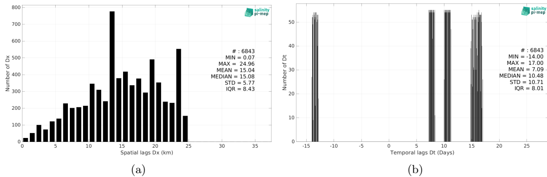
Figure 6: Histograms of the spatial (a) and temporal (b) lags between the location/time of the TSG (CSIC-UTM) measurement and the date of the corresponding ISAS v7 - Monthly (Ifremer-LOPS-CMEMS) SSS pixel.
