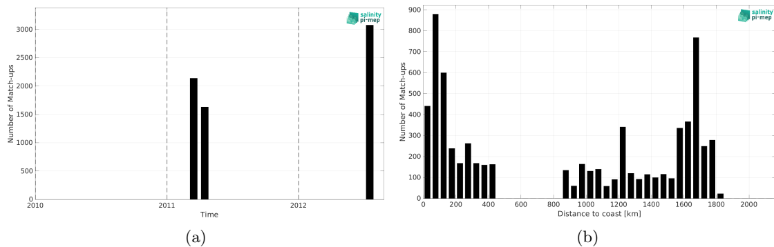
Figure 2: Number of match-ups between TSG (CSIC-UTM) and ISAS v7 - Monthly (Ifremer-LOPS-CMEMS) SSS as a function of time (a) and as function of the distance to coast (b) over the Gulf Stream Pi-MEP region and for the full satellite product period.
