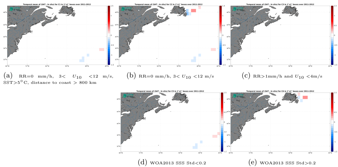
Figure 14: Temporal mean gridded over spatial boxes of size 1^\circ \times 1^\circ of \Delta SSS (ISAS v7 - Monthly (Ifremer-LOPS-CMEMS) - TSG (CSIC-UTM)) for 5 different subdatasets corresponding to: RR=0 mm/h, 3 < U_{10} < 12 m/s, SST > 5°C, distance to coast > 800 km (a), RR=0 mm/h, 3 < U_{10} < 12 m/s (b), RR > 1mm/h and U_{10} < 4 m/s (c), WOA2013 SSS Std < 0.2 (d), WOA2013 SSS Std > 0.2 (e).
