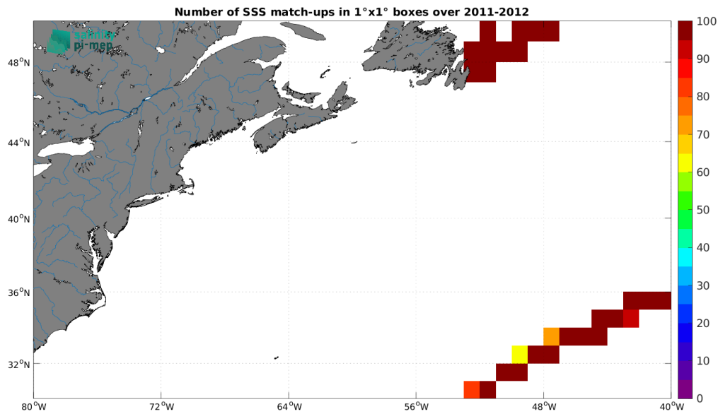
Figure 5: Number of SSS match-ups between TSG (CSIC-UTM) SSS and the ISAS v7 - Monthly (Ifremer-LOPS-CMEMS) SSS product for the Gulf Stream Pi-MEP region over 1^\circ \times 1^\circ boxes and for the full satellite product period.
