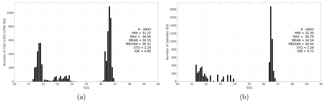
Figure 3: Histograms of SSS from TSG (CSIC-UTM) (a) and ISAS v7 - Monthly (Ifremer-LOPS-CMEMS) (b) considering all match-up pairs per bins of 0.1 over the Gulf Stream Pi-MEP region and for the full satellite product period.
