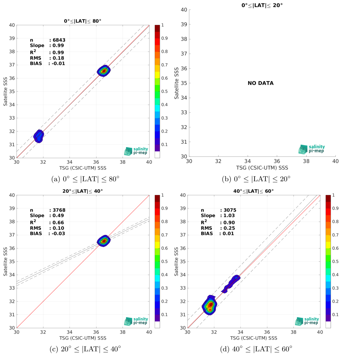
Figure 10: Contour maps of the concentration of ISAS v7 - Monthly (Ifremer-LOPS-CMEMS) SSS (y-axis) versus TSG (CSIC-UTM) SSS (x-axis) at match-up pairs for different latitude bands. For each plot, the red line shows x=y . The black thin and dashed lines indicate a linear fit through the data cloud and the \pm 95\% confidence levels, respectively. The number match-up pairs n , the slope and R^2 coefficient of the linear fit, the root mean square (RMS) and the mean bias between satellite and in situ data are indicated for each latitude band in each plots.
