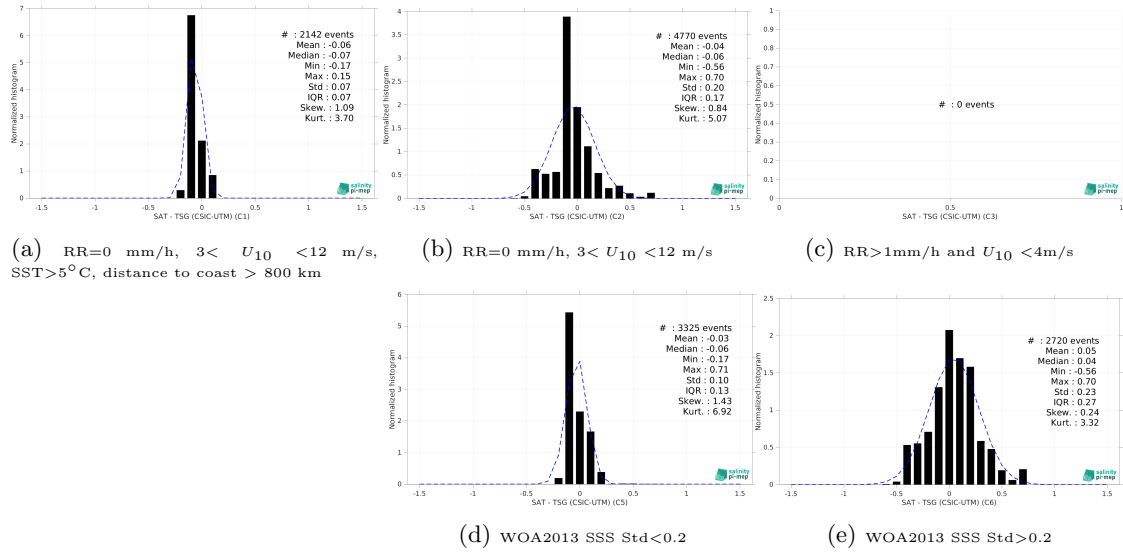
Figure 15: Normalized histogram of \Delta SSS (ISAS v7 - Monthly (Ifremer-LOPS-CMEMS) - TSG (CSIC-UTM)) for 5 different subdatasets corresponding to: RR=0 mm/h, 3 < U_{10} < 12 m/s, SST>5°C, distance to coast > 800 km (a), RR=0 mm/h, 3 < U_{10} < 12 m/s (b), RR>1mm/h and U_{10} < 4 m/s (c), WOA2013 SSS Std<0.2 (d), WOA2013 SSS Std>0.2 (e).
