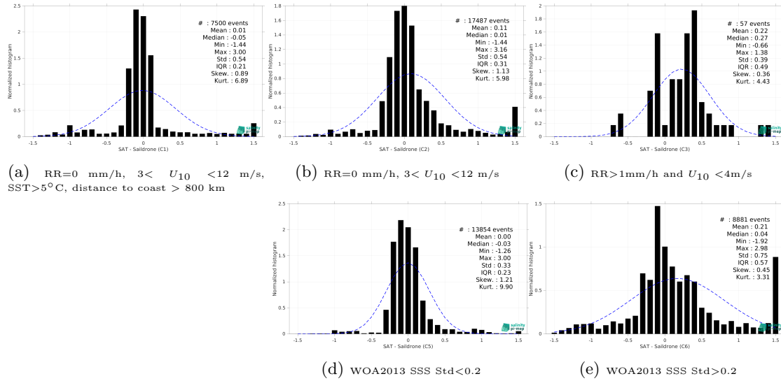
Figure 15: Normalized histogram of \Delta SSS (ISAS v7 - Monthly (Ifremer-LOPS-CMEMS) - Saldrone) for 5 different subdatasets corresponding to: RR=0 mm/h, 3 < U_{10} < 12 m/s, SST>5°C, distance to coast > 800 km (a), RR=0 mm/h, 3 < U_{10} < 12 m/s (b), RR>1mm/h and U_{10} < 4 m/s (c), WOA2013 SSS Std<0.2 (d), WOA2013 SSS Std>0.2 (e).
