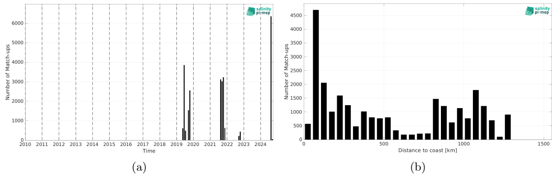
Figure 2: Number of match-ups between Saildrone and ISAS v7 - Monthly (Ifremer-LOPS-CMEMS) SSS as a function of time (a) and as function of the distance to coast (b) over the Gulf Stream Pi-MEP region and for the full satellite product period.
