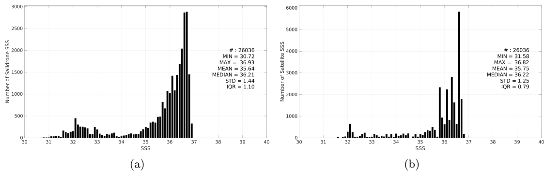
Figure 3: Histograms of SSS from Saildrone (a) and ISAS v7 - Monthly (Ifremer-LOPS-CMEMS) (b) considering all match-up pairs per bins of 0.1 over the Gulf Stream Pi-MEP region and for the full satellite product period.
