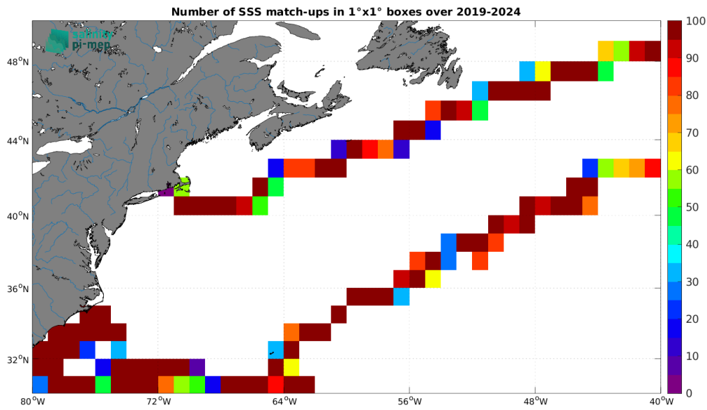
Figure 5: Number of SSS match-ups between Saildrone SSS and the ISAS v7 - Monthly (Ifremer-LOPS-CMEMS) SSS product for the Gulf Stream Pi-MEP region over 1^\circ \times 1^\circ boxes and for the full satellite product period.
