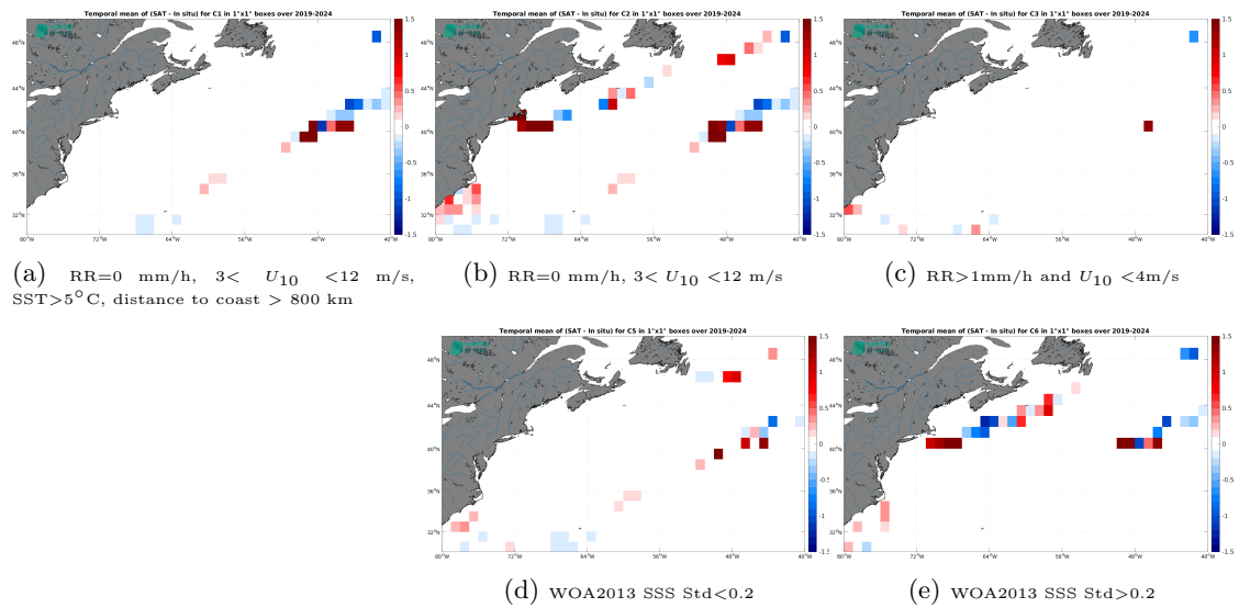
Figure 14: Temporal mean gridded over spatial boxes of size 1^\circ \times 1^\circ of \Delta SSS (ISAS v7 - Monthly (Ifremer-LOPS-CMEMS) - Saildrone) for 5 different subdatasets corresponding to:RR=0 mm/h, 3 < U_{10} < 12 m/s, SST>5°C, distance to coast > 800 km (a), RR=0 mm/h, 3 < U_{10} < 12 m/s (b), RR>1mm/h and U_{10} < 4 m/s (c), WOA2013 SSS Std<0.2 (d), WOA2013 SSS Std>0.2 (e).
