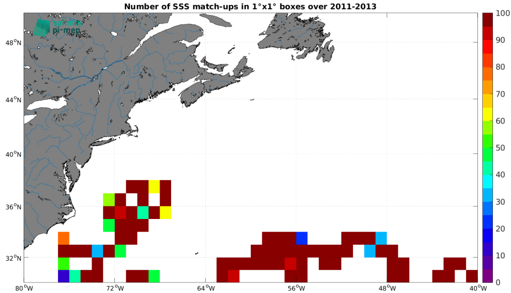
Figure 4: Number of SSS match-ups between Surface drifters SSS and the ISAS v7 - Monthly (Ifremer-LOPS-CMEMS) SSS product for the Gulf Stream Pi-MEP region over 1^\circ \times 1^\circ boxes and for the full satellite product period.
