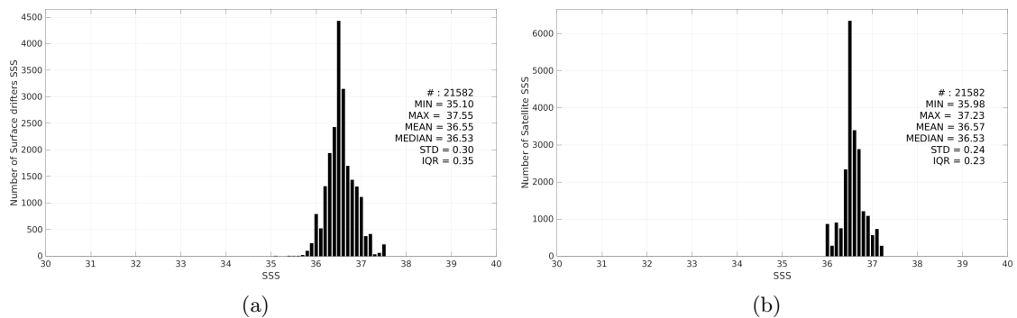
Figure 3: Histograms of SSS from Surface drifters (a) and ISAS v7 - Monthly (Ifremer-LOPS-CMEMS) (b) considering all match-up pairs per bins of 0.1 over the Gulf Stream Pi-MEP region and for the full satellite product period.
