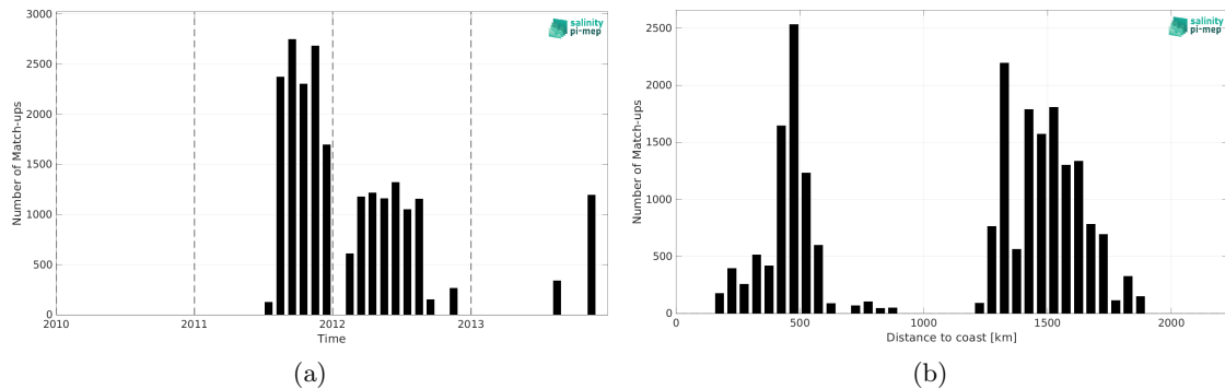
Figure 2: Number of match-ups between Surface drifters and ISAS v7 - Monthly (Ifremer-LOPS-CMEMS) SSS as a function of time (a) and as function of the distance to coast (b) over the Gulf Stream Pi-MEP region and for the full satellite product period.
