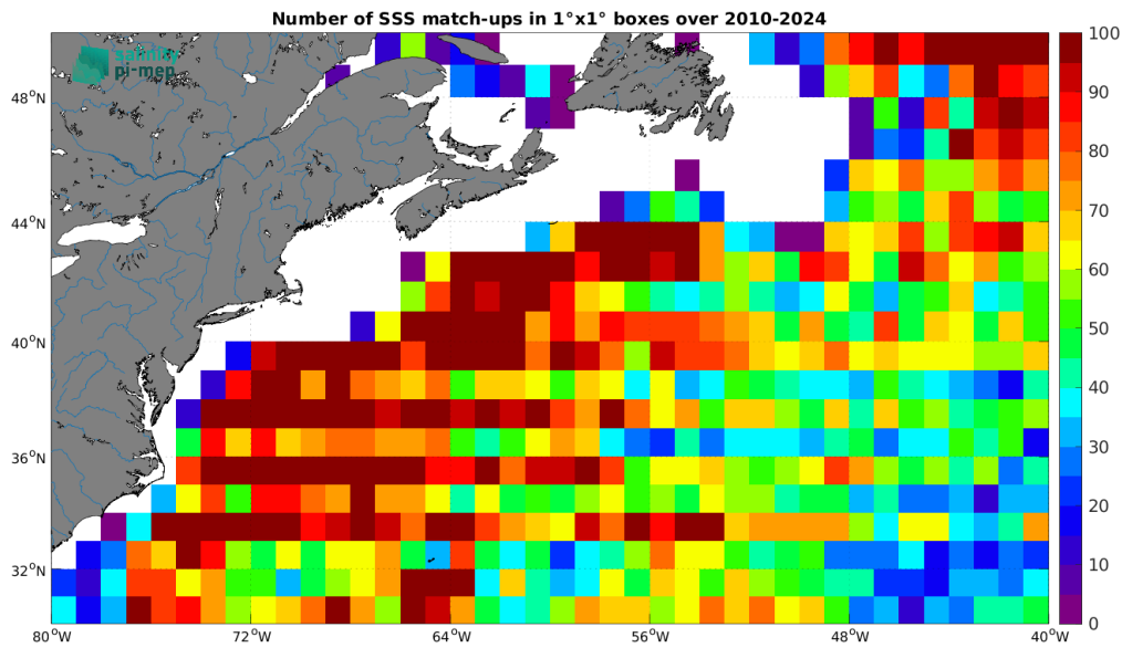
Figure 5: Number of SSS match-ups between Argo SSS and the ISAS v7 - Monthly (Ifremer-LOPS-CMEMS) SSS product for the Gulf Stream Pi-MEP region over 1^\circ \times 1^\circ boxes and for the full satellite product period.
