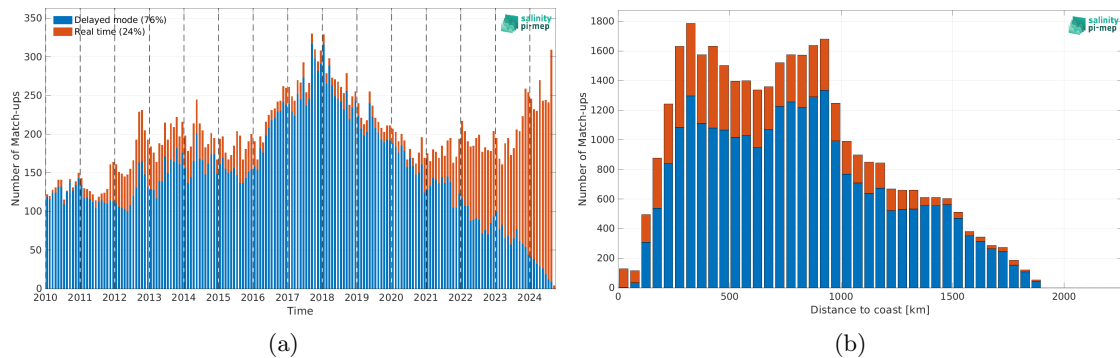
Figure 2: Number of match-ups between Argo and ISAS v7 - Monthly (Ifremer-LOPS-CMEMS) SSS as a function of time (a) and as function of the distance to coast (b) over the Gulf Stream Pi-MEP region and for the full satellite product period.
