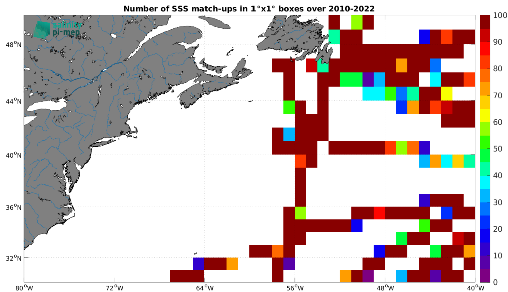
Figure 5: Number of SSS match-ups between TSG (GOSUD-Research-vessel) SSS and the CCI SSS L4 Merged-OI v5.5 - 7-day running (ESA) SSS product for the Gulf Stream Pi-MEP region over 1^\circ \times 1^\circ boxes and for the full satellite product period.
