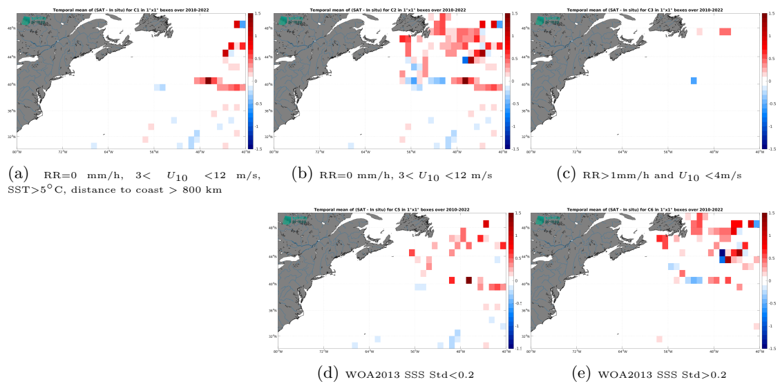
Figure 14: Temporal mean gridded over spatial boxes of size 1^\circ \times 1^\circ of \Delta SSS (CCI SSS L4 Merged-OI v5.5 - 7-day running (ESA) - TSG (GOSUD-Research-vessel)) for 5 different subdatasets corresponding to:RR=0 mm/h, 3 < U_{10} < 12 m/s, SST>5°C, distance to coast > 800 km (a), RR=0 mm/h, 3 < U_{10} < 12 m/s (b), RR>1mm/h and U_{10} < 4 m/s (c), WOA2013 SSS Std<0.2 (d), WOA2013 SSS Std>0.2 (e).
