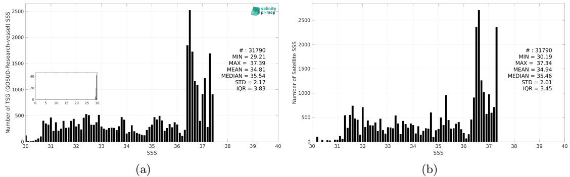
Figure 3: Histograms of SSS from TSG (GOSUD-Research-vessel) (a) and CCI SSS L4 Merged-OI v5.5 - 7-day running (ESA) (b) considering all match-up pairs per bins of 0.1 over the Gulf Stream Pi-MEP region and for the full satellite product period.
