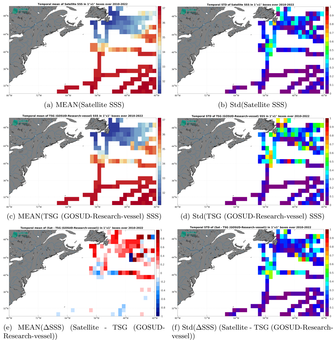
Figure 7: Temporal mean (left) and Std (right) of SSS from CCI SSS L4 Merged-OI v5.5 - 7-day running (ESA) (top), TSG (GOSUD-Research-vessel) (middle), and of \Delta SSS (Satellite - TSG (GOSUD-Research-vessel)). Only match-up pairs are used to generate these maps.
