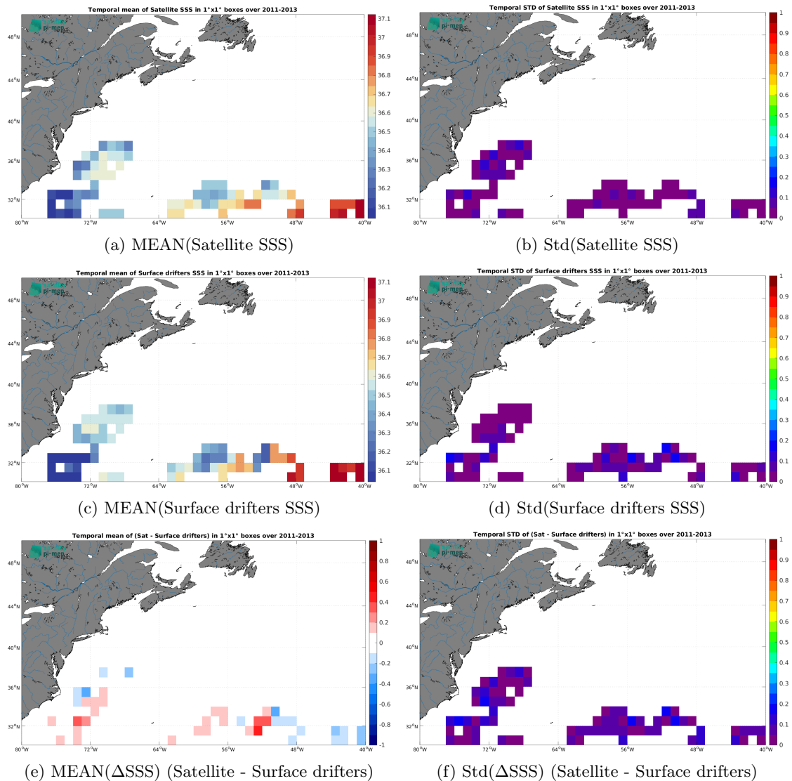
Figure 6: Temporal mean (left) and Std (right) of SSS from CCI SSS L4 Merged-OI v5.5 - 7-day running (ESA) (top), Surface drifters (middle), and of \Delta SSS (Satellite - Surface drifters). Only match-up pairs are used to generate these maps.
