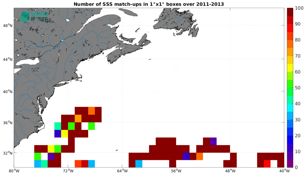
Figure 4: Number of SSS match-ups between Surface drifters SSS and the CCI SSS L4 Merged-OI v5.5 - 7-day running (ESA) SSS product for the Gulf Stream Pi-MEP region over 1^\circ \times 1^\circ boxes and for the full satellite product period.
