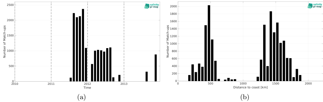
Figure 2: Number of match-ups between Surface drifters and CCI SSS L4 Merged-OI v5.5 - 7-day running (ESA) SSS as a function of time (a) and as function of the distance to coast (b) over the Gulf Stream Pi-MEP region and for the full satellite product period.
