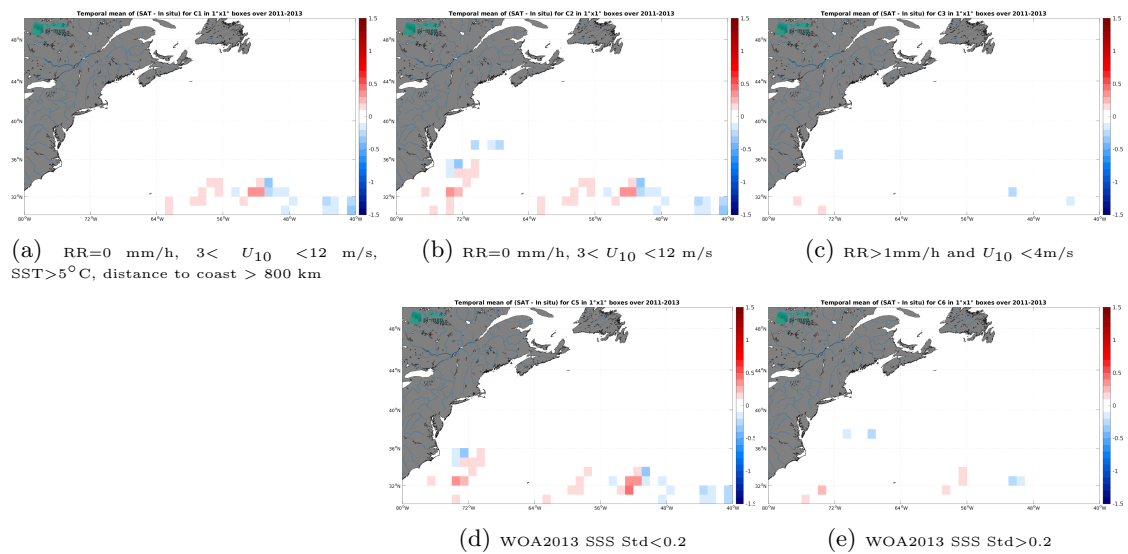
Figure 13: Temporal mean gridded over spatial boxes of size 1^\circ \times 1^\circ of \Delta SSS (CCI SSS L4 Merged-OI v5.5 - 7-day running (ESA) - Surface drifters) for 5 different subdatasets corresponding to:RR=0 mm/h, 3 < U_{10} < 12 m/s, SST >5^\circ C, distance to coast > 800 km (a), RR=0 mm/h, 3 < U_{10} < 12 m/s (b), RR >1 mm/h and U_{10} < 4 m/s (c), WOA2013 SSS Std <0.2 (d), WOA2013 SSS Std >0.2 (e).
