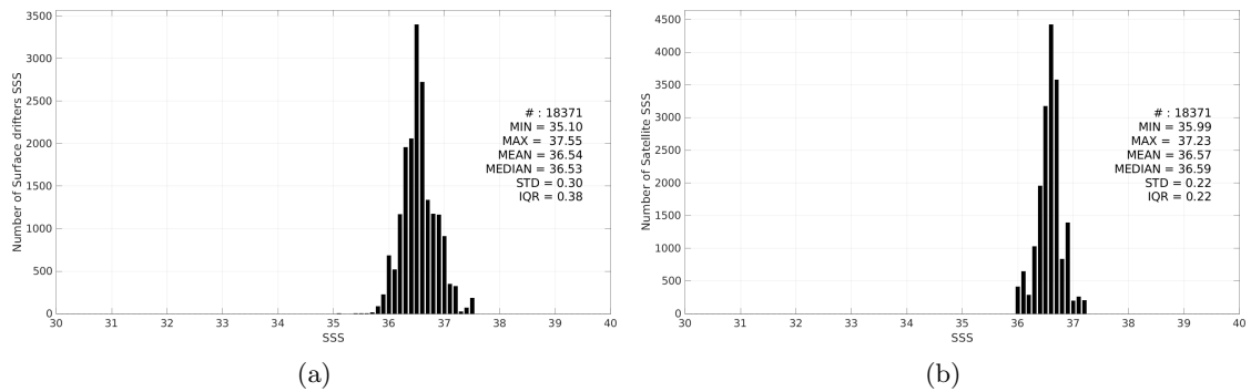
Figure 3: Histograms of SSS from Surface drifters (a) and CCI SSS L4 Merged-OI v5.5 - 7-day running (ESA) (b) considering all match-up pairs per bins of 0.1 over the Gulf Stream Pi-MEP region and for the full satellite product period.
