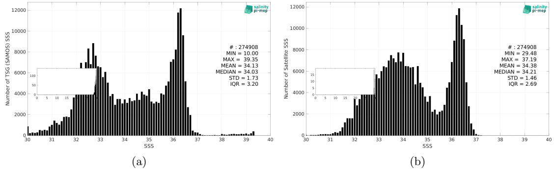
Figure 3: Histograms of SSS from TSG (SAMOS) (a) and CCI SSS L4 Merged-OI v4.41 - 7-day running (ESA) (b) considering all match-up pairs per bins of 0.1 over the Gulf Stream Pi-MEP region and for the full satellite product period.
