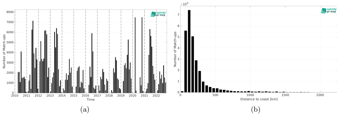
Figure 2: Number of match-ups between TSG (SAMOS) and CCI SSS L4 Merged-OI v4.41 - 7-day running (ESA) SSS as a function of time (a) and as function of the distance to coast (b) over the Gulf Stream Pi-MEP region and for the full satellite product period.
