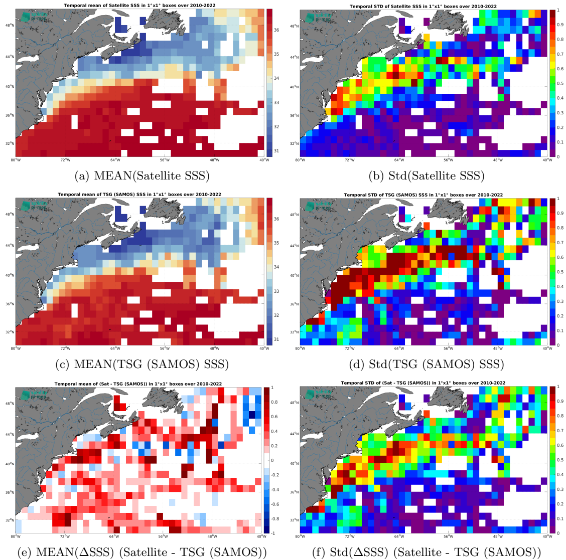
Figure 7: Temporal mean (left) and Std (right) of SSS from CCI SSS L4 Merged-OI v4.41 - 7-day running (ESA) (top), TSG (SAMOS) (middle), and of \Delta SSS (Satellite - TSG (SAMOS)). Only match-up pairs are used to generate these maps.
