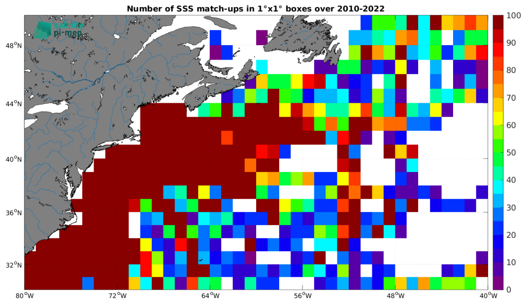
Figure 5: Number of SSS match-ups between TSG (SAMOS) SSS and the CCI SSS L4 Merged-OI v4.41 - 7-day running (ESA) SSS product for the Gulf Stream Pi-MEP region over 1^\circ \times 1^\circ boxes and for the full satellite product period.
