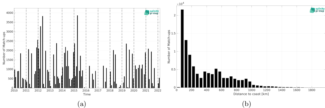
Figure 2: Number of match-ups between TSG (LEGOS-DM) and CCI SSS L4 Merged-OI v4.41 - 7-day running (ESA) SSS as a function of time (a) and as function of the distance to coast (b) over the Gulf Stream Pi-MEP region and for the full satellite product period.
