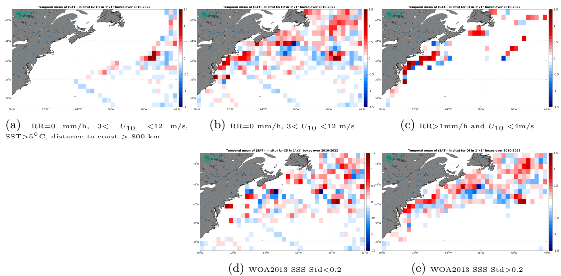
Figure 14: Temporal mean gridded over spatial boxes of size 1^\circ \times 1^\circ of \Delta SSS (CCI SSS L4 Merged-OI v4.41 - 7-day running (ESA) - TSG (LEGOS-DM)) for 5 different subdatasets corresponding to:RR=0 mm/h, 3 < U_{10} < 12 m/s, SST >5^\circ C, distance to coast > 800 km (a), RR=0 mm/h, 3 < U_{10} < 12 m/s (b), RR >1 mm/h and U_{10} < 4 m/s (c), WOA2013 SSS Std <0.2 (d), WOA2013 SSS Std >0.2 (e).
