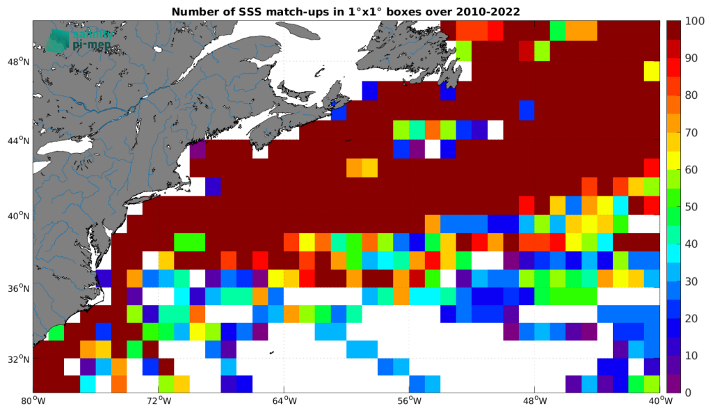
Figure 5: Number of SSS match-ups between TSG (LEGOS-DM) SSS and the CCI SSS L4 Merged-OI v4.41 - 7-day running (ESA) SSS product for the Gulf Stream Pi-MEP region over 1^\circ \times 1^\circ boxes and for the full satellite product period.
