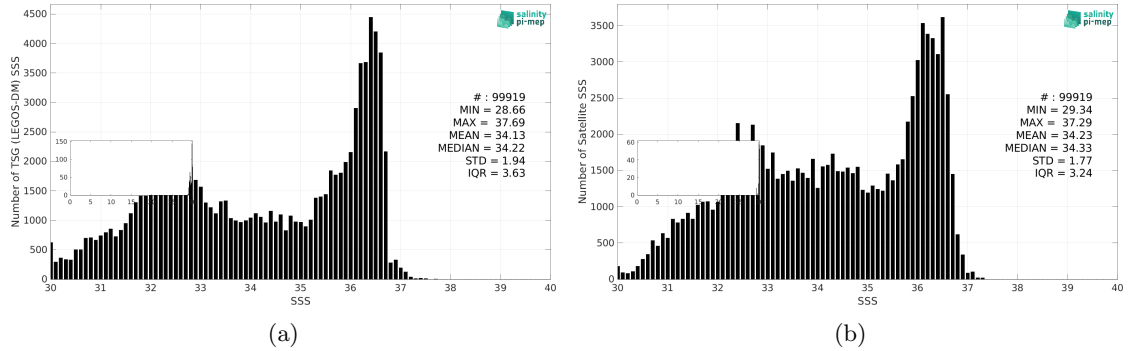
Figure 3: Histograms of SSS from TSG (LEGOS-DM) (a) and CCI SSS L4 Merged-OI v4.41 - 7-day running (ESA) (b) considering all match-up pairs per bins of 0.1 over the Gulf Stream Pi-MEP region and for the full satellite product period.
