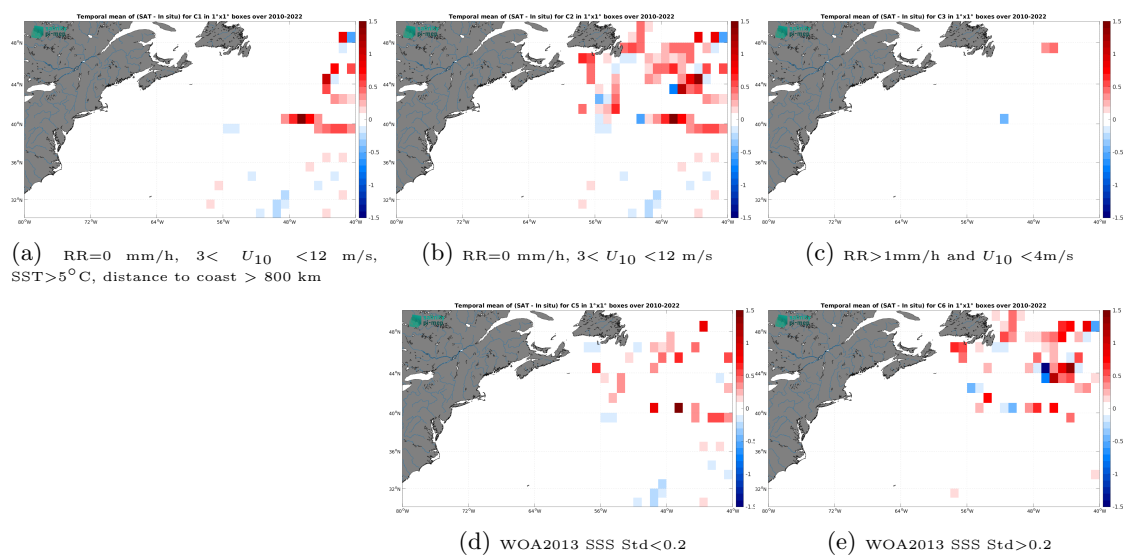
Figure 14: Temporal mean gridded over spatial boxes of size 1^\circ \times 1^\circ of \Delta\text{SSS} (CCI SSS L4 Merged-OI v4.41 - 7-day running (ESA) - TSG (GOSUD-Research-vessel)) for 5 different subdatasets corresponding to:RR=0 mm/h, 3 < U_{10} < 12 m/s, SST >5^\circ\text{C} , distance to coast > 800 km (a), RR=0 mm/h, 3 < U_{10} < 12 m/s (b), RR >1 mm/h and U_{10} < 4 m/s (c), WOA2013 SSS Std <0.2 (d), WOA2013 SSS Std >0.2 (e).
