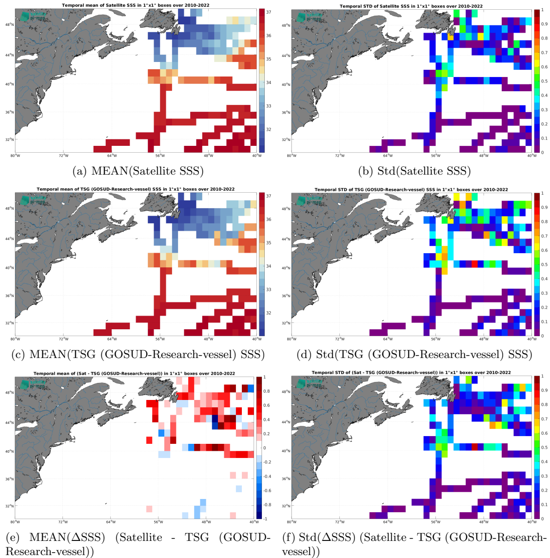
Figure 7: Temporal mean (left) and Std (right) of SSS from CCI SSS L4 Merged-OI v4.41 - 7-day running (ESA) (top), TSG (GOSUD-Research-vessel) (middle), and of \Delta SSS (Satellite - TSG (GOSUD-Research-vessel)). Only match-up pairs are used to generate these maps.
