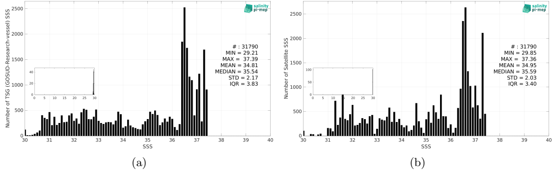
Figure 3: Histograms of SSS from TSG (GOSUD-Research-vessel) (a) and CCI SSS L4 Merged-OI v4.41 - 7-day running (ESA) (b) considering all match-up pairs per bins of 0.1 over the Gulf Stream Pi-MEP region and for the full satellite product period.
