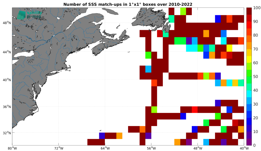
Figure 5: Number of SSS match-ups between TSG (GOSUD-Research-vessel) SSS and the CCI SSS L4 Merged-OI v4.41 - 7-day running (ESA) SSS product for the Gulf Stream Pi-MEP region over 1^\circ \times 1^\circ boxes and for the full satellite product period.
