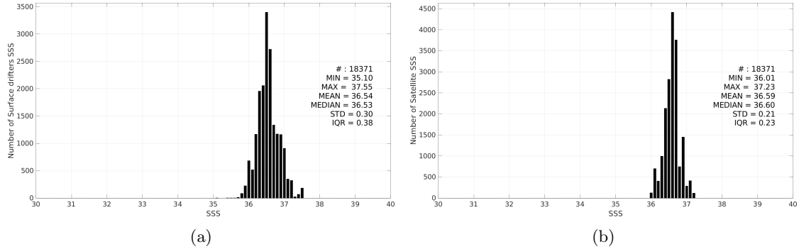
Figure 3: Histograms of SSS from Surface drifters (a) and CCI SSS L4 Merged-OI v4.41 - 7-day running (ESA) (b) considering all match-up pairs per bins of 0.1 over the Gulf Stream Pi-MEP region and for the full satellite product period.
