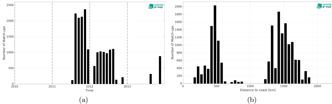
Figure 2: Number of match-ups between Surface drifters and CCI SSS L4 Merged-OI v4.41 - 7-day running (ESA) SSS as a function of time (a) and as function of the distance to coast (b) over the Gulf Stream Pi-MEP region and for the full satellite product period.
