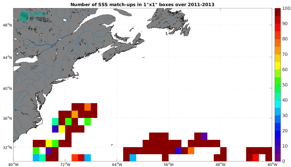
Figure 4: Number of SSS match-ups between Surface drifters SSS and the CCI SSS L4 Merged-OI v4.41 - 7-day running (ESA) SSS product for the Gulf Stream Pi-MEP region over 1^\circ \times 1^\circ boxes and for the full satellite product period.
