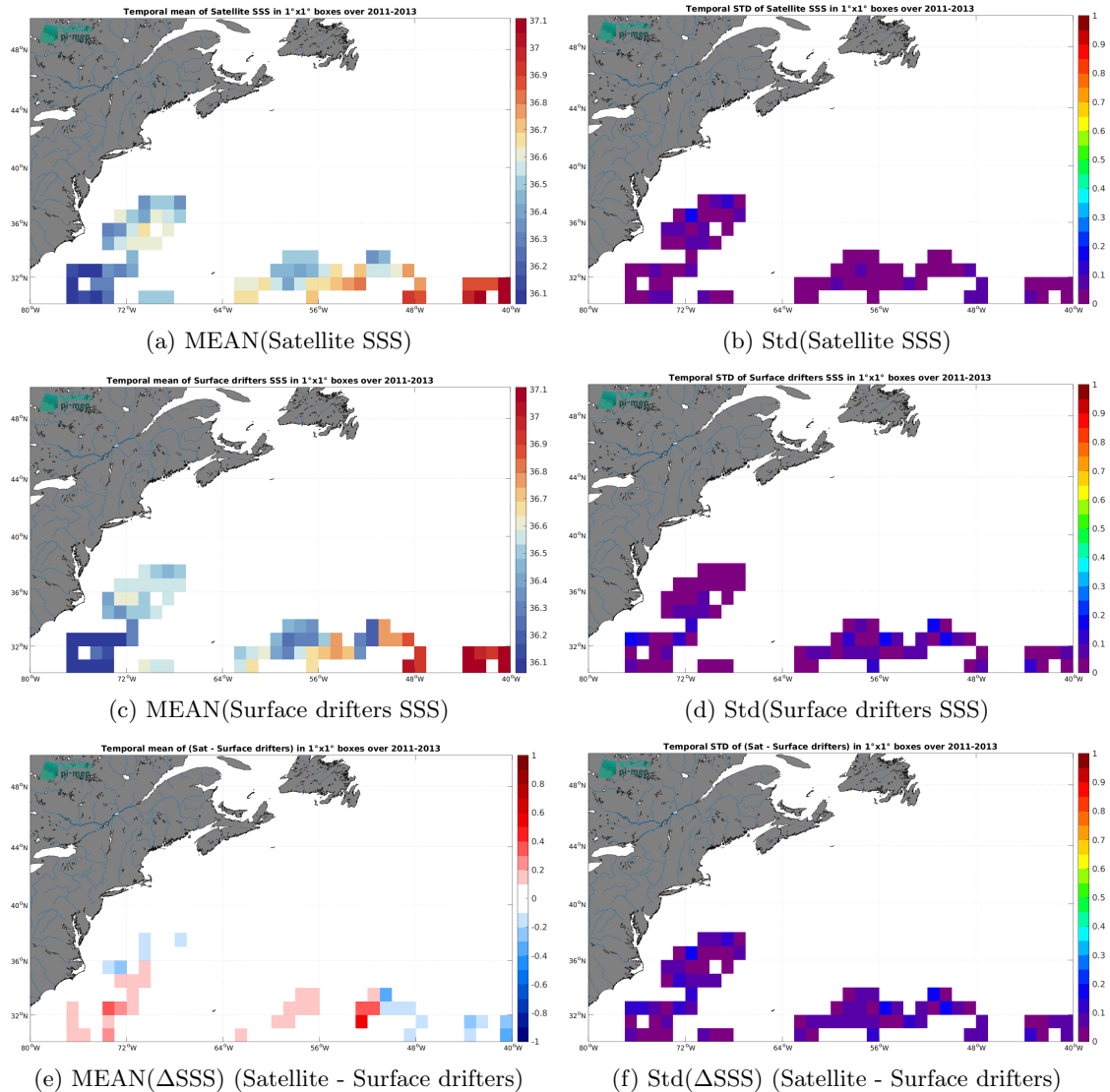
Figure 6: Temporal mean (left) and Std (right) of SSS from CCI SSS L4 Merged-OI v4.41 - 7-day running (ESA) (top), Surface drifters (middle), and of \Delta SSS (Satellite - Surface drifters). Only match-up pairs are used to generate these maps.
