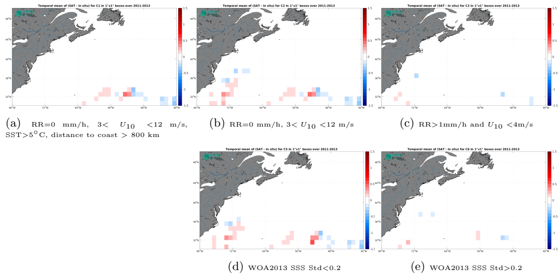
Figure 13: Temporal mean gridded over spatial boxes of size 1^\circ \times 1^\circ of \Delta\text{SSS} (CCI SSS L4 Merged-OI v4.41 - 7-day running (ESA) - Surface drifters) for 5 different subdatasets corresponding to:RR=0 mm/h, 3 < U_{10} < 12 m/s, SST >5^\circ\text{C} , distance to coast > 800 km (a), RR=0 mm/h, 3 < U_{10} < 12 m/s (b), RR >1 mm/h and U_{10} < 4 m/s (c), WOA2013 SSS Std <0.2 (d), WOA2013 SSS Std >0.2 (e).
