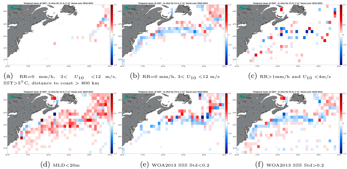
Figure 14: Temporal mean gridded over spatial boxes of size 1^\circ \times 1^\circ of \Delta SSS (CCI SSS L4 Merged-OI v4.41 - 7-day running (ESA) - Argo) for 6 different subdatasets corresponding to:RR=0 mm/h, 3 < U_{10} < 12 m/s, SST > 5^\circ\text{C} , distance to coast > 800 km (a), RR=0 mm/h, 3 < U_{10} < 12 m/s (b), RR > 1 mm/h and U_{10} < 4 m/s (c),MLD < 20 m (d),WOA2013 SSS Std < 0.2 (e),WOA2013 SSS Std > 0.2 (f).
