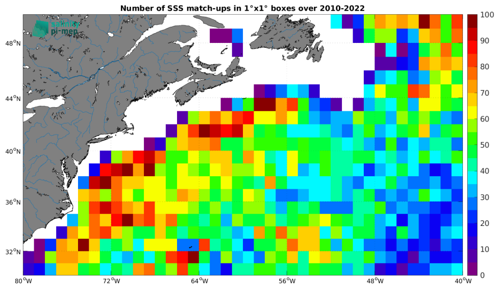
Figure 5: Number of SSS match-ups between Argo SSS and the CCI SSS L4 Merged-OI v4.41 - 7-day running (ESA) SSS product for the Gulf Stream Pi-MEP region over 1^\circ \times 1^\circ boxes and for the full satellite product period.
