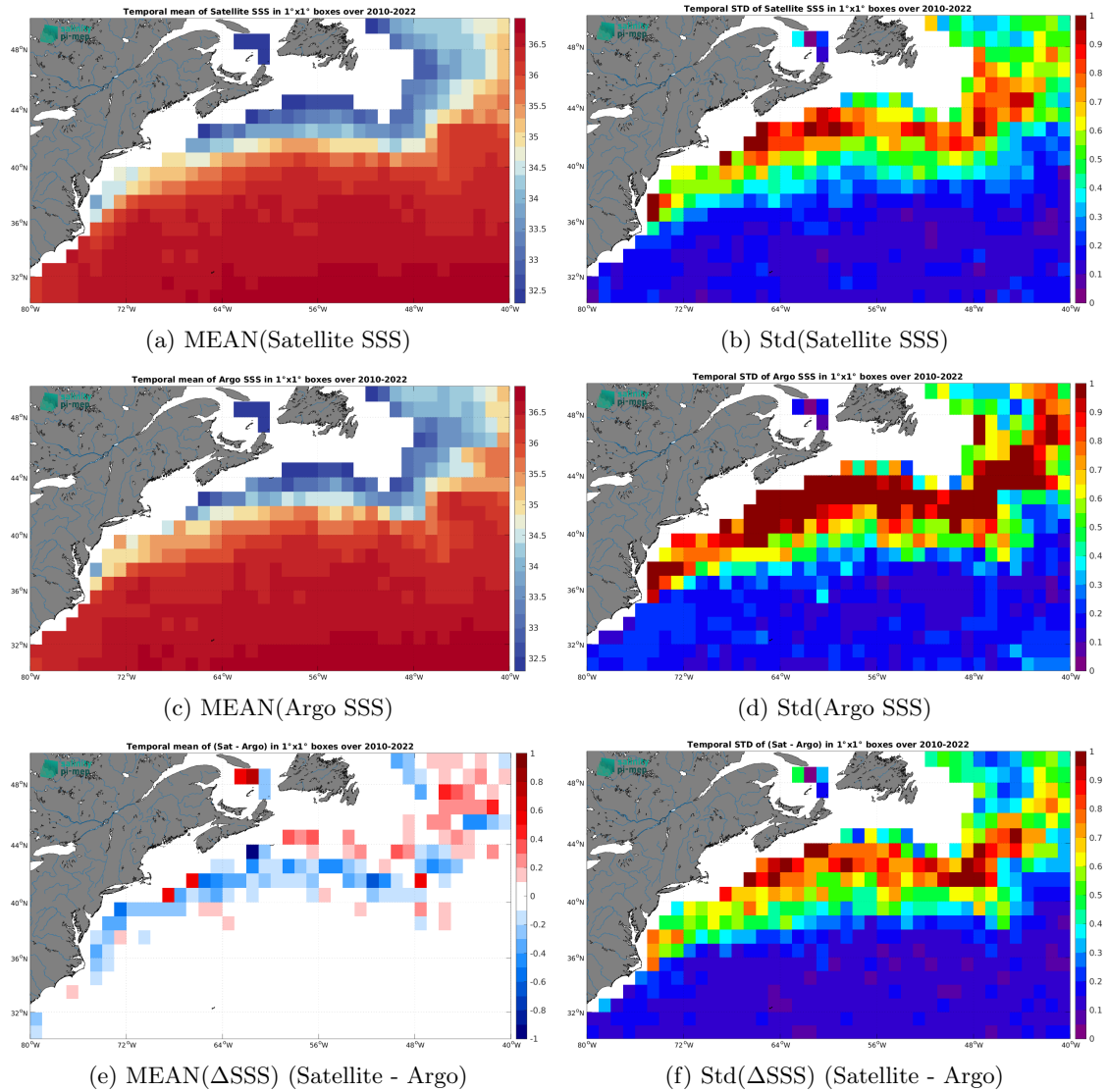
Figure 7: Temporal mean (left) and Std (right) of SSS from CCI SSS L4 Merged-OI v4.41 - 7-day running (ESA) (top), Argo (middle), and of \Delta SSS (Satellite - Argo). Only match-up pairs are used to generate these maps.
