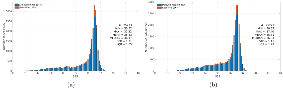
Figure 3: Histograms of SSS from Argo (a) and CCI SSS L4 Merged-OI v4.41 - 7-day running (ESA) (b) considering all match-up pairs per bins of 0.1 over the Gulf Stream Pi-MEP region and for the full satellite product period.
