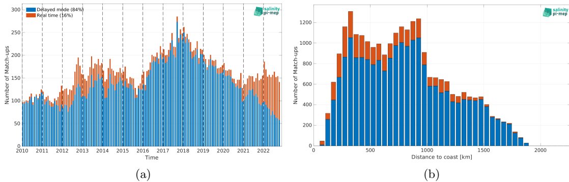
Figure 2: Number of match-ups between Argo and CCI SSS L4 Merged-OI v4.41 - 7-day running (ESA) SSS as a function of time (a) and as function of the distance to coast (b) over the Gulf Stream Pi-MEP region and for the full satellite product period.
