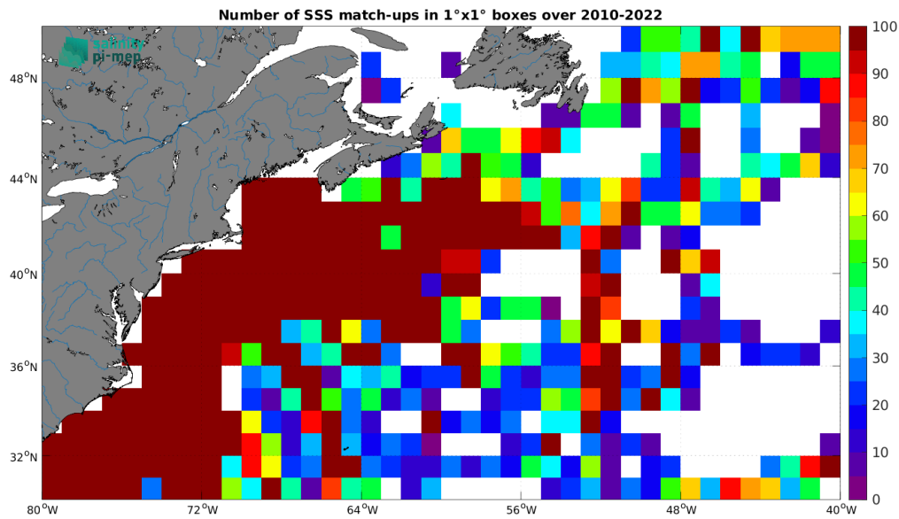
Figure 5: Number of SSS match-ups between TSG (SAMOS) SSS and the CCI SSS L4 Merged-OI v4.41 - 30-day running (ESA) SSS product for the Gulf Stream Pi-MEP region over 1^\circ \times 1^\circ boxes and for the full satellite product period.
