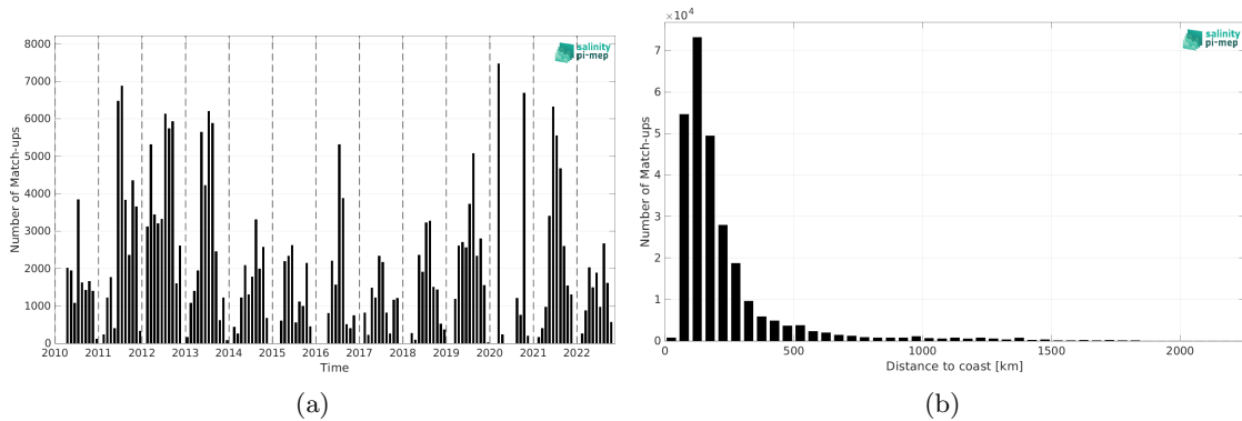
Figure 2: Number of match-ups between TSG (SAMOS) and CCI SSS L4 Merged-OI v4.41 - 30-day running (ESA) SSS as a function of time (a) and as function of the distance to coast (b) over the Gulf Stream Pi-MEP region and for the full satellite product period.
