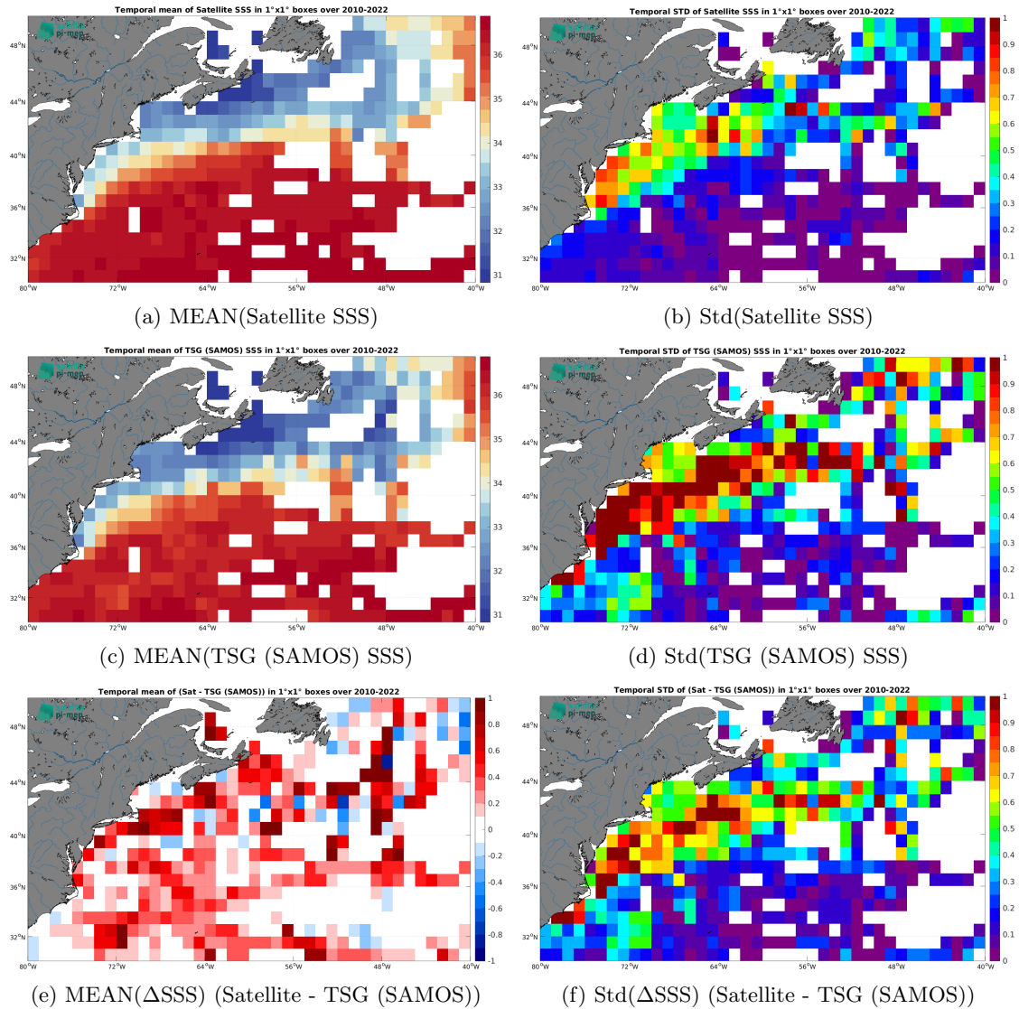
Figure 7: Temporal mean (left) and Std (right) of SSS from CCI SSS L4 Merged-OI v4.41 - 30-day running (ESA) (top), TSG (SAMOS) (middle), and of \Delta SSS (Satellite - TSG (SAMOS)). Only match-up pairs are used to generate these maps.
