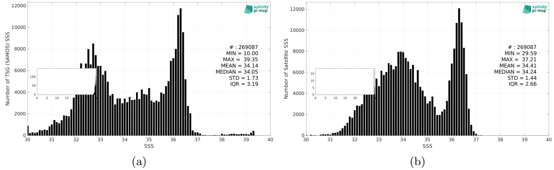
Figure 3: Histograms of SSS from TSG (SAMOS) (a) and CCI SSS L4 Merged-OI v4.41 - 30-day running (ESA) (b) considering all match-up pairs per bins of 0.1 over the Gulf Stream Pi-MEP region and for the full satellite product period.
