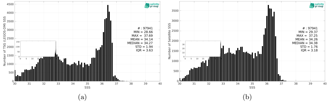
Figure 3: Histograms of SSS from TSG (LEGOS-DM) (a) and CCI SSS L4 Merged-OI v4.41 - 30-day running (ESA) (b) considering all match-up pairs per bins of 0.1 over the Gulf Stream Pi-MEP region and for the full satellite product period.
