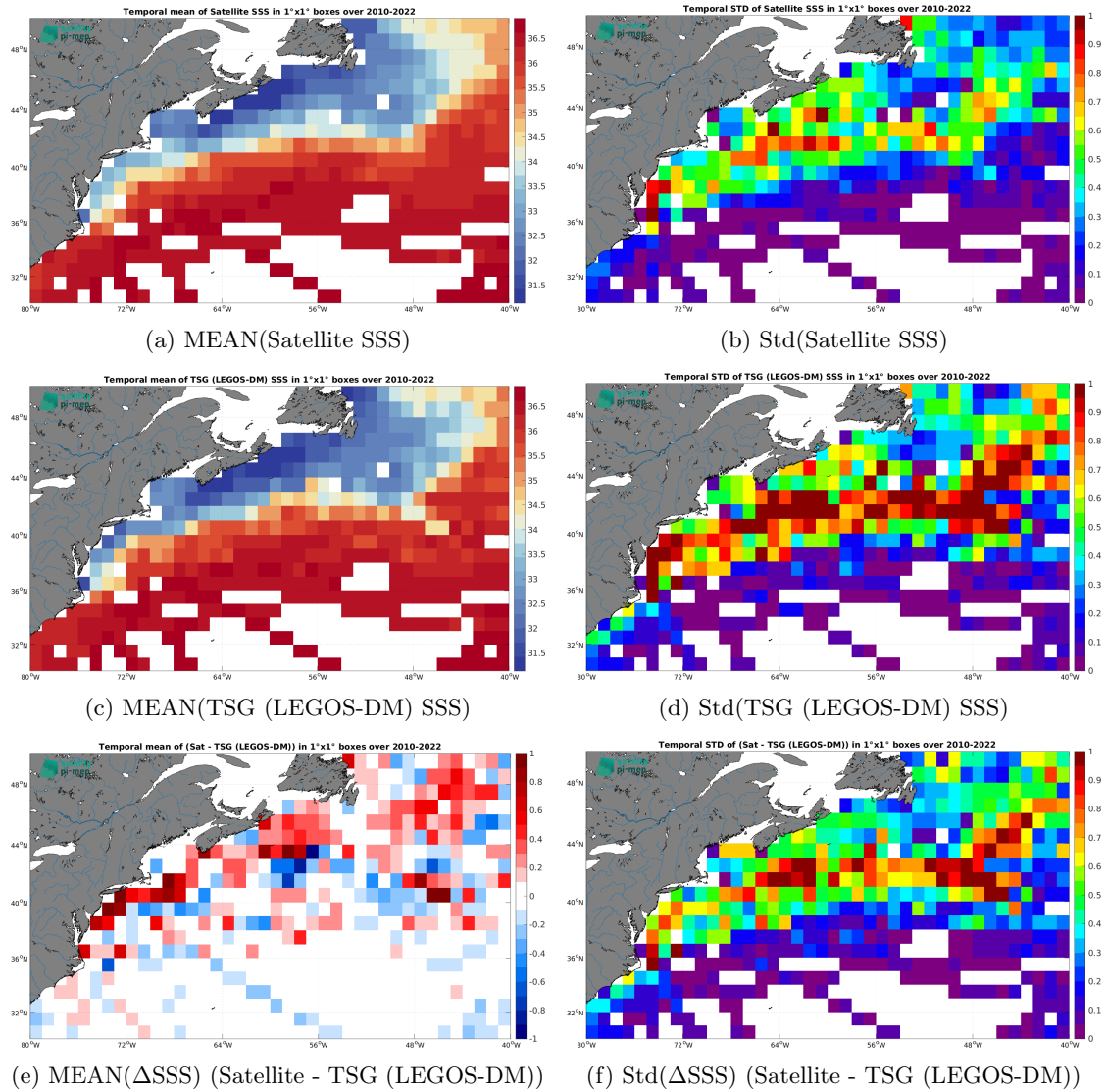
Figure 7: Temporal mean (left) and Std (right) of SSS from CCI SSS L4 Merged-OI v4.41 - 30-day running (ESA) (top), TSG (LEGOS-DM) (middle), and of \Delta SSS (Satellite - TSG (LEGOS-DM)). Only match-up pairs are used to generate these maps.
