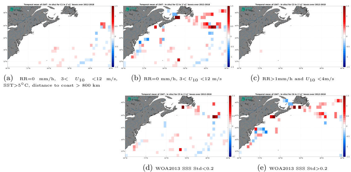
Figure 14: Temporal mean gridded over spatial boxes of size 1^\circ \times 1^\circ of \Delta SSS (CCI SSS L4 Merged-OI v4.41 - 30-day running (ESA) - TSG (GOSUD-Sailing-ship)) for 5 different subdatasets corresponding to:RR=0 mm/h, 3 < U_{10} < 12 m/s, SST >5^\circ C, distance to coast > 800 km (a), RR=0 mm/h, 3 < U_{10} < 12 m/s (b), RR >1 mm/h and U_{10} < 4 m/s (c), WOA2013 SSS Std <0.2 (d), WOA2013 SSS Std >0.2 (e).
