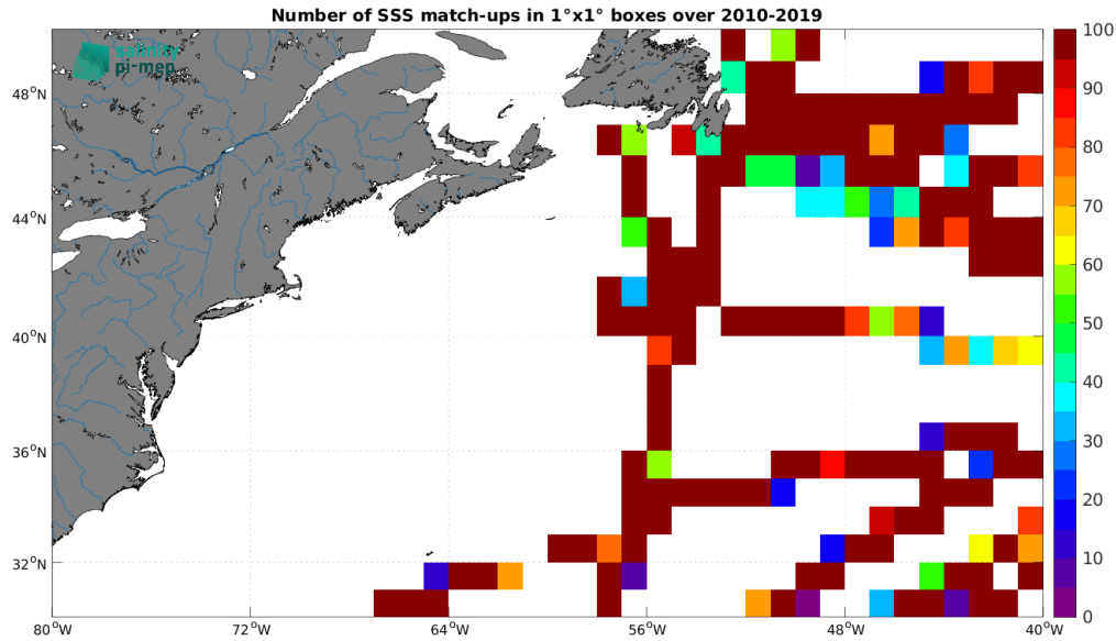
Figure 5: Number of SSS match-ups between TSG (GOSUD-Research-vessel) SSS and the CCI SSS L4 Merged-OI v4.41 - 30-day running (ESA) SSS product for the Gulf Stream Pi-MEP region over 1^\circ \times 1^\circ boxes and for the full satellite product period.
