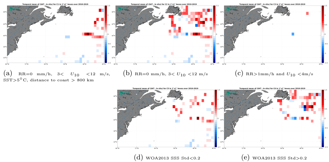
Figure 14: Temporal mean gridded over spatial boxes of size 1^\circ \times 1^\circ of \Delta SSS (CCI SSS L4 Merged-OI v4.41 - 30-day running (ESA) - TSG (GOSUD-Research-vessel)) for 5 different subdatasets corresponding to:RR=0 mm/h, 3 < U_{10} < 12 m/s, SST >5^\circ C, distance to coast > 800 km (a), RR=0 mm/h, 3 < U_{10} < 12 m/s (b), RR >1 mm/h and U_{10} < 4 m/s (c), WOA2013 SSS Std <0.2 (d), WOA2013 SSS Std >0.2 (e).
