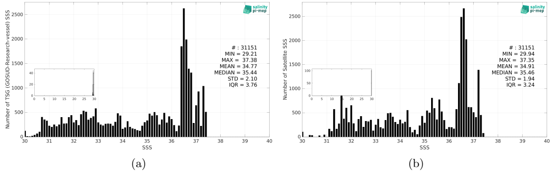
Figure 3: Histograms of SSS from TSG (GOSUD-Research-vessel) (a) and CCI SSS L4 Merged-OI v4.41 - 30-day running (ESA) (b) considering all match-up pairs per bins of 0.1 over the Gulf Stream Pi-MEP region and for the full satellite product period.
