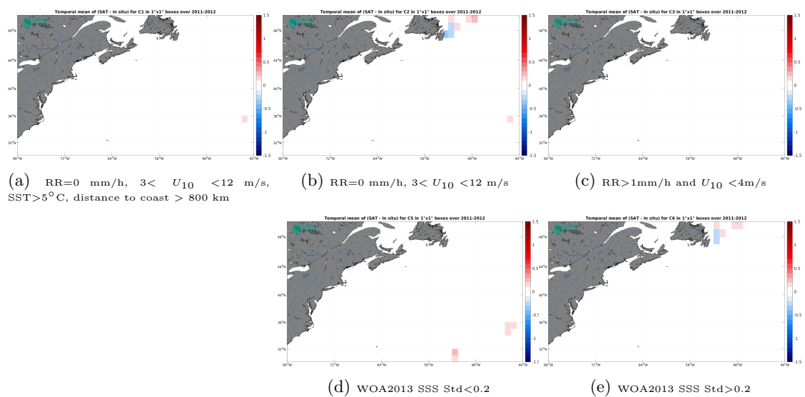
Figure 14: Temporal mean gridded over spatial boxes of size 1^\circ \times 1^\circ of \Delta\text{SSS} (CCI SSS L4 Merged-OI v4.41 - 30-day running (ESA) - TSG (CSIC-UTM)) for 5 different subdatasets corresponding to:RR=0 mm/h, 3 < U_{10} < 12 m/s, SST >5^\circ\text{C} , distance to coast > 800 km (a), RR=0 mm/h, 3 < U_{10} < 12 m/s (b), RR >1 mm/h and U_{10} < 4 m/s (c), WOA2013 SSS Std <0.2 (d), WOA2013 SSS Std >0.2 (e).
