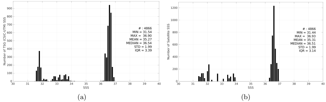
Figure 3: Histograms of SSS from TSG (CSIC-UTM) (a) and CCI SSS L4 Merged-OI v4.41 - 30-day running (ESA) (b) considering all match-up pairs per bins of 0.1 over the Gulf Stream Pi-MEP region and for the full satellite product period.
