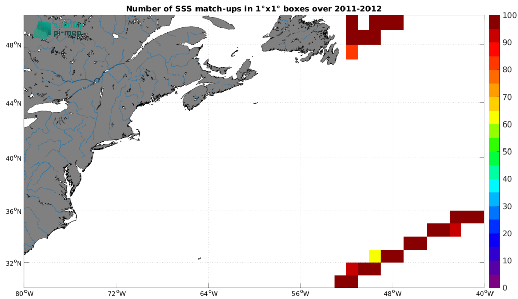
Figure 5: Number of SSS match-ups between TSG (CSIC-UTM) SSS and the CCI SSS L4 Merged-OI v4.41 - 30-day running (ESA) SSS product for the Gulf Stream Pi-MEP region over 1^\circ \times 1^\circ boxes and for the full satellite product period.
