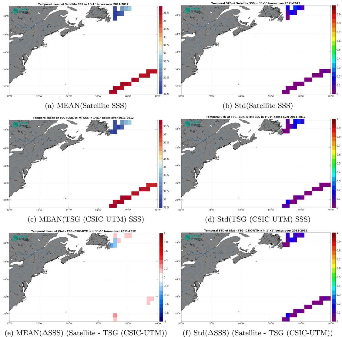
Figure 7: Temporal mean (left) and Std (right) of SSS from CCI SSS L4 Merged-OI v4.41 - 30-day running (ESA) (top), TSG (CSIC-UTM) (middle), and of \Delta SSS (Satellite - TSG (CSIC-UTM)). Only match-up pairs are used to generate these maps.
