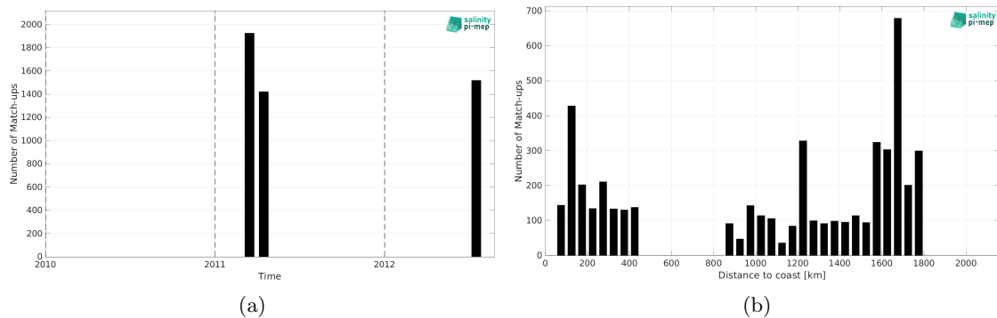
Figure 2: Number of match-ups between TSG (CSIC-UTM) and CCI SSS L4 Merged-OI v4.41 - 30-day running (ESA) SSS as a function of time (a) and as function of the distance to coast (b) over the Gulf Stream Pi-MEP region and for the full satellite product period.
