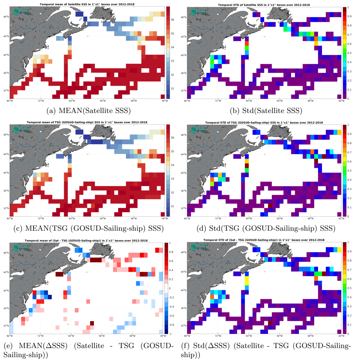
Figure 6: Temporal mean (left) and Std (right) of SSS from CCI SSS L4 Merged-OI v4.4 - 7-day running (ESA) (top), TSG (GOSUD-Sailing-ship) (middle), and of \Delta SSS (Satellite - TSG (GOSUD-Sailing-ship)). Only match-up pairs are used to generate these maps.
