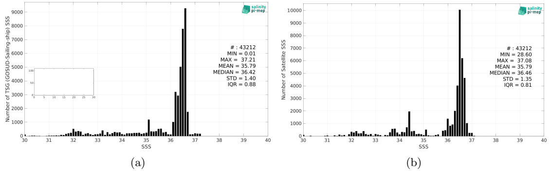
Figure 2: Histograms of SSS from TSG (GOSUD-Sailing-ship) (a) and CCI SSS L4 Merged-OI v4.4 - 7-day running (ESA) (b) considering all match-up pairs per bins of 0.1 over the Gulf Stream Pi-MEP region and for the full satellite product period.
