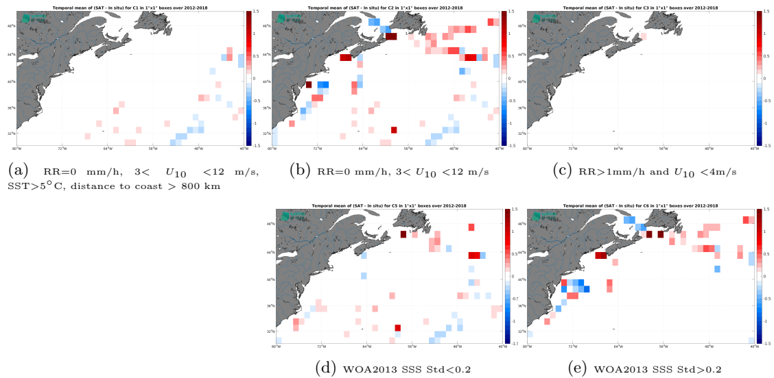
Figure 12: Temporal mean gridded over spatial boxes of size 1^{\circ}\times 1^{\circ} of \Delta SSS (CCI SSS L4 Merged-OI v4.4 - 7-day running (ESA) - TSG (GOSUD-Sailing-ship)) for 5 different subdatasets corresponding to:RR=0 mm/h, 3 < U_{10} < 12 m/s, SST > 5^{\circ}\text{C} , distance to coast > 800 km (a), RR=0 mm/h, 3 < U_{10} < 12 m/s (b), RR > 1 mm/h and U_{10} < 4 m/s (c), WOA2013 SSS Std < 0.2 (d), WOA2013 SSS Std > 0.2 (e).
