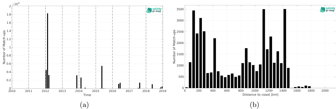
Figure 1: Number of match-ups between TSG (GOSUD-Sailing-ship) and CCI SSS L4 Merged-OI v4.4 - 7-day running (ESA) SSS as a function of time (a) and as function of the distance to coast (b) over the Gulf Stream Pi-MEP region and for the full satellite product period.
