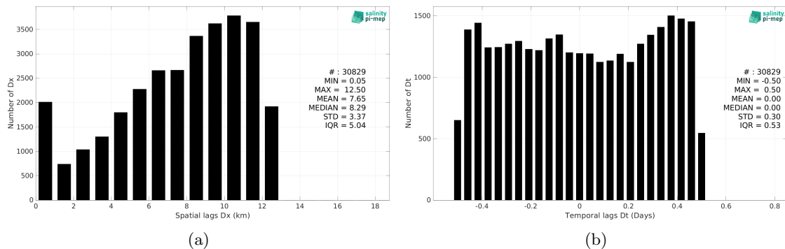
Figure 5: Histograms of the spatial (a) and temporal (b) lags between the location/time of the TSG (GOSUD-Research-vessel) measurement and the date of the corresponding CCI SSS L4 Merged-OI v4.4 - 7-day running (ESA) SSS pixel.
