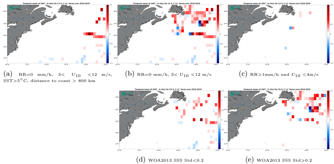
Figure 12: Temporal mean gridded over spatial boxes of size 1^\circ \times 1^\circ of \Delta SSS (CCI SSS L4 Merged-OI v4.4 - 7-day running (ESA) - TSG (GOSUD-Research-vessel)) for 5 different subdatasets corresponding to:RR=0 mm/h, 3 < U_{10} < 12 m/s, SST > 5^\circ\text{C} , distance to coast > 800 km (a), RR=0 mm/h, 3 < U_{10} < 12 m/s (b), RR > 1 mm/h and U_{10} < 4 m/s (c), WOA2013 SSS Std < 0.2 (d), WOA2013 SSS Std > 0.2 (e).
