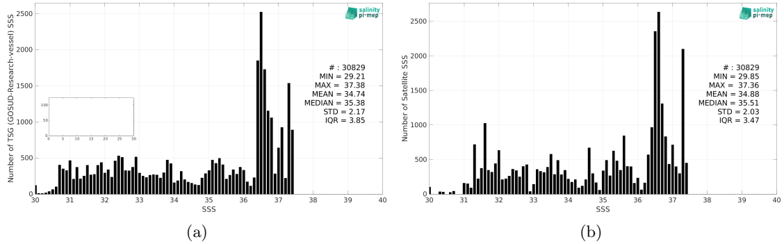
Figure 2: Histograms of SSS from TSG (GOSUD-Research-vessel) (a) and CCI SSS L4 Merged-OI v4.4 - 7-day running (ESA) (b) considering all match-up pairs per bins of 0.1 over the Gulf Stream Pi-MEP region and for the full satellite product period.
