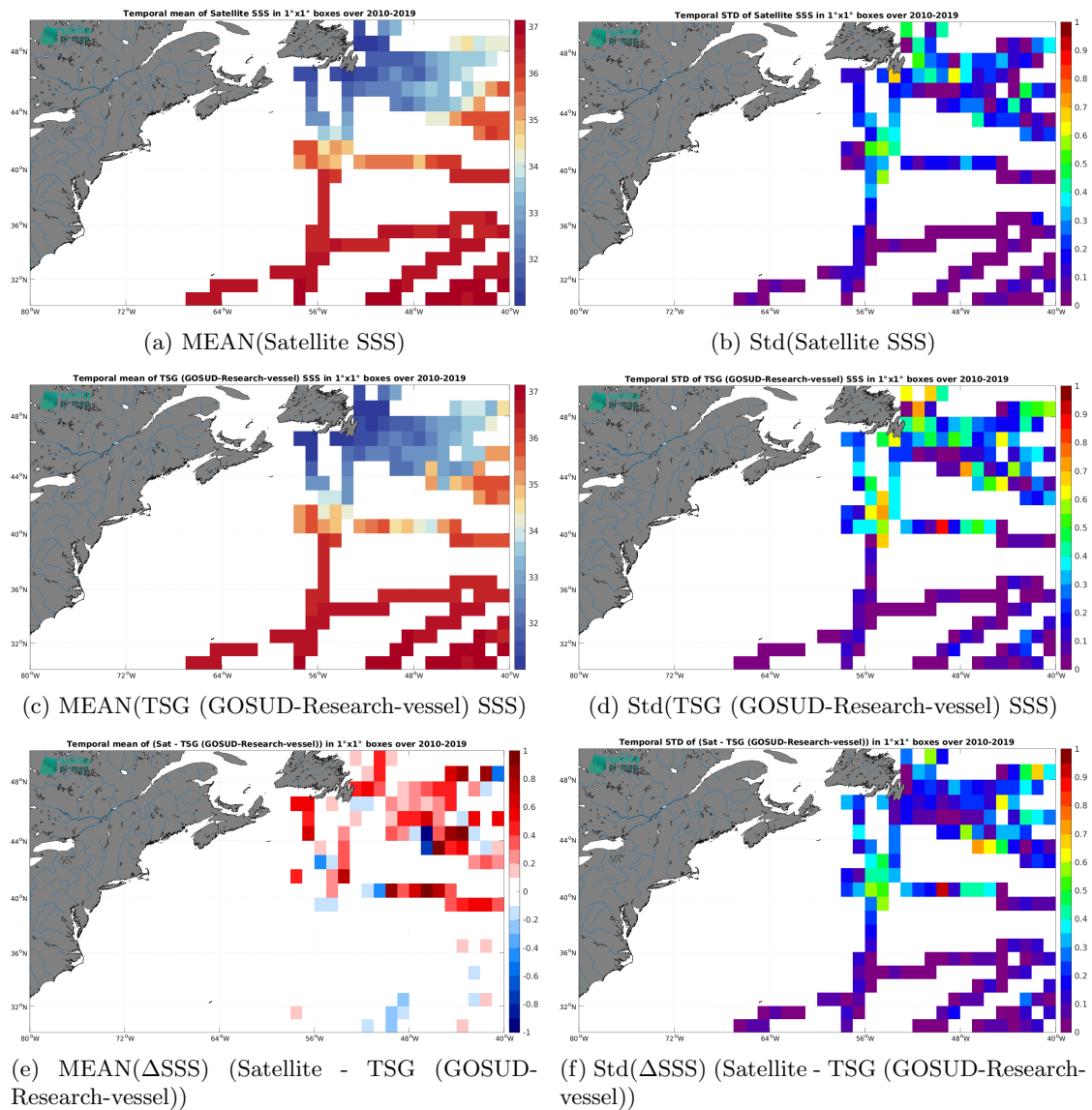
Figure 6: Temporal mean (left) and Std (right) of SSS from CCI SSS L4 Merged-OI v4.4 - 7-day running (ESA) (top), TSG (GOSUD-Research-vessel) (middle), and of \Delta SSS (Satellite - TSG (GOSUD-Research-vessel)). Only match-up pairs are used to generate these maps.
