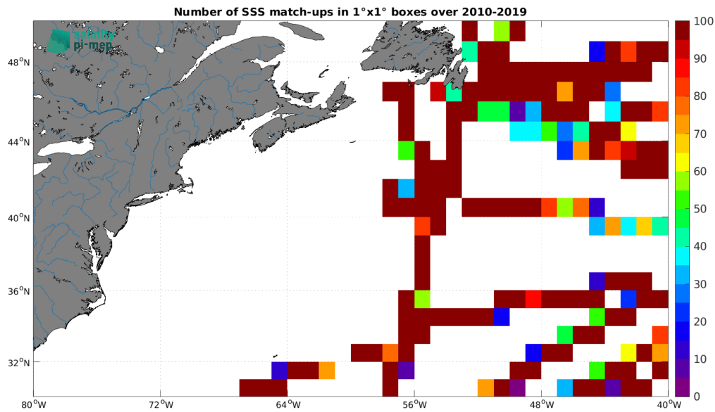
Figure 4: Number of SSS match-ups between TSG (GOSUD-Research-vessel) SSS and the CCI SSS L4 Merged-OI v4.4 - 7-day running (ESA) SSS product for the Gulf Stream Pi-MEP region over 1^\circ \times 1^\circ boxes and for the full satellite product period.
