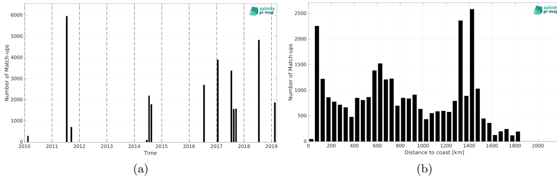
Figure 1: Number of match-ups between TSG (GOSUD-Research-vessel) and CCI SSS L4 Merged-OI v4.4 - 7-day running (ESA) SSS as a function of time (a) and as function of the distance to coast (b) over the Gulf Stream Pi-MEP region and for the full satellite product period.
