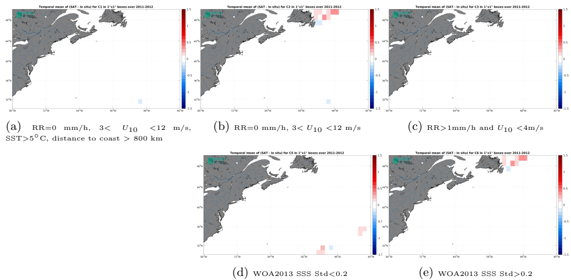
Figure 12: Temporal mean gridded over spatial boxes of size 1^\circ \times 1^\circ of \Delta SSS (CCI SSS L4 Merged-OI v4.4 - 7-day running (ESA) - TSG (CSIC-UTM)) for 5 different subdatasets corresponding to:RR=0 mm/h, 3 < U_{10} < 12 m/s, SST >5^\circ C, distance to coast > 800 km (a), RR=0 mm/h, 3 < U_{10} < 12 m/s (b), RR >1 mm/h and U_{10} < 4 m/s (c), WOA2013 SSS Std <0.2 (d), WOA2013 SSS Std >0.2 (e).
