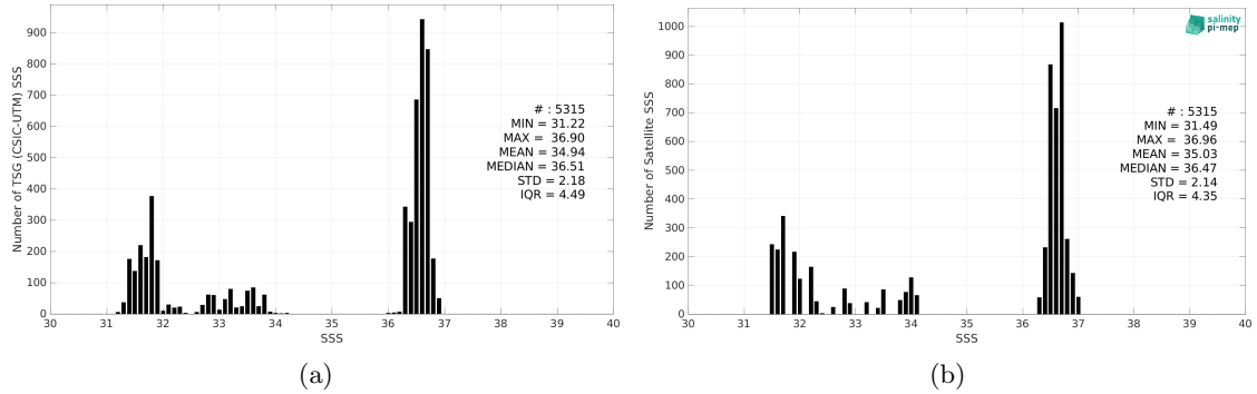
Figure 2: Histograms of SSS from TSG (CSIC-UTM) (a) and CCI SSS L4 Merged-OI v4.4 - 7-day running (ESA) (b) considering all match-up pairs per bins of 0.1 over the Gulf Stream Pi-MEP region and for the full satellite product period.
