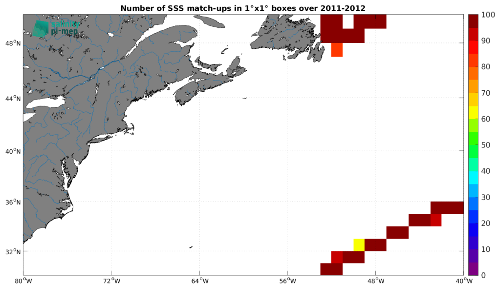
Figure 4: Number of SSS match-ups between TSG (CSIC-UTM) SSS and the CCI SSS L4 Merged-OI v4.4 - 7-day running (ESA) SSS product for the Gulf Stream Pi-MEP region over 1^\circ \times 1^\circ boxes and for the full satellite product period.
