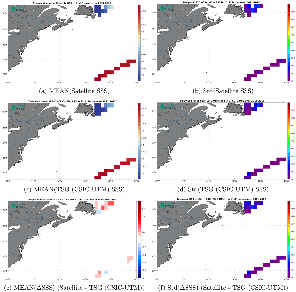
Figure 6: Temporal mean (left) and Std (right) of SSS from CCI SSS L4 Merged-OI v4.4 - 7-day running (ESA) (top), TSG (CSIC-UTM) (middle), and of \Delta SSS (Satellite - TSG (CSIC-UTM)). Only match-up pairs are used to generate these maps.
