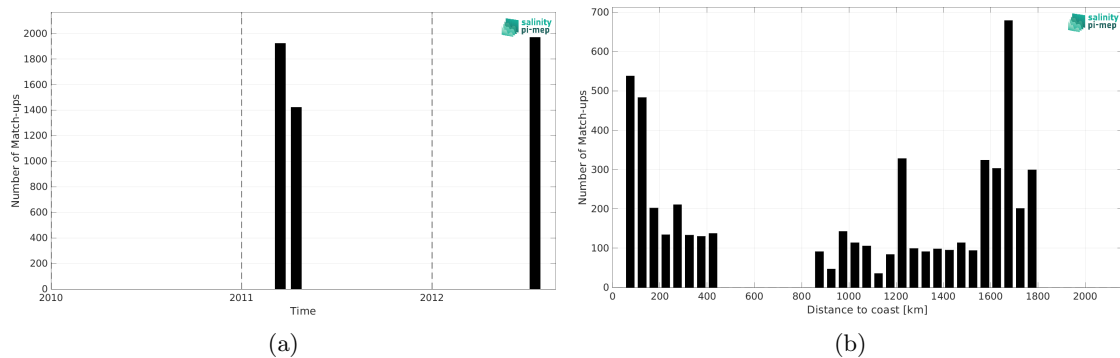
Figure 1: Number of match-ups between TSG (CSIC-UTM) and CCI SSS L4 Merged-OI v4.4 - 7-day running (ESA) SSS as a function of time (a) and as function of the distance to coast (b) over the Gulf Stream Pi-MEP region and for the full satellite product period.
