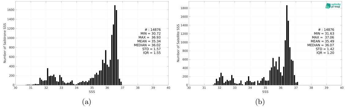
Figure 2: Histograms of SSS from Saildrone (a) and CCI SSS L4 Merged-OI v4.4 - 7-day running (ESA) (b) considering all match-up pairs per bins of 0.1 over the Gulf Stream Pi-MEP region and for the full satellite product period.
