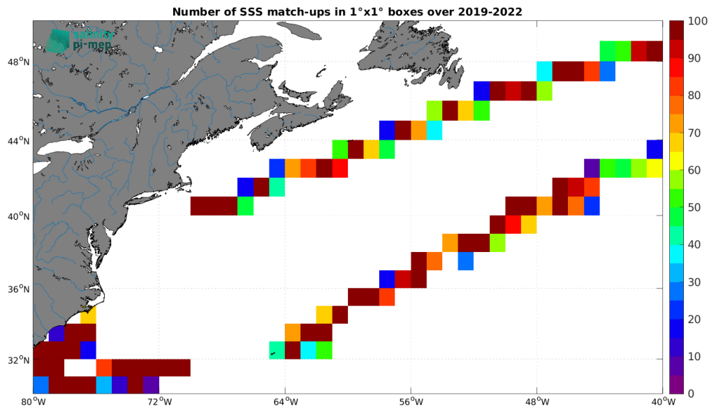
Figure 4: Number of SSS match-ups between Saildrone SSS and the CCI SSS L4 Merged-OI v4.4 - 7-day running (ESA) SSS product for the Gulf Stream Pi-MEP region over 1^\circ \times 1^\circ boxes and for the full satellite product period.
