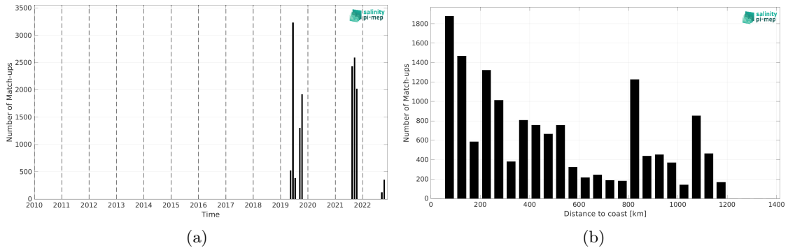
Figure 1: Number of match-ups between Saildrone and CCI SSS L4 Merged-OI v4.4 - 7-day running (ESA) SSS as a function of time (a) and as function of the distance to coast (b) over the Gulf Stream Pi-MEP region and for the full satellite product period.
