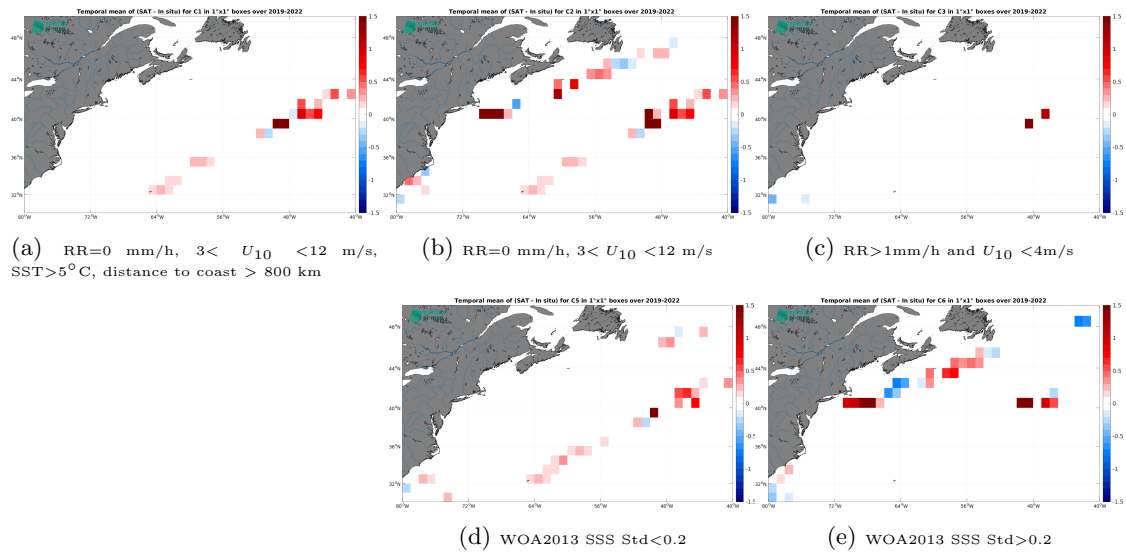
Figure 12: Temporal mean gridded over spatial boxes of size 1^\circ \times 1^\circ of \Delta SSS (CCI SSS L4 Merged-OI v4.4 - 7-day running (ESA) - Saildrone) for 5 different subdatasets corresponding to:RR=0 mm/h, 3 < U_{10} < 12 m/s, SST >5^\circ C, distance to coast > 800 km (a), RR=0 mm/h, 3 < U_{10} < 12 m/s (b), RR >1 mm/h and U_{10} < 4 m/s (c), WOA2013 SSS Std <0.2 (d), WOA2013 SSS Std >0.2 (e).
