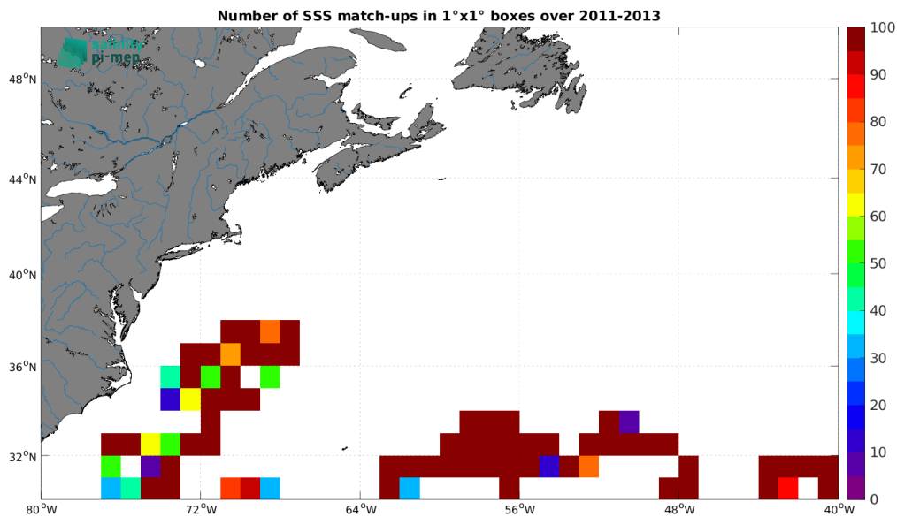
Figure 3: Number of SSS match-ups between Surface drifters SSS and the CCI SSS L4 Merged-OI v4.4 - 7-day running (ESA) SSS product for the Gulf Stream Pi-MEP region over 1^\circ \times 1^\circ boxes and for the full satellite product period.
