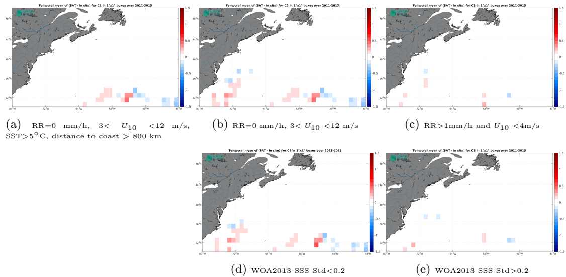
Figure 11: Temporal mean gridded over spatial boxes of size 1^{\circ}\times 1^{\circ} of \Delta\text{SSS} (CCI SSS L4 Merged-OI v4.4 - 7-day running (ESA) - Surface drifters) for 5 different subdatasets corresponding to:RR=0 mm/h, 3 < U_{10} < 12 m/s, SST >5^{\circ}\text{C} , distance to coast > 800 km (a), RR=0 mm/h, 3 < U_{10} < 12 m/s (b), RR >1 mm/h and U_{10} < 4 m/s (c), WOA2013 SSS Std <0.2 (d), WOA2013 SSS Std >0.2 (e).
