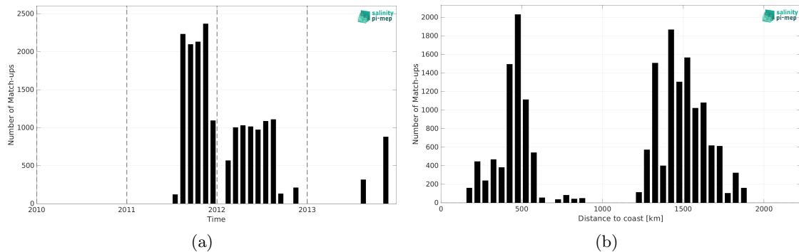
Figure 1: Number of match-ups between Surface drifters and CCI SSS L4 Merged-OI v4.4 - 7-day running (ESA) SSS as a function of time (a) and as function of the distance to coast (b) over the Gulf Stream Pi-MEP region and for the full satellite product period.
