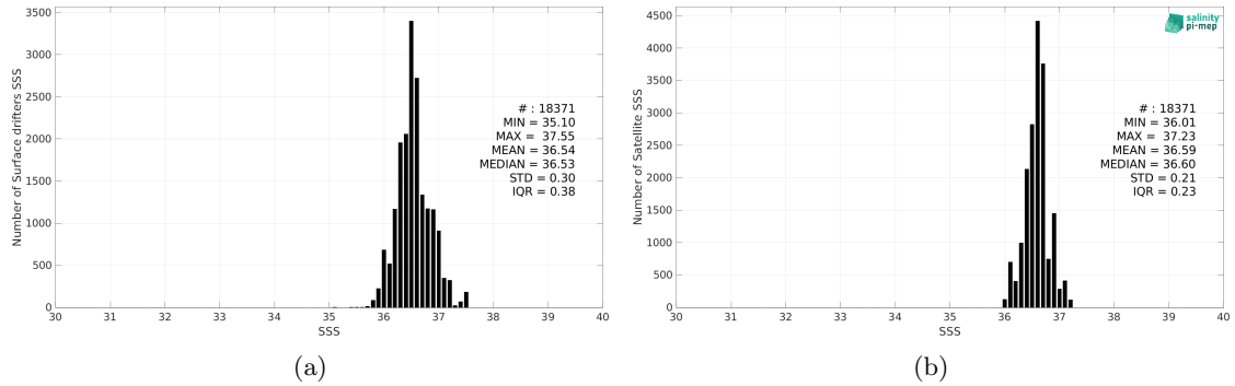
Figure 2: Histograms of SSS from Surface drifters (a) and CCI SSS L4 Merged-OI v4.4 - 7-day running (ESA) (b) considering all match-up pairs per bins of 0.1 over the Gulf Stream Pi-MEP region and for the full satellite product period.
