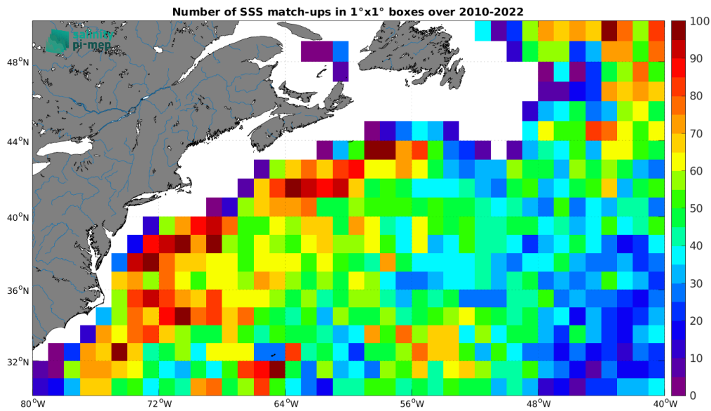
Figure 4: Number of SSS match-ups between Argo SSS and the CCI SSS L4 Merged-OI v4.4 - 7-day running (ESA) SSS product for the Gulf Stream Pi-MEP region over 1^\circ \times 1^\circ boxes and for the full satellite product period.
