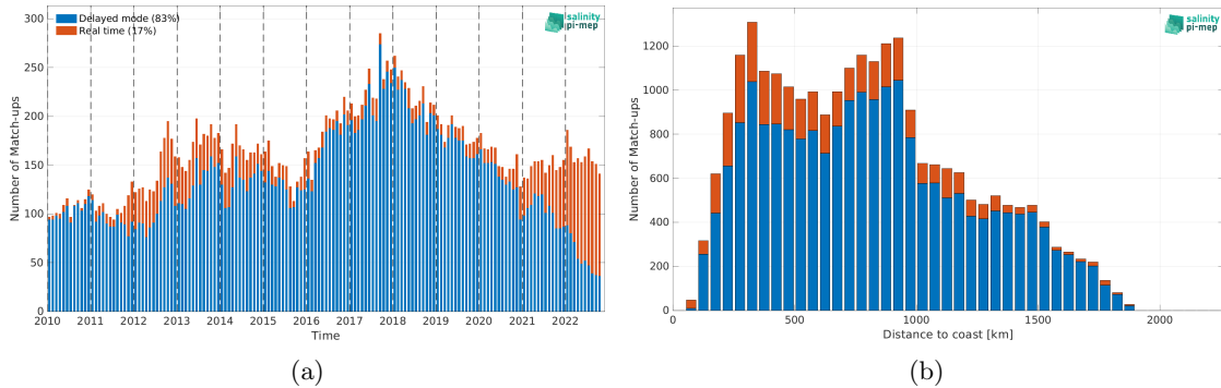
Figure 1: Number of match-ups between Argo and CCI SSS L4 Merged-OI v4.4 - 7-day running (ESA) SSS as a function of time (a) and as function of the distance to coast (b) over the Gulf Stream Pi-MEP region and for the full satellite product period.
