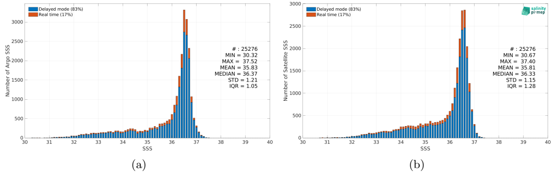
Figure 2: Histograms of SSS from Argo (a) and CCI SSS L4 Merged-OI v4.4 - 7-day running (ESA) (b) considering all match-up pairs per bins of 0.1 over the Gulf Stream Pi-MEP region and for the full satellite product period.
