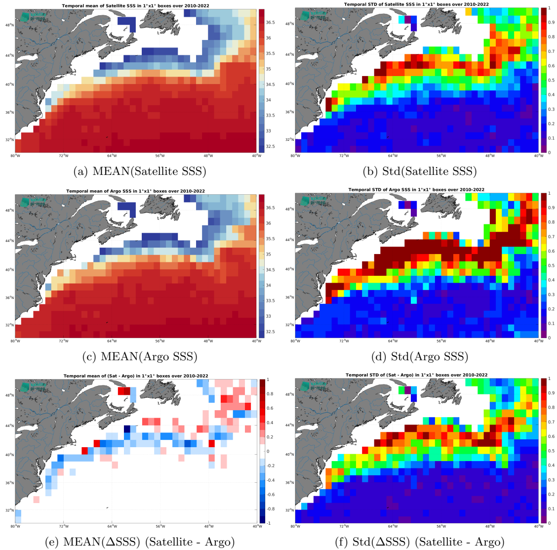
Figure 6: Temporal mean (left) and Std (right) of SSS from CCI SSS L4 Merged-OI v4.4 - 7-day running (ESA) (top), Argo (middle), and of \Delta SSS (Satellite - Argo). Only match-up pairs are used to generate these maps.
