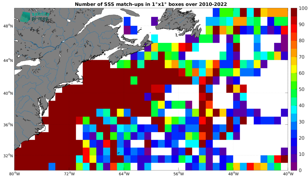
Figure 4: Number of SSS match-ups between TSG (SAMOS) SSS and the CCI SSS L4 Merged-OI v4.4 - 30-day running (ESA) SSS product for the Gulf Stream Pi-MEP region over 1^\circ \times 1^\circ boxes and for the full satellite product period.
