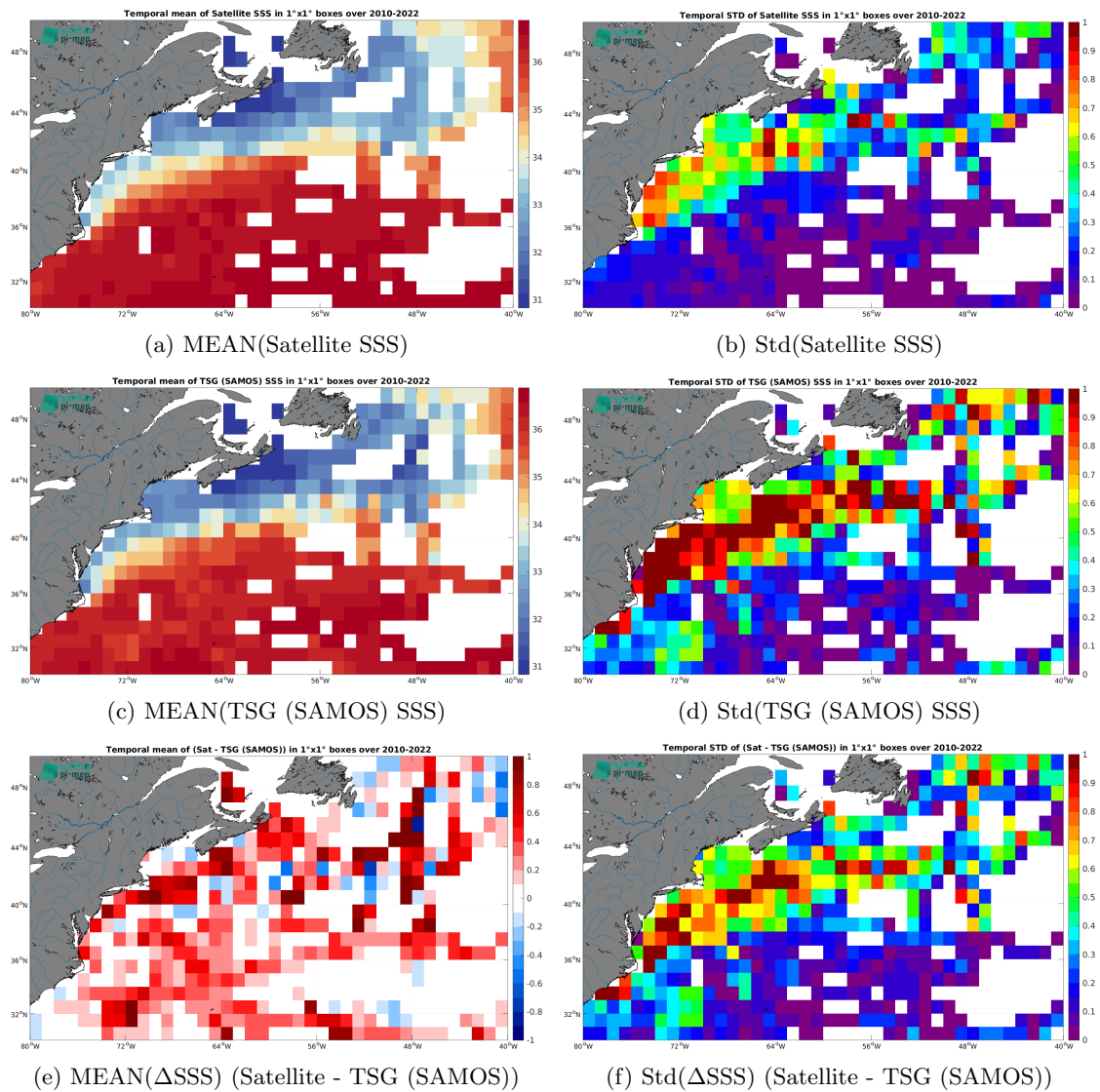
Figure 6: Temporal mean (left) and Std (right) of SSS from CCI SSS L4 Merged-OI v4.4 - 30-day running (ESA) (top), TSG (SAMOS) (middle), and of \Delta SSS (Satellite - TSG (SAMOS)). Only match-up pairs are used to generate these maps.
