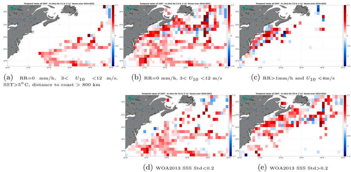
Figure 12: Temporal mean gridded over spatial boxes of size 1^\circ \times 1^\circ of \Delta\text{SSS} (CCI SSS L4 Merged-OI v4.4 - 30-day running (ESA) - TSG (SAMOS)) for 5 different subdatasets corresponding to:RR=0 mm/h, 3 < U_{10} < 12 m/s, SST >5^\circ\text{C} , distance to coast > 800 km (a), RR=0 mm/h, 3 < U_{10} < 12 m/s (b), RR >1 mm/h and U_{10} < 4 m/s (c), WOA2013 SSS Std <0.2 (d), WOA2013 SSS Std >0.2 (e).
