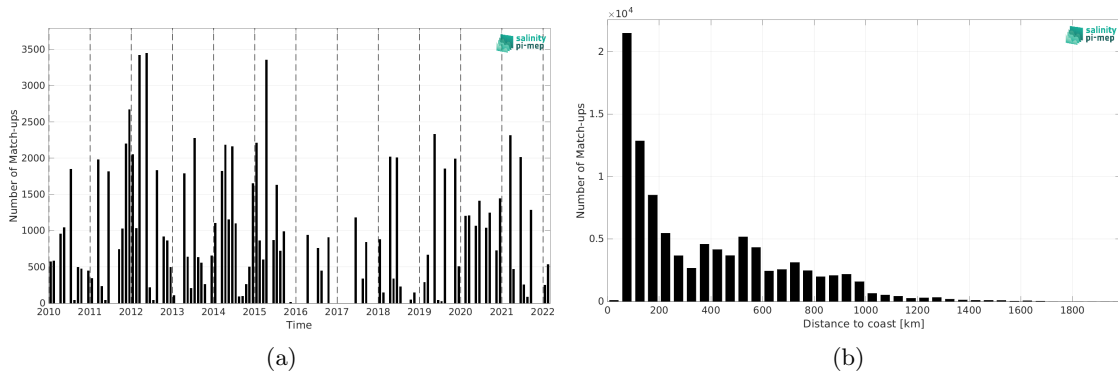
Figure 1: Number of match-ups between TSG (LEGOS-DM) and CCI SSS L4 Merged-OI v4.4 - 30-day running (ESA) SSS as a function of time (a) and as function of the distance to coast (b) over the Gulf Stream Pi-MEP region and for the full satellite product period.
