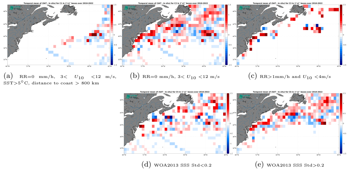
Figure 12: Temporal mean gridded over spatial boxes of size 1^{\circ}\times 1^{\circ} of \Delta\text{SSS} (CCI SSS L4 Merged-OI v4.4 - 30-day running (ESA) - TSG (LEGOS-DM)) for 5 different subdatasets corresponding to:RR=0 mm/h, 3 < U_{10} < 12 m/s, SST >5^{\circ}\text{C} , distance to coast > 800 km (a), RR=0 mm/h, 3 < U_{10} < 12 m/s (b), RR >1 mm/h and U_{10} < 4 m/s (c), WOA2013 SSS Std <0.2 (d), WOA2013 SSS Std >0.2 (e).
