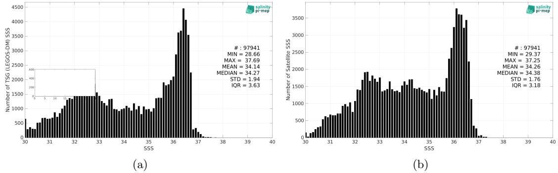
Figure 2: Histograms of SSS from TSG (LEGOS-DM) (a) and CCI SSS L4 Merged-OI v4.4 - 30-day running (ESA) (b) considering all match-up pairs per bins of 0.1 over the Gulf Stream Pi-MEP region and for the full satellite product period.
