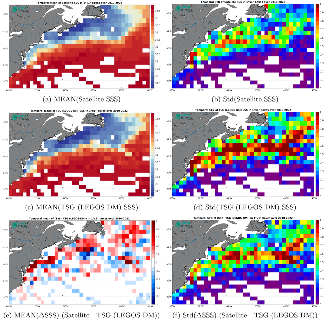
Figure 6: Temporal mean (left) and Std (right) of SSS from CCI SSS L4 Merged-OI v4.4 - 30-day running (ESA) (top), TSG (LEGOS-DM) (middle), and of \Delta SSS (Satellite - TSG (LEGOS-DM)). Only match-up pairs are used to generate these maps.
