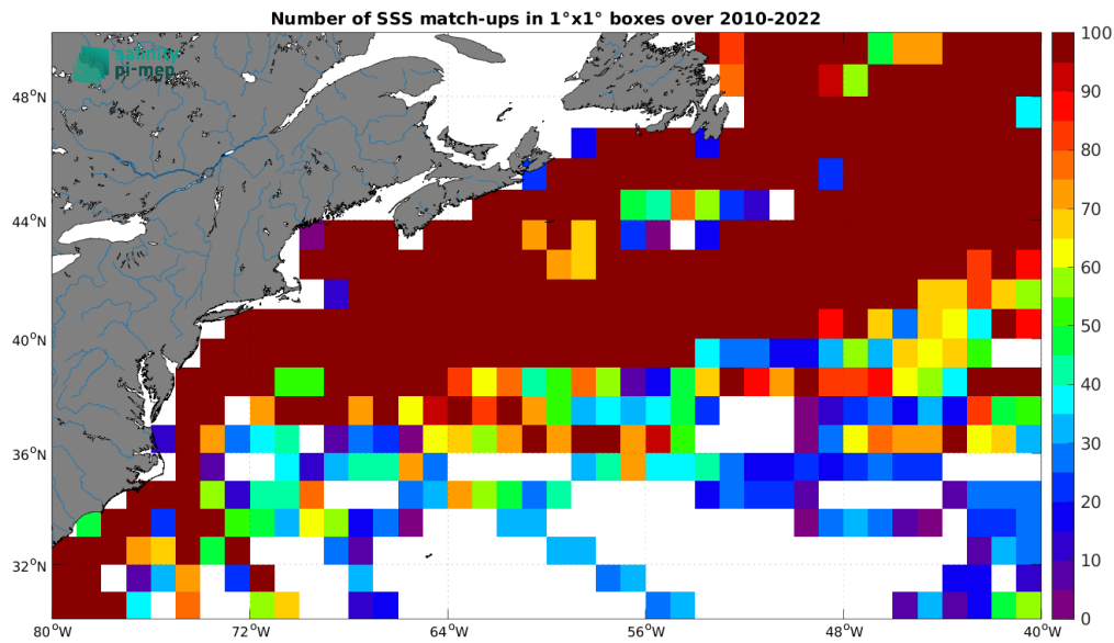
Figure 4: Number of SSS match-ups between TSG (LEGOS-DM) SSS and the CCI SSS L4 Merged-OI v4.4 - 30-day running (ESA) SSS product for the Gulf Stream Pi-MEP region over 1^\circ \times 1^\circ boxes and for the full satellite product period.
