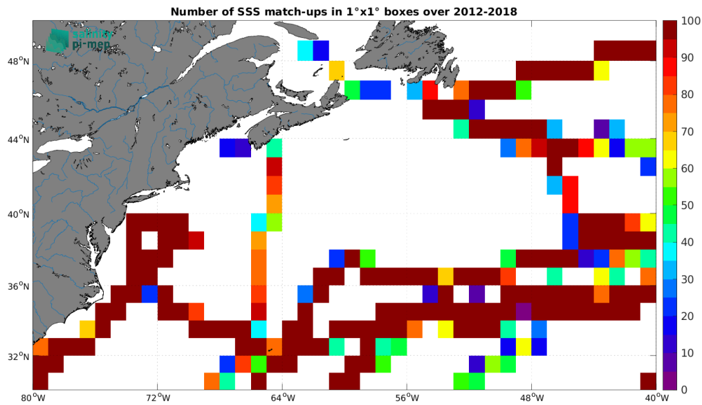
Figure 4: Number of SSS match-ups between TSG (GOSUD-Sailing-ship) SSS and the CCI SSS L4 Merged-OI v4.4 - 30-day running (ESA) SSS product for the Gulf Stream Pi-MEP region over 1^\circ \times 1^\circ boxes and for the full satellite product period.
