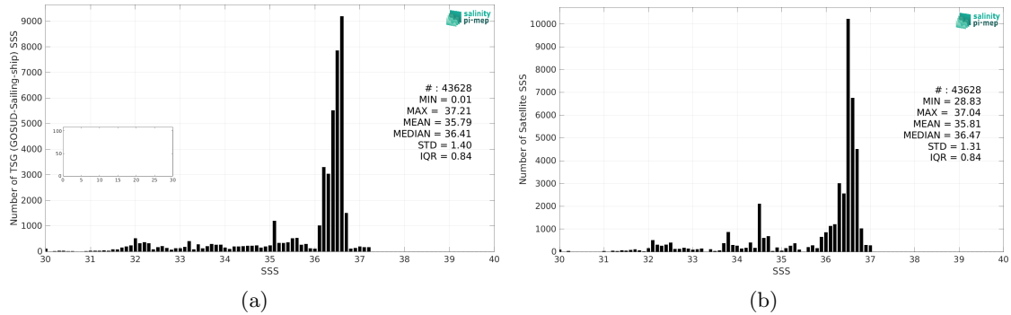
Figure 2: Histograms of SSS from TSG (GOSUD-Sailing-ship) (a) and CCI SSS L4 Merged-OI v4.4 - 30-day running (ESA) (b) considering all match-up pairs per bins of 0.1 over the Gulf Stream Pi-MEP region and for the full satellite product period.
