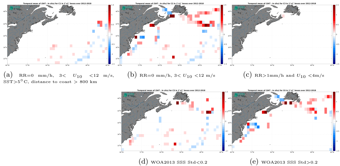
Figure 12: Temporal mean gridded over spatial boxes of size 1^{\circ}\times 1^{\circ} of \Delta SSS (CCI SSS L4 Merged-OI v4.4 - 30-day running (ESA) - TSG (GOSUD-Sailing-ship)) for 5 different subdatasets corresponding to:RR=0 mm/h, 3 < U_{10} < 12 m/s, SST > 5^{\circ}\text{C} , distance to coast > 800 km (a), RR=0 mm/h, 3 < U_{10} < 12 m/s (b), RR > 1 mm/h and U_{10} < 4 m/s (c), WOA2013 SSS Std < 0.2 (d), WOA2013 SSS Std > 0.2 (e).
