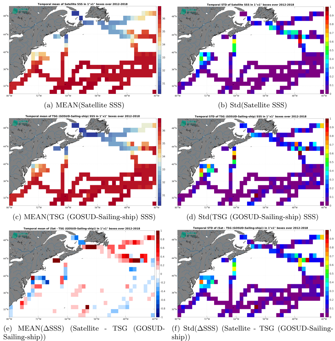
Figure 6: Temporal mean (left) and Std (right) of SSS from CCI SSS L4 Merged-OI v4.4 - 30-day running (ESA) (top), TSG (GOSUD-Sailing-ship) (middle), and of \Delta SSS (Satellite - TSG (GOSUD-Sailing-ship)). Only match-up pairs are used to generate these maps.
