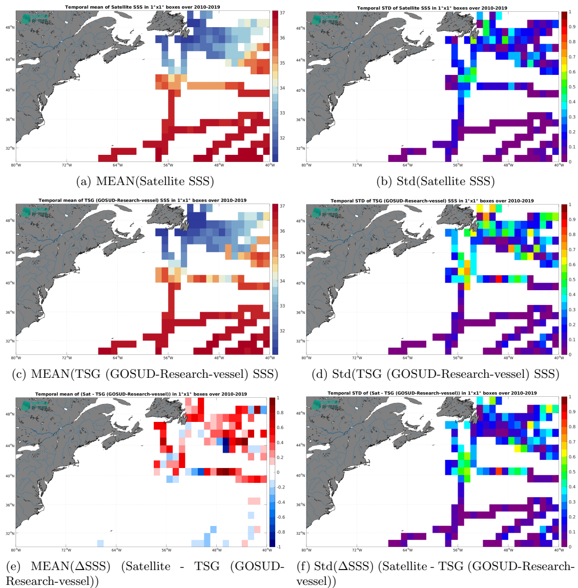
Figure 6: Temporal mean (left) and Std (right) of SSS from CCI SSS L4 Merged-OI v4.4 - 30-day running (ESA) (top), TSG (GOSUD-Research-vessel) (middle), and of \Delta SSS (Satellite - TSG (GOSUD-Research-vessel)). Only match-up pairs are used to generate these maps.
