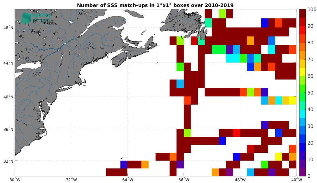
Figure 4: Number of SSS match-ups between TSG (GOSUD-Research-vessel) SSS and the CCI SSS L4 Merged-OI v4.4 - 30-day running (ESA) SSS product for the Gulf Stream Pi-MEP region over 1^\circ \times 1^\circ boxes and for the full satellite product period.
