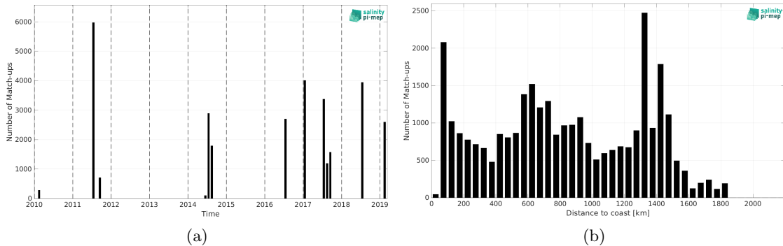
Figure 1: Number of match-ups between TSG (GOSUD-Research-vessel) and CCI SSS L4 Merged-OI v4.4 - 30-day running (ESA) SSS as a function of time (a) and as function of the distance to coast (b) over the Gulf Stream Pi-MEP region and for the full satellite product period.
