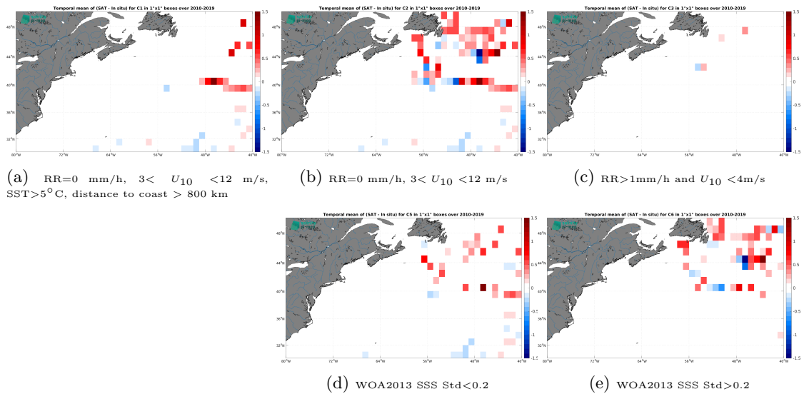
Figure 12: Temporal mean gridded over spatial boxes of size 1^\circ \times 1^\circ of \Delta SSS (CCI SSS L4 Merged-OI v4.4 - 30-day running (ESA) - TSG (GOSUD-Research-vessel)) for 5 different subdatasets corresponding to:RR=0 mm/h, 3 < U_{10} < 12 m/s, SST >5^\circ\text{C} , distance to coast > 800 km (a), RR=0 mm/h, 3 < U_{10} < 12 m/s (b), RR >1 mm/h and U_{10} < 4 m/s (c), WOA2013 SSS Std <0.2 (d), WOA2013 SSS Std >0.2 (e).
