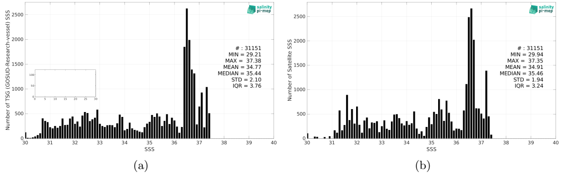
Figure 2: Histograms of SSS from TSG (GOSUD-Research-vessel) (a) and CCI SSS L4 Merged-OI v4.4 - 30-day running (ESA) (b) considering all match-up pairs per bins of 0.1 over the Gulf Stream Pi-MEP region and for the full satellite product period.
