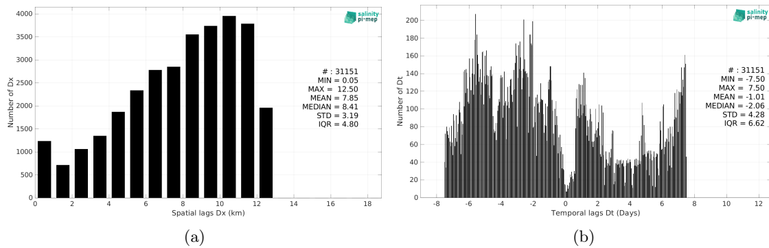
Figure 5: Histograms of the spatial (a) and temporal (b) lags between the location/time of the TSG (GOSUD-Research-vessel) measurement and the date of the corresponding CCI SSS L4 Merged-OI v4.4 - 30-day running (ESA) SSS pixel.
