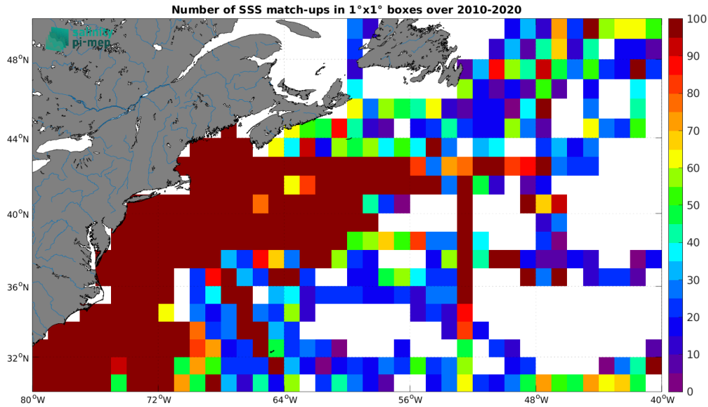
Figure 4: Number of SSS match-ups between TSG (SAMOS) SSS and the CCI SSS L4 Merged-OI v3.2 - 7-day running (ESA) SSS product for the Gulf Stream Pi-MEP region over 1^\circ \times 1^\circ boxes and for the full satellite product period.
