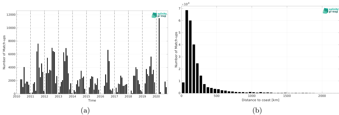
Figure 1: Number of match-ups between TSG (SAMOS) and CCI SSS L4 Merged-OI v3.2 - 7-day running (ESA) SSS as a function of time (a) and as function of the distance to coast (b) over the Gulf Stream Pi-MEP region and for the full satellite product period.
