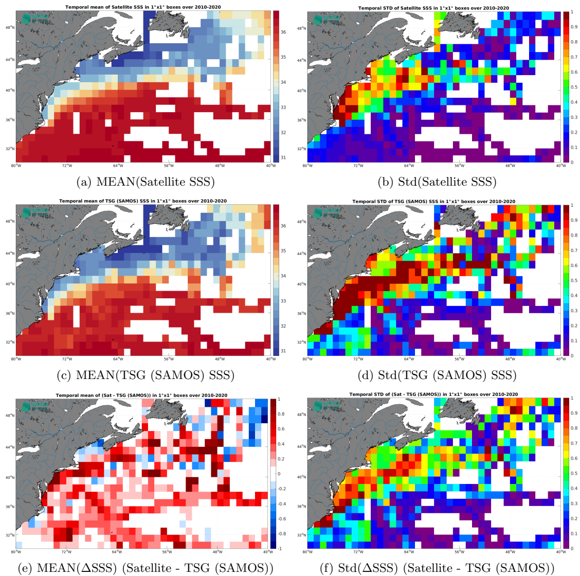
Figure 6: Temporal mean (left) and Std (right) of SSS from CCI SSS L4 Merged-OI v3.2 - 7-day running (ESA) (top), TSG (SAMOS) (middle), and of \Delta SSS (Satellite - TSG (SAMOS)). Only match-up pairs are used to generate these maps.
