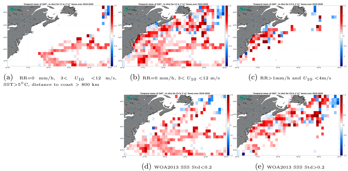
Figure 12: Temporal mean gridded over spatial boxes of size 1^\circ \times 1^\circ of \Delta\text{SSS} (CCI SSS L4 Merged-OI v3.2 - 7-day running (ESA) - TSG (SAMOS)) for 5 different subdatasets corresponding to:RR=0 mm/h, 3 < U_{10} < 12 m/s, SST >5^\circ\text{C} , distance to coast > 800 km (a), RR=0 mm/h, 3 < U_{10} < 12 m/s (b), RR >1 mm/h and U_{10} < 4 m/s (c), WOA2013 SSS Std <0.2 (d), WOA2013 SSS Std >0.2 (e).
