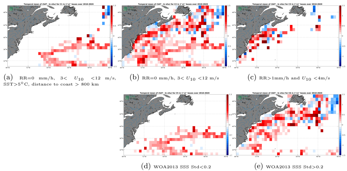
Figure 12: Temporal mean gridded over spatial boxes of size 1°x1° of \Delta SSS (CCI SSS L4 Merged-OI v3.2 - 7-day running (ESA) - TSG (SAMOS)) for 5 different subdatasets corresponding to:RR=0 mm/h, 3 < U_{10} < 12 m/s, SST>5°C, distance to coast > 800 km (a), RR=0 mm/h, 3 < U_{10} < 12 m/s (b), RR>1mm/h and U_{10} < 4m/s (c), WOA2013 SSS Std<0.2 (d), WOA2013 SSS Std>0.2 (e).
