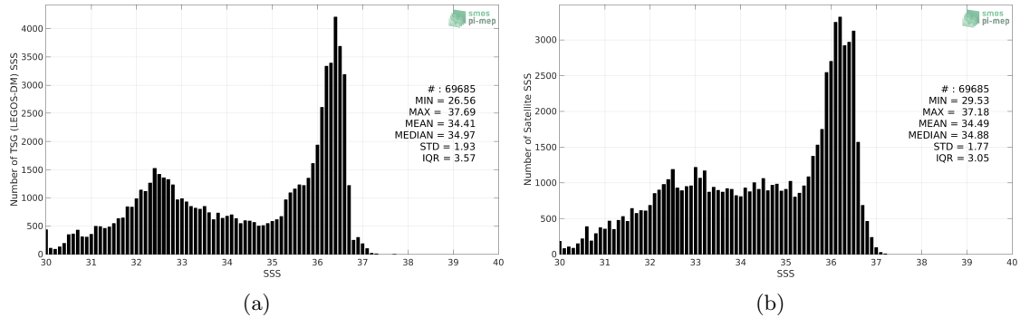
Figure 2: Histograms of SSS from TSG (LEGOS-DM) (a) and CCI SSS L4 Merged-OI v3.2 - 7-day running (ESA) (b) considering all match-up pairs per bins of 0.1 over the Gulf Stream Pi-MEP region and for the full satellite product period.
