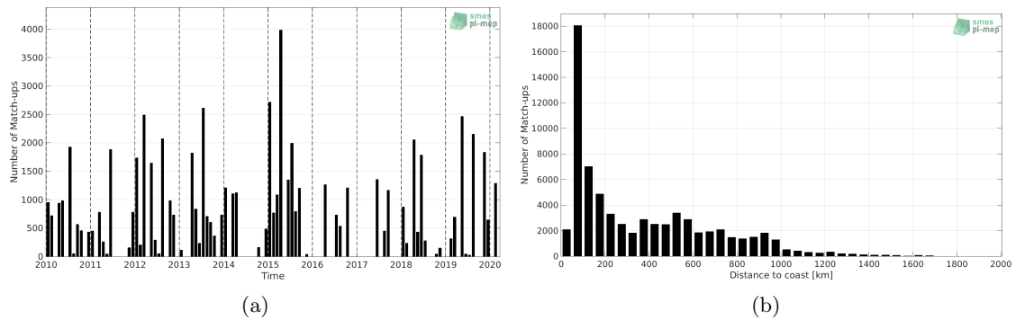
Figure 1: Number of match-ups between TSG (LEGOS-DM) and CCI SSS L4 Merged-OI v3.2 - 7-day running (ESA) SSS as a function of time (a) and as function of the distance to coast (b) over the Gulf Stream Pi-MEP region and for the full satellite product period.
