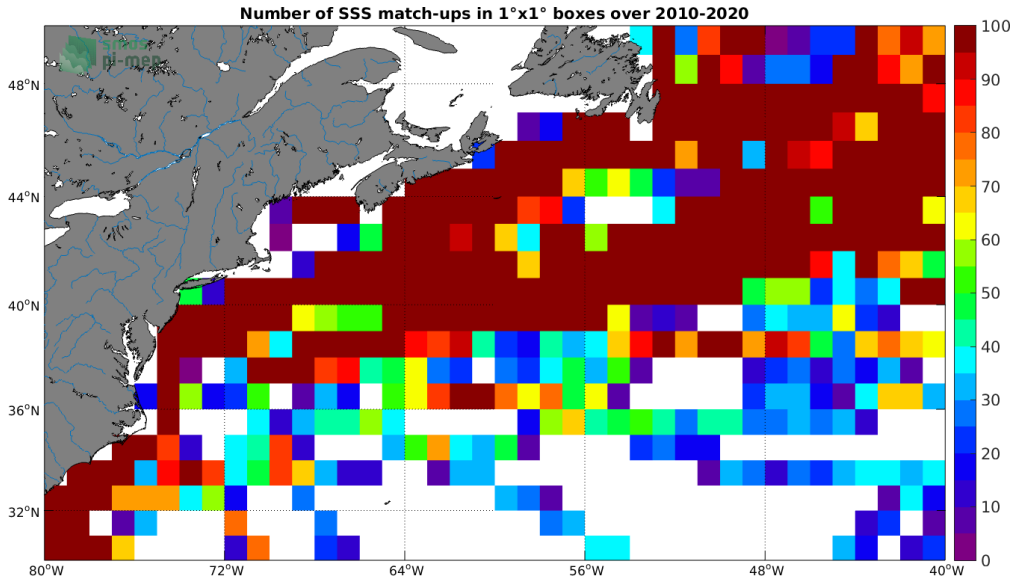
Figure 4: Number of SSS match-ups between TSG (LEGOS-DM) SSS and the CCI SSS L4 Merged-OI v3.2 - 7-day running (ESA) SSS product for the Gulf Stream Pi-MEP region over 1^\circ \times 1^\circ boxes and for the full satellite product period.
