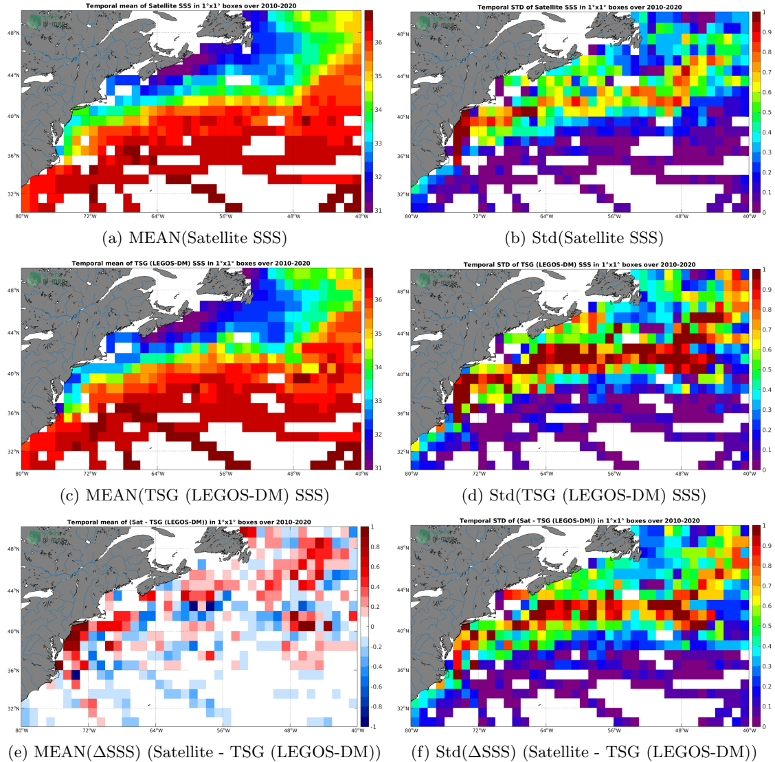
Figure 6: Temporal mean (left) and Std (right) of SSS from CCI SSS L4 Merged-OI v3.2 - 7-day running (ESA) (top), TSG (LEGOS-DM) (middle), and of \Delta SSS (Satellite - TSG (LEGOS-DM)). Only match-up pairs are used to generate these maps.
