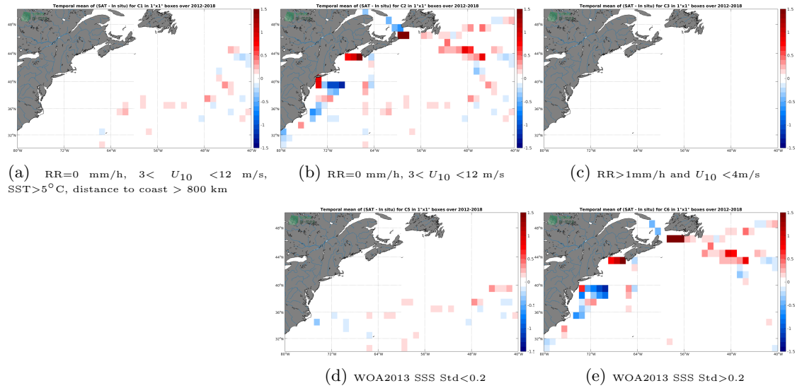
Figure 12: Temporal mean gridded over spatial boxes of size 1^\circ \times 1^\circ of \Delta SSS (CCI SSS L4 Merged-OI v3.2 - 7-day running (ESA) - TSG (GOSUD-Sailing-ship)) for 5 different subdatasets corresponding to: RR=0 mm/h, 3 < U_{10} < 12 m/s, SST > 5^\circ\text{C} , distance to coast > 800 km (a), RR=0 mm/h, 3 < U_{10} < 12 m/s (b), RR > 1 mm/h and U_{10} < 4 m/s (c), WOA2013 SSS Std < 0.2 (d), WOA2013 SSS Std > 0.2 (e).
