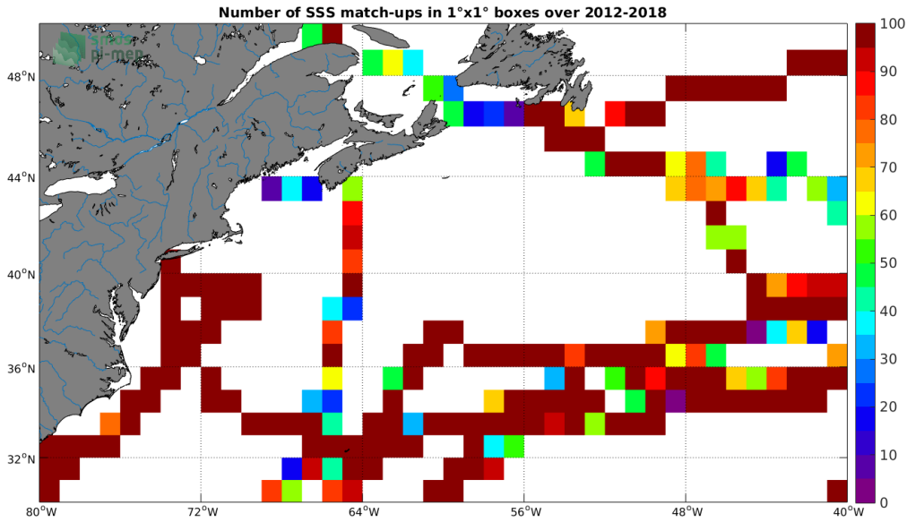
Figure 4: Number of SSS match-ups between TSG (GOSUD-Sailing-ship) SSS and the CCI SSS L4 Merged-OI v3.2 - 7-day running (ESA) SSS product for the Gulf Stream Pi-MEP region over 1^{\circ} \times 1^{\circ} boxes and for the full satellite product period.
