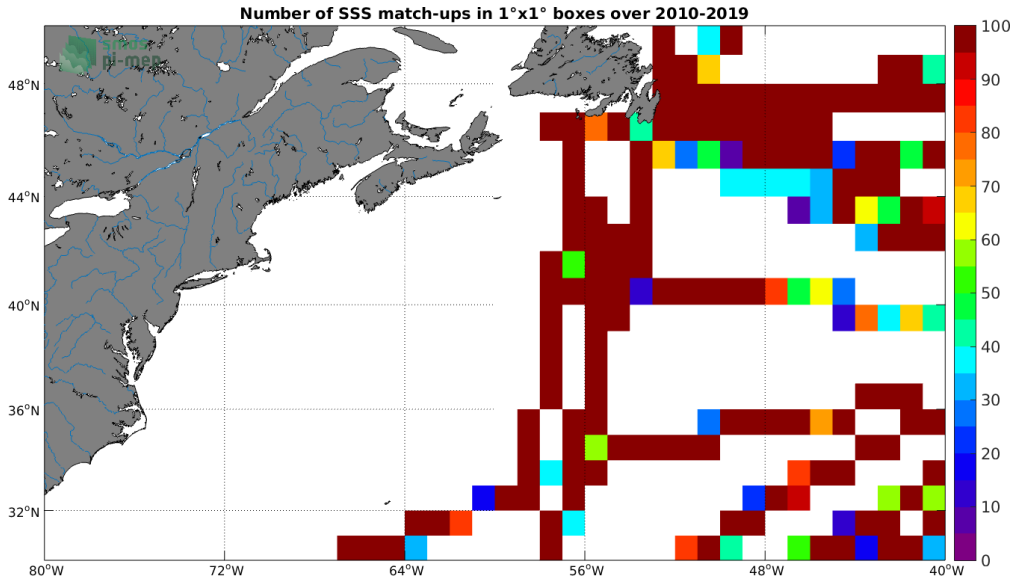
Figure 4: Number of SSS match-ups between TSG (GOSUD-Research-vessel) SSS and the CCI SSS L4 Merged-OI v3.2 - 7-day running (ESA) SSS product for the Gulf Stream Pi-MEP region over 1^{\circ} \times 1^{\circ} boxes and for the full satellite product period.
