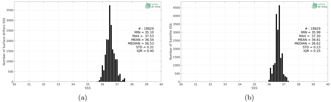
Figure 2: Histograms of SSS from Surface drifters (a) and CCI SSS L4 Merged-OI v3.2 - 7-day running (ESA) (b) considering all match-up pairs per bins of 0.1 over the Gulf Stream Pi-MEP region and for the full satellite product period.
