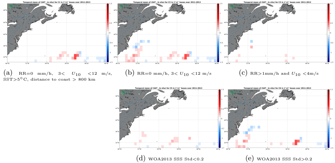
Figure 11: Temporal mean gridded over spatial boxes of size 1^{\circ}\times 1^{\circ} of \Delta\text{SSS} (CCI SSS L4 Merged-OI v3.2 - 7-day running (ESA) - Surface drifters) for 5 different subdatasets corresponding to:RR=0 mm/h, 3 < U_{10} < 12 m/s, SST >5^{\circ}\text{C} , distance to coast > 800 km (a), RR=0 mm/h, 3 < U_{10} < 12 m/s (b), RR >1 mm/h and U_{10} < 4 m/s (c), WOA2013 SSS Std <0.2 (d), WOA2013 SSS Std >0.2 (e).
