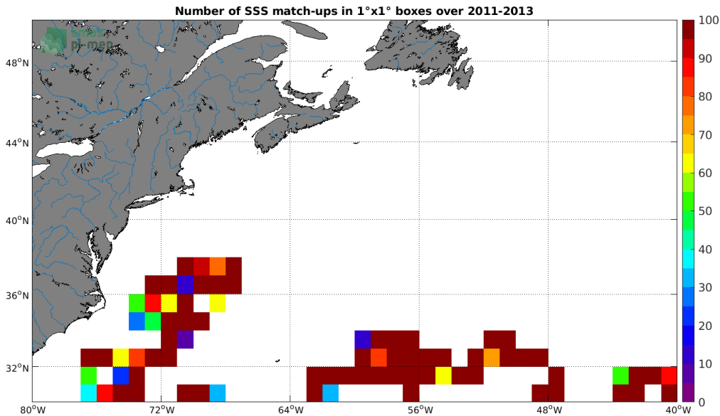
Figure 3: Number of SSS match-ups between Surface drifters SSS and the CCI SSS L4 Merged-OI v3.2 - 7-day running (ESA) SSS product for the Gulf Stream Pi-MEP region over 1^\circ \times 1^\circ boxes and for the full satellite product period.
