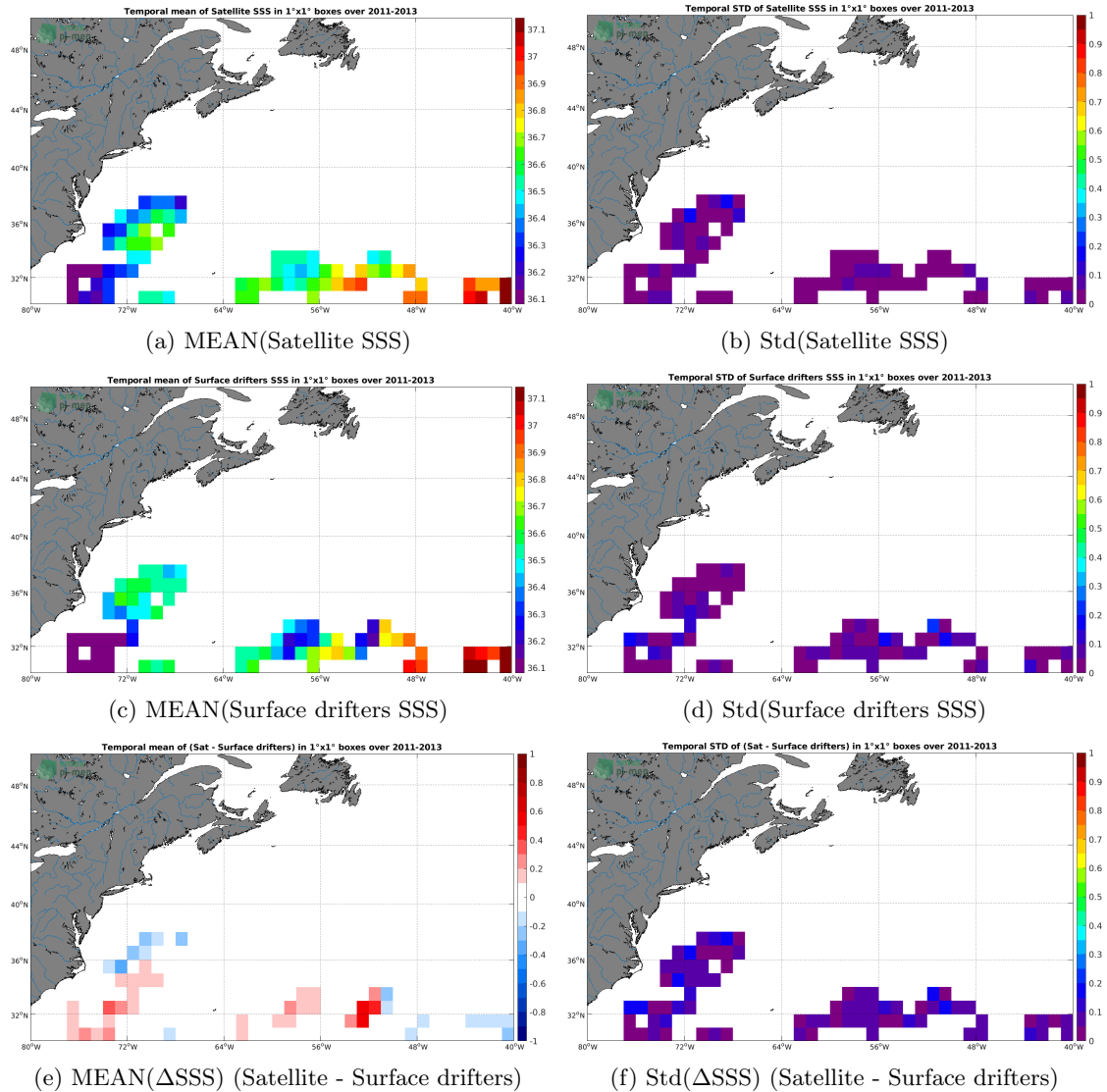
Figure 5: Temporal mean (left) and Std (right) of SSS from CCI SSS L4 Merged-OI v3.2 - 7-day running (ESA) (top), Surface drifters (middle), and of \Delta SSS (Satellite - Surface drifters). Only match-up pairs are used to generate these maps.
