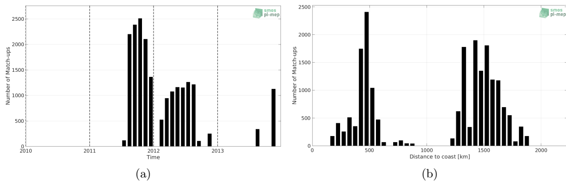
Figure 1: Number of match-ups between Surface drifters and CCI SSS L4 Merged-OI v3.2 - 7-day running (ESA) SSS as a function of time (a) and as function of the distance to coast (b) over the Gulf Stream Pi-MEP region and for the full satellite product period.
