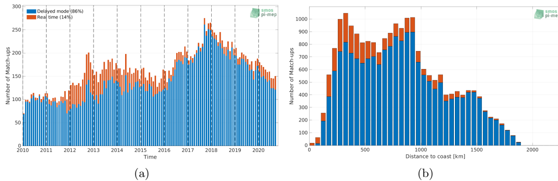
Figure 1: Number of match-ups between Argo and CCI SSS L4 Merged-OI v3.2 - 7-day running (ESA) SSS as a function of time (a) and as function of the distance to coast (b) over the Gulf Stream Pi-MEP region and for the full satellite product period.
