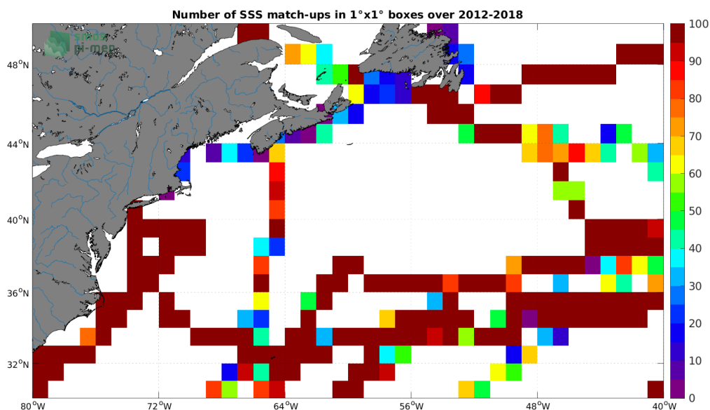
Figure 4: Number of SSS match-ups between TSG (GOSUD-Sailing-ship) SSS and the CCI SSS L4 Merged-OI v3.2 - 30-day running (ESA) SSS product for the Gulf Stream Pi-MEP region over 1^\circ \times 1^\circ boxes and for the full satellite product period.
