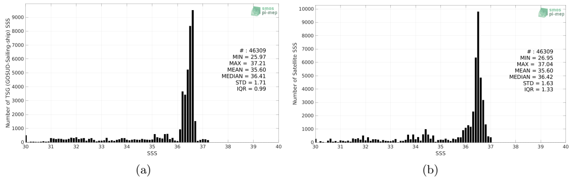
Figure 2: Histograms of SSS from TSG (GOSUD-Sailing-ship) (a) and CCI SSS L4 Merged-OI v3.2 - 30-day running (ESA) (b) considering all match-up pairs per bins of 0.1 over the Gulf Stream Pi-MEP region and for the full satellite product period.
