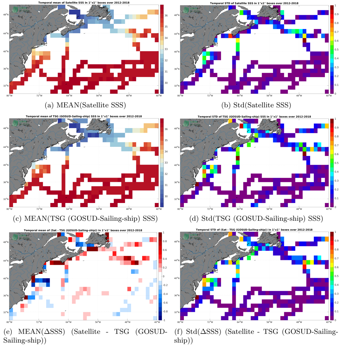
Figure 6: Temporal mean (left) and Std (right) of SSS from CCI SSS L4 Merged-OI v3.2 - 30-day running (ESA) (top), TSG (GOSUD-Sailing-ship) (middle), and of \Delta SSS (Satellite - TSG (GOSUD-Sailing-ship)). Only match-up pairs are used to generate these maps.
