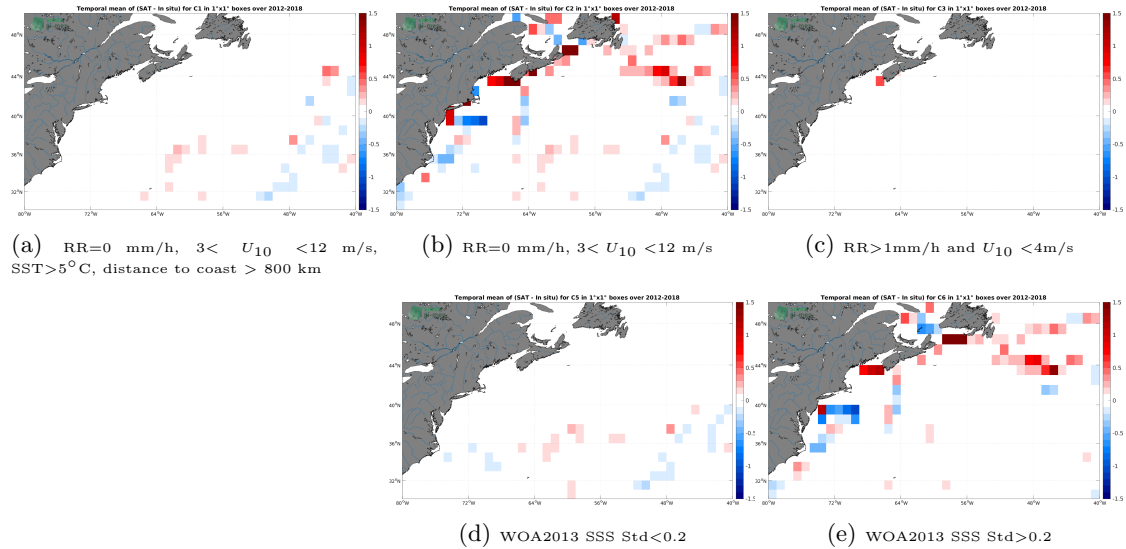
Figure 12: Temporal mean gridded over spatial boxes of size 1^{\circ}\times 1^{\circ} of \Delta SSS (CCI SSS L4 Merged-OI v3.2 - 30-day running (ESA) - TSG (GOSUD-Sailing-ship)) for 5 different subdatasets corresponding to:RR=0 mm/h, 3 < U_{10} < 12 m/s, SST > 5^{\circ}\text{C} , distance to coast > 800 km (a), RR=0 mm/h, 3 < U_{10} < 12 m/s (b), RR > 1 mm/h and U_{10} < 4 m/s (c), WOA2013 SSS Std < 0.2 (d), WOA2013 SSS Std > 0.2 (e).
