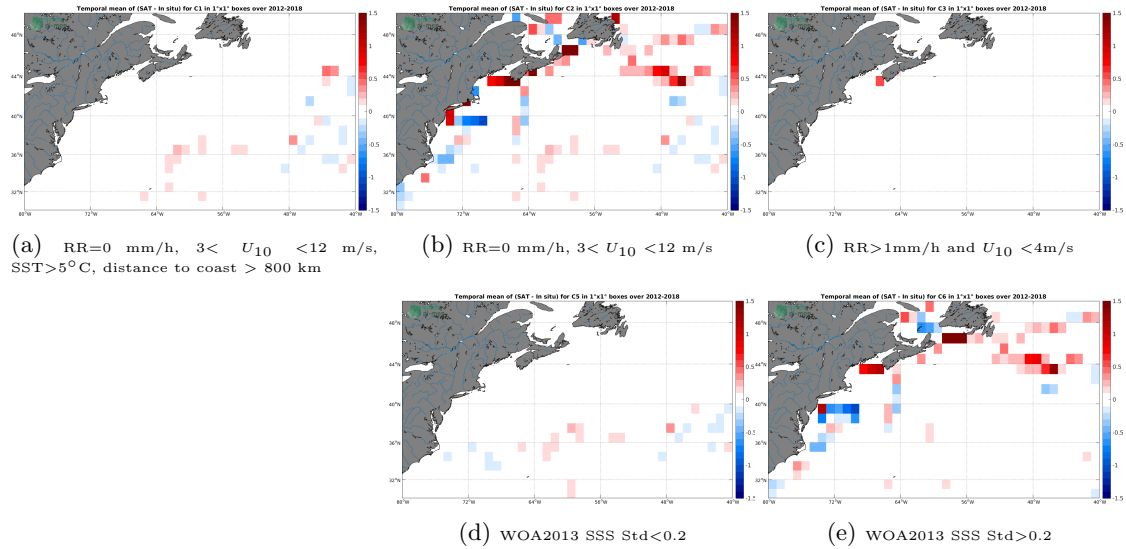
Figure 12: Temporal mean gridded over spatial boxes of size 1^\circ \times 1^\circ of \Delta SSS (CCI SSS L4 Merged-OI v3.2 - 30-day running (ESA) - TSG (GOSUD-Sailing-ship)) for 5 different subdatasets corresponding to:RR=0 mm/h, 3 < U_{10} < 12 m/s, SST >5^\circ\text{C} , distance to coast > 800 km (a), RR=0 mm/h, 3 < U_{10} < 12 m/s (b), RR >1 mm/h and U_{10} < 4 m/s (c), WOA2013 SSS Std <0.2 (d), WOA2013 SSS Std >0.2 (e).
