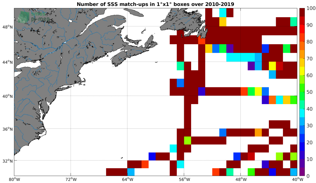
Figure 4: Number of SSS match-ups between TSG (GOSUD-Research-vessel) SSS and the CCI SSS L4 Merged-OI v3.2 - 30-day running (ESA) SSS product for the Gulf Stream Pi-MEP region over 1°x1° boxes and for the full satellite product period.
