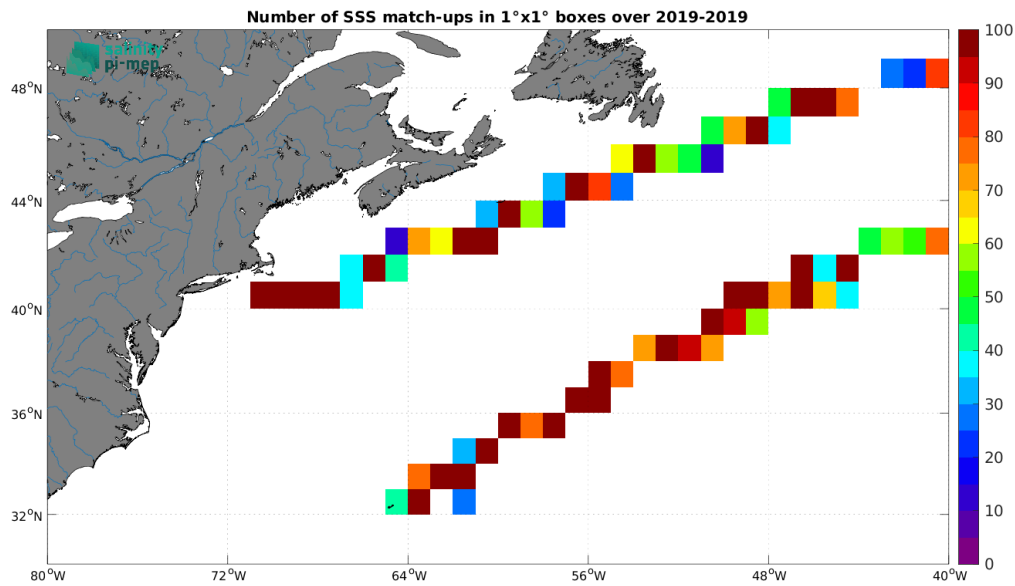
Figure 4: Number of SSS match-ups between Saildrone SSS and the CCI SSS L4 Merged-OI v3.2 - 30-day running (ESA) SSS product for the Gulf Stream Pi-MEP region over 1^\circ \times 1^\circ boxes and for the full satellite product period.
