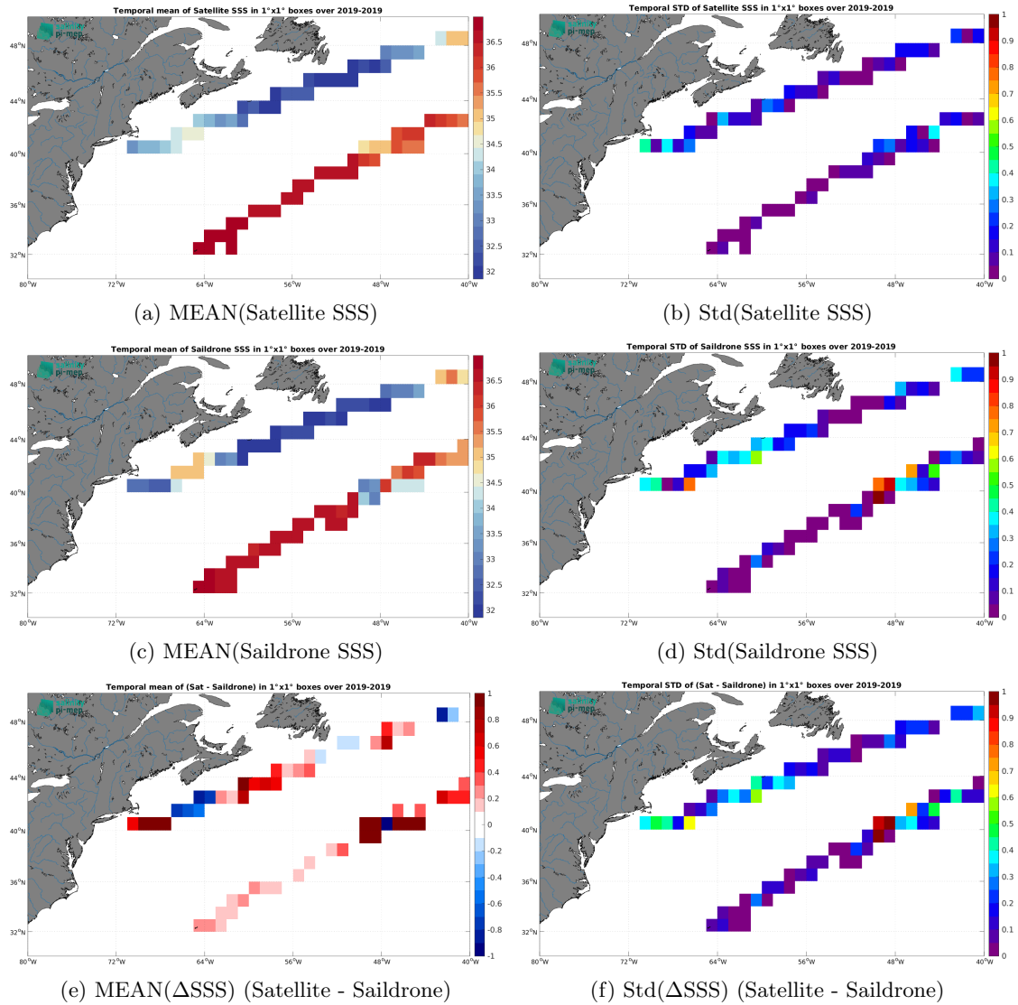
Figure 6: Temporal mean (left) and Std (right) of SSS from CCI SSS L4 Merged-OI v3.2 - 30-day running (ESA) (top), Saildrone (middle), and of \Delta SSS (Satellite - Saildrone). Only match-up pairs are used to generate these maps.
