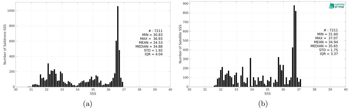
Figure 2: Histograms of SSS from Saildrone (a) and CCI SSS L4 Merged-OI v3.2 - 30-day running (ESA) (b) considering all match-up pairs per bins of 0.1 over the Gulf Stream Pi-MEP region and for the full satellite product period.
