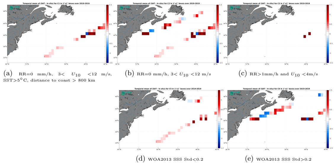
Figure 12: Temporal mean gridded over spatial boxes of size 1^\circ \times 1^\circ of \Delta SSS (CCI SSS L4 Merged-OI v3.2 - 30-day running (ESA) - Saildrone) for 5 different subdatasets corresponding to: RR=0 mm/h, 3 < U_{10} < 12 m/s, SST > 5^\circ C , distance to coast > 800 km (a), RR=0 mm/h, 3 < U_{10} < 12 m/s (b), RR > 1 mm/h and U_{10} < 4 m/s (c), WOA2013 SSS Std < 0.2 (d), WOA2013 SSS Std > 0.2 (e).
