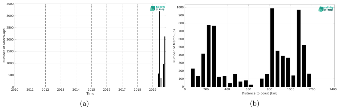
Figure 1: Number of match-ups between Saildrone and CCI SSS L4 Merged-OI v3.2 - 30-day running (ESA) SSS as a function of time (a) and as function of the distance to coast (b) over the Gulf Stream Pi-MEP region and for the full satellite product period.
