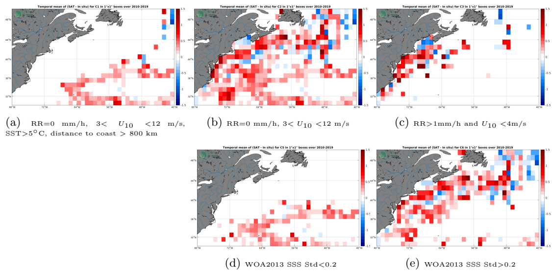
Figure 12: Temporal mean gridded over spatial boxes of size 1^\circ \times 1^\circ of \Delta SSS (CCI SSS L4 Merged-OI v2.31 - 7-day running (ESA) - TSG (SAMOS)) for 5 different subdatasets corresponding to:RR=0 mm/h, 3 < U_{10} < 12 m/s, SST >5^\circ\text{C} , distance to coast > 800 km (a), RR=0 mm/h, 3 < U_{10} < 12 m/s (b), RR >1 mm/h and U_{10} < 4 m/s (c), WOA2013 SSS Std <0.2 (d), WOA2013 SSS Std >0.2 (e).
