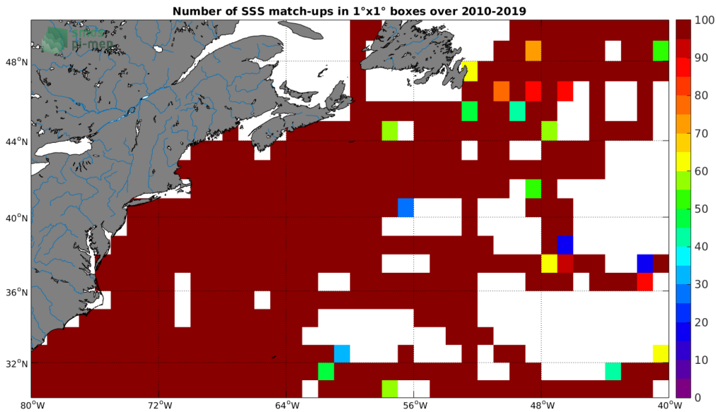
Figure 4: Number of SSS match-ups between TSG (SAMOS) SSS and the CCI SSS L4 Merged-OI v2.31 - 7-day running (ESA) SSS product for the Gulf Stream Pi-MEP region over 1^\circ \times 1^\circ boxes and for the full satellite product period.
