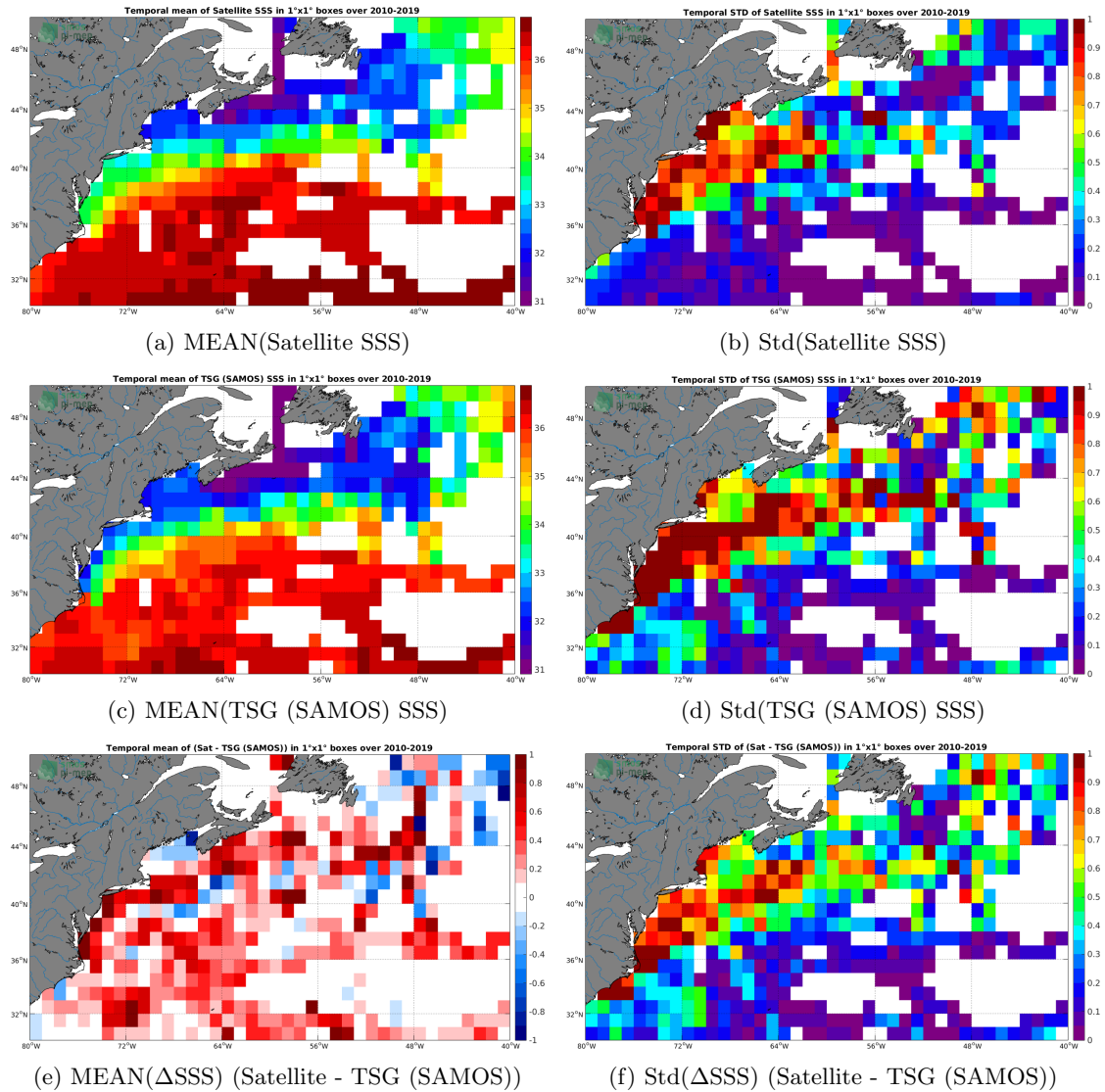
Figure 6: Temporal mean (left) and Std (right) of SSS from CCI SSS L4 Merged-OI v2.31 - 7-day running (ESA) (top), TSG (SAMOS) (middle), and of \Delta SSS (Satellite - TSG (SAMOS)). Only match-up pairs are used to generate these maps.
