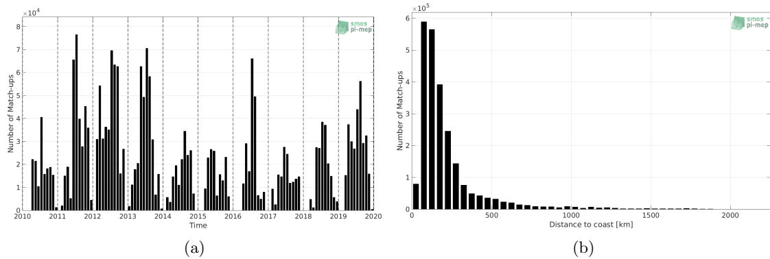
Figure 1: Number of match-ups between TSG (SAMOS) and CCI SSS L4 Merged-OI v2.31 - 7-day running (ESA) SSS as a function of time (a) and as function of the distance to coast (b) over the Gulf Stream Pi-MEP region and for the full satellite product period.
