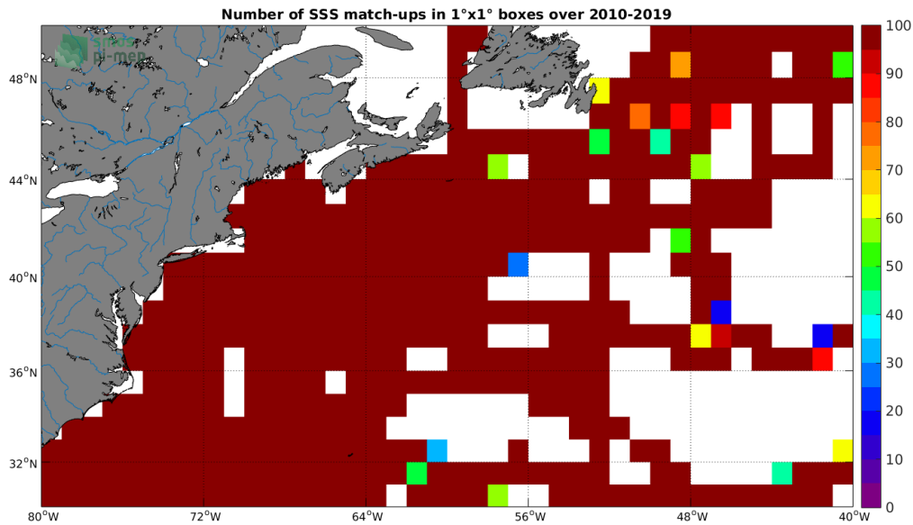
Figure 4: Number of SSS match-ups between TSG (SAMOS) SSS and the CCI L4 Merged-OI v2.31 - 7-day running (ESA) SSS product for the Gulf Stream Pi-MEP region over 1^\circ \times 1^\circ boxes and for the full satellite product period.
