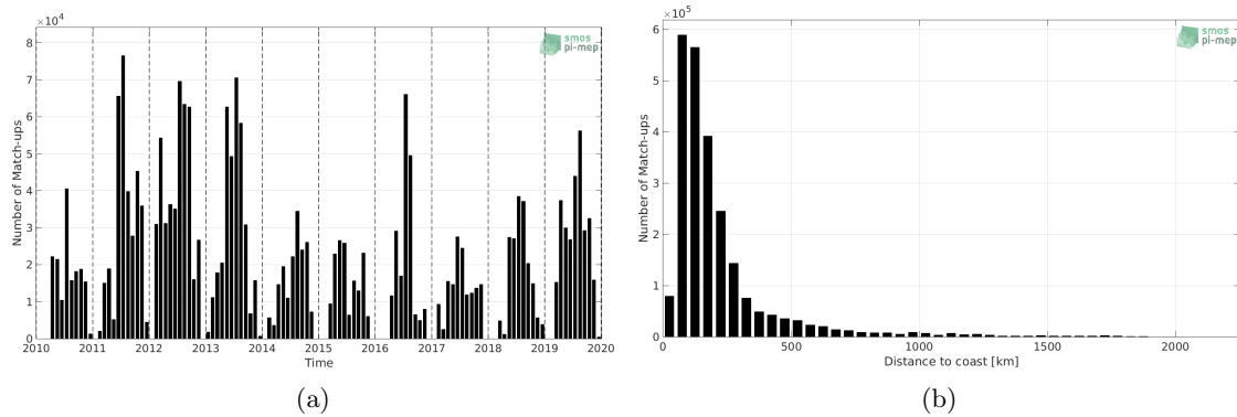
Figure 1: Number of match-ups between TSG (SAMOS) and CCI L4 Merged-OI v2.31 - 7-day running (ESA) SSS as a function of time (a) and as function of the distance to coast (b) over the Gulf Stream Pi-MEP region and for the full satellite product period.
