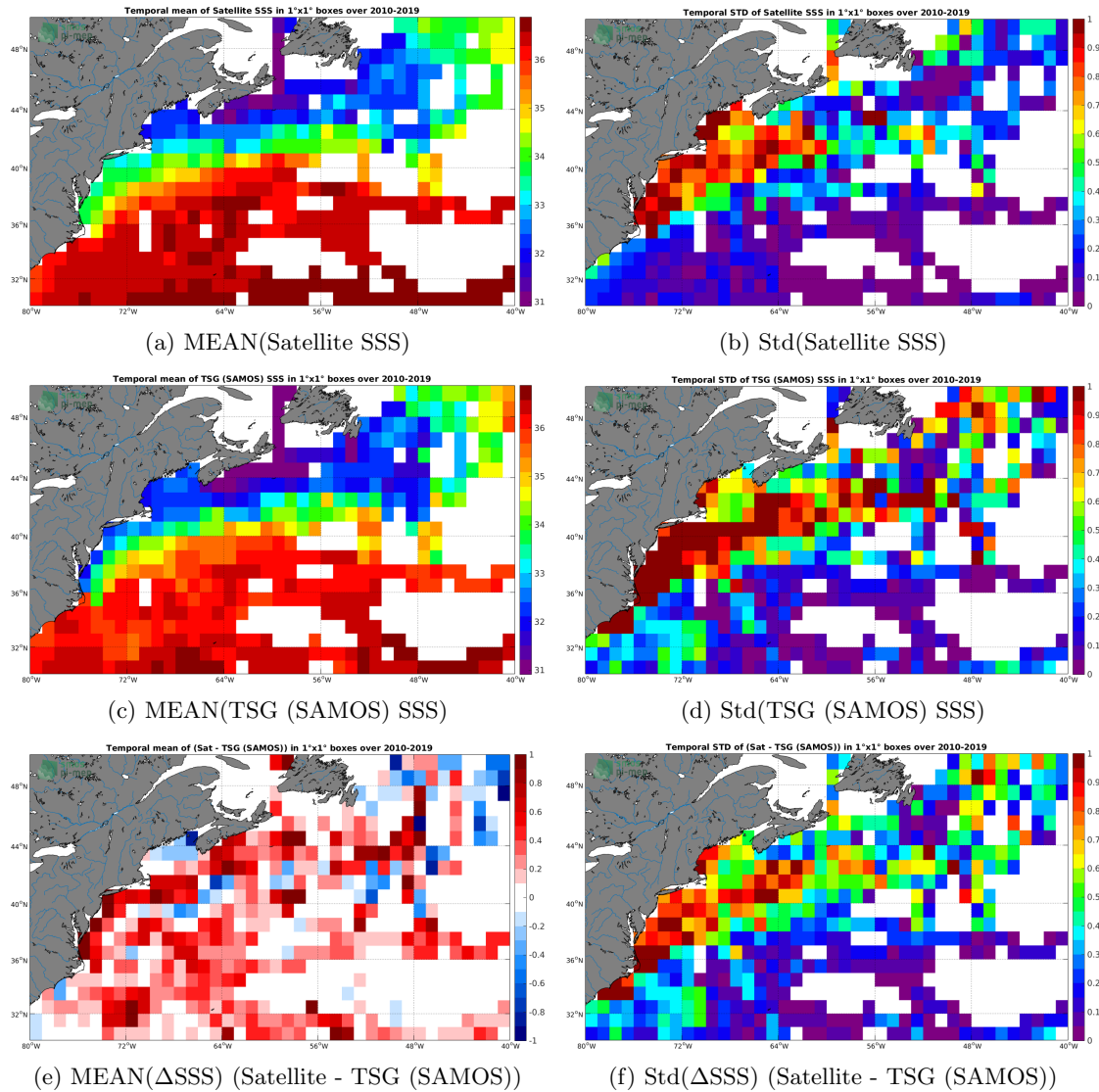
Figure 6: Temporal mean (left) and Std (right) of SSS from CCI L4 Merged-OI v2.31 - 7-day running (ESA) (top), TSG (SAMOS) (middle), and of \Delta SSS (Satellite - TSG (SAMOS)). Only match-up pairs are used to generate these maps.
