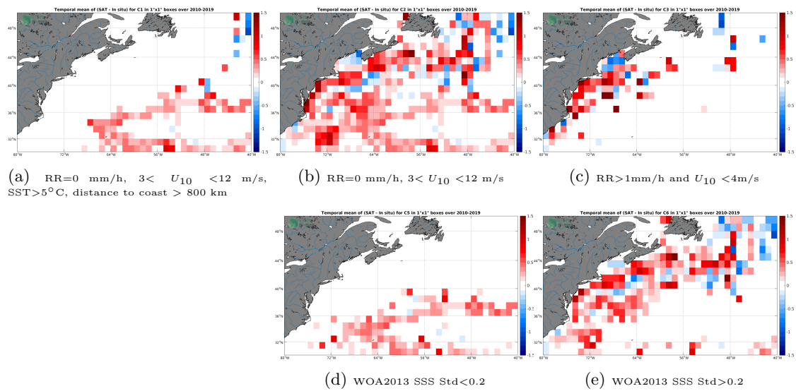
Figure 12: Temporal mean gridded over spatial boxes of size 1^\circ \times 1^\circ of \Delta SSS (CCI L4 Merged-OI v2.31 - 7-day running (ESA) - TSG (SAMOS)) for 5 different subdatasets corresponding to:RR=0 mm/h, 3 < U_{10} < 12 m/s, SST >5^\circ\text{C} , distance to coast > 800 km (a), RR=0 mm/h, 3 < U_{10} < 12 m/s (b), RR >1 mm/h and U_{10} < 4 m/s (c), WOA2013 SSS Std <0.2 (d), WOA2013 SSS Std >0.2 (e).
