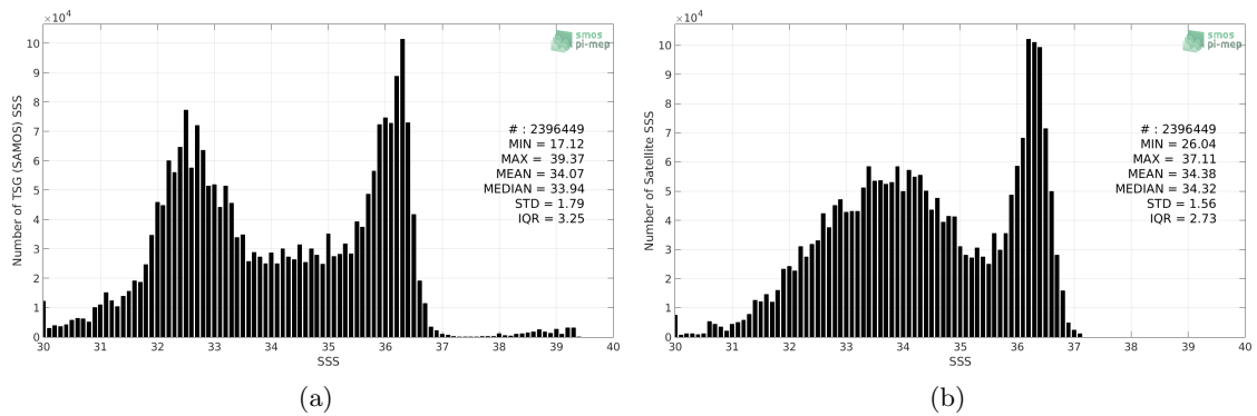
Figure 2: Histograms of SSS from TSG (SAMOS) (a) and CCI L4 Merged-OI v2.31 - 7-day running (ESA) (b) considering all match-up pairs per bins of 0.1 over the Gulf Stream Pi-MEP region and for the full satellite product period.
