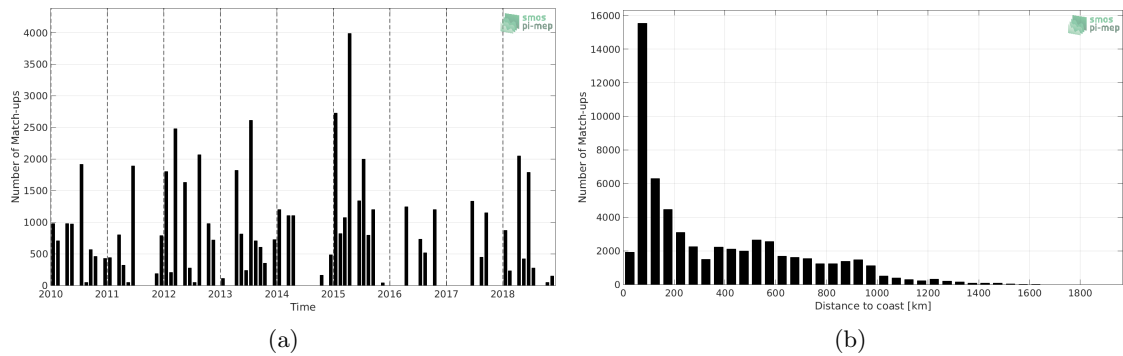
Figure 1: Number of match-ups between TSG (LEGOS-DM) and CCI SSS L4 Merged-OI v2.31 - 7-day running (ESA) SSS as a function of time (a) and as function of the distance to coast (b) over the Gulf Stream Pi-MEP region and for the full satellite product period.
