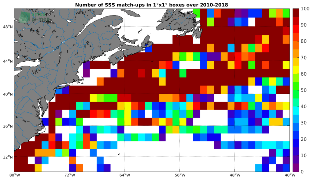
Figure 4: Number of SSS match-ups between TSG (LEGOS-DM) SSS and the CCI SSS L4 Merged-OI v2.31 - 7-day running (ESA) SSS product for the Gulf Stream Pi-MEP region over 1^\circ \times 1^\circ boxes and for the full satellite product period.
