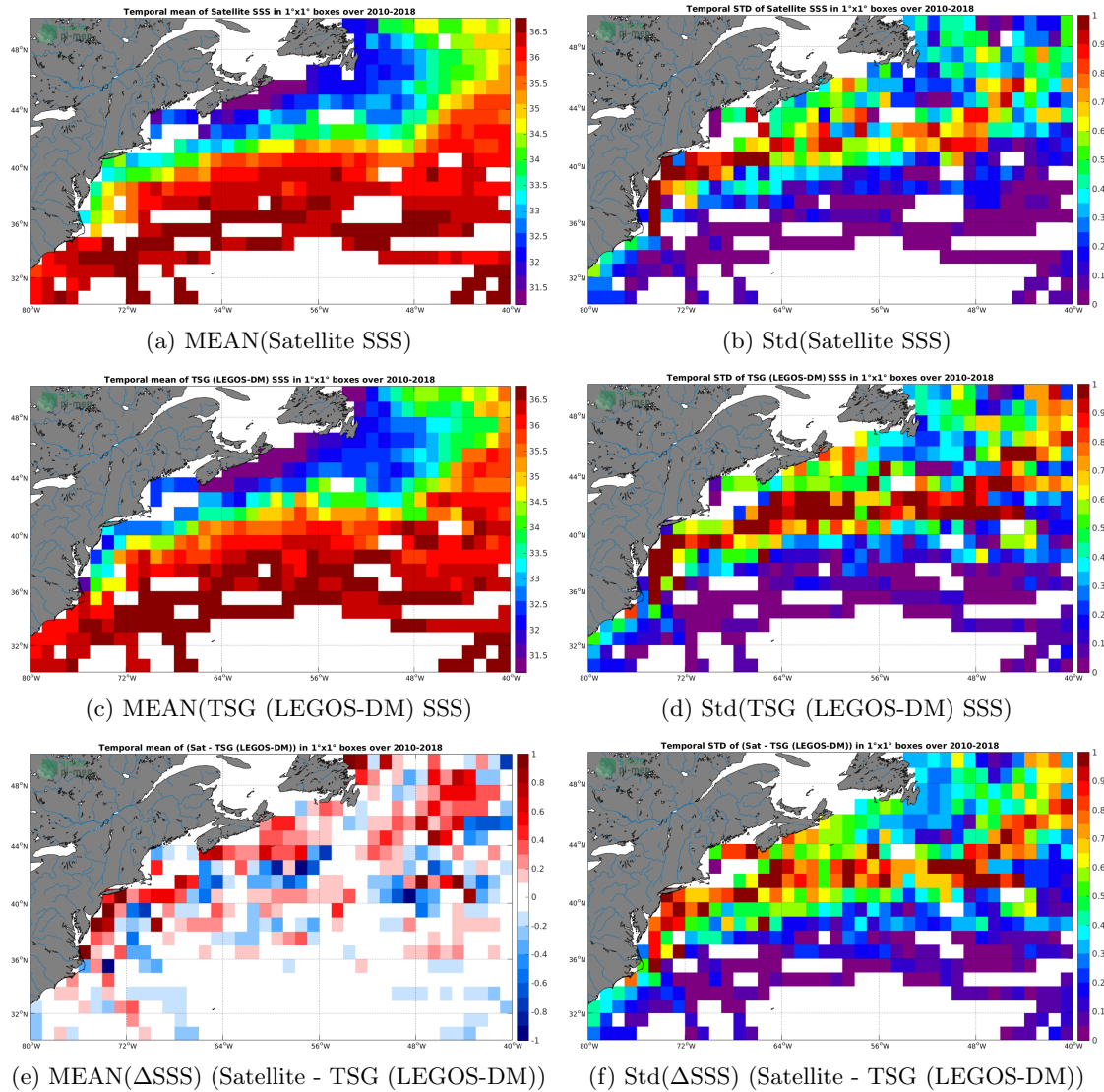
Figure 6: Temporal mean (left) and Std (right) of SSS from CCI L4 Merged-OI v2.31 - 7-day running (ESA) (top), TSG (LEGOS-DM) in situ dataset (middle), and of \Delta SSS (Satellite - TSG (LEGOS-DM)). Only match-up pairs are used to generate these maps.
