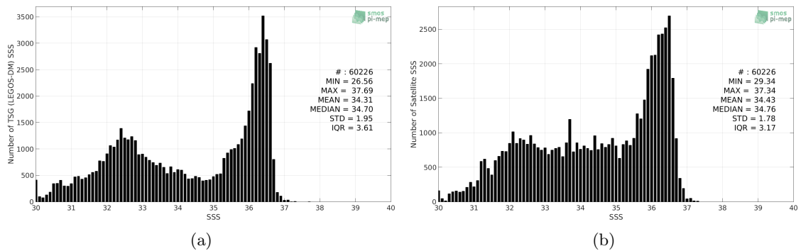
Figure 2: Histograms of SSS from TSG (LEGOS-DM) (a) and CCI L4 Merged-OI v2.31 - 7-day running (ESA) (b) considering all match-up pairs per bins of 0.1 over the Gulf Stream Pi-MEP region and for the full satellite product period.
