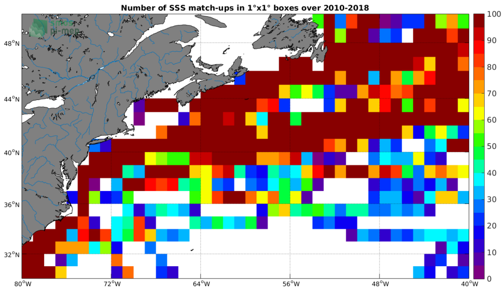
Figure 4: Number of SSS match-ups between TSG (LEGOS-DM) SSS and the CCI L4 Merged-OI v2.31 - 7-day running (ESA) SSS product for the Gulf Stream Pi-MEP region over 1^\circ \times 1^\circ boxes and for the full satellite product period.
