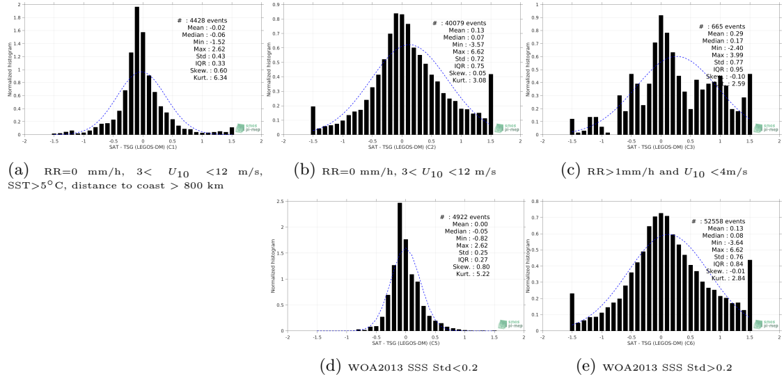
Figure 13: Normalized histogram of \Delta SSS (CCI L4 Merged-OI v2.31 - 7-day running (ESA) - TSG (LEGOS-DM)) for 5 different subdatasets corresponding to: RR=0 mm/h, 3 < U_{10} < 12 m/s, SST>5°C, distance to coast > 800 km (a), RR=0 mm/h, 3 < U_{10} < 12 m/s (b), RR>1mm/h and U_{10} < 4 m/s (c), WOA2013 SSS Std<0.2 (d), WOA2013 SSS Std>0.2 (e).
