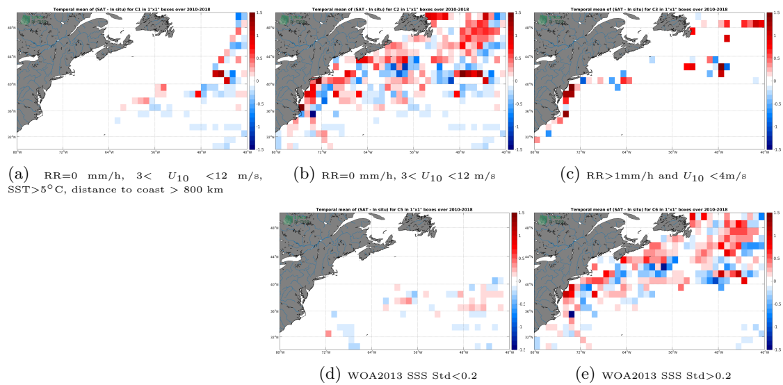
Figure 12: Temporal mean gridded over spatial boxes of size 1^\circ \times 1^\circ of \Delta SSS (CCI L4 Merged-OI v2.31 - 7-day running (ESA) - TSG (LEGOS-DM)) for 5 different subdatasets corresponding to:RR=0 mm/h, 3 < U_{10} < 12 m/s, SST >5^\circ\text{C} , distance to coast > 800 km (a), RR=0 mm/h, 3 < U_{10} < 12 m/s (b), RR >1 mm/h and U_{10} < 4 m/s (c), WOA2013 SSS Std <0.2 (d), WOA2013 SSS Std >0.2 (e).
