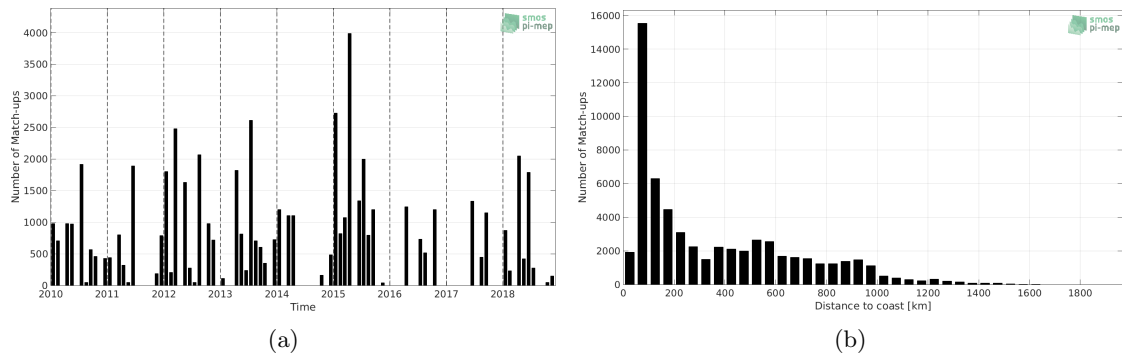
Figure 1: Number of match-ups between TSG (LEGOS-DM) and CCI L4 Merged-OI v2.31 - 7-day running (ESA) SSS as a function of time (a) and as function of the distance to coast (b) over the Gulf Stream Pi-MEP region and for the full satellite product period.
