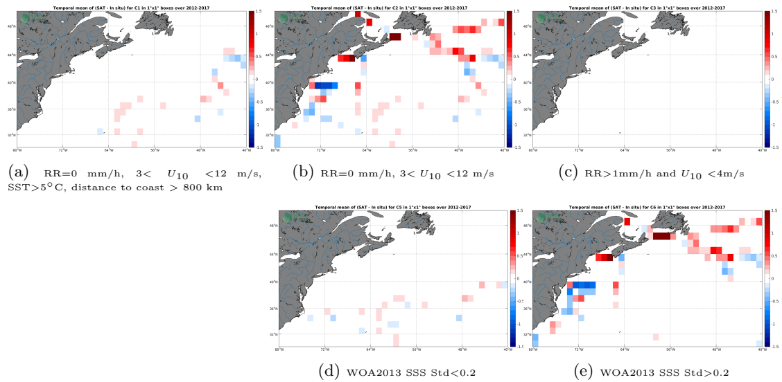
Figure 12: Temporal mean gridded over spatial boxes of size 1^\circ \times 1^\circ of \Delta SSS (CCI SSS L4 Merged-OI v2.31 - 7-day running (ESA) - TSG (GOSUD-Sailing-ship)) for 5 different subdatasets corresponding to: RR=0 mm/h, 3 < U_{10} < 12 m/s, SST >5^\circ\text{C} , distance to coast > 800 km (a), RR=0 mm/h, 3 < U_{10} < 12 m/s (b), RR >1 mm/h and U_{10} < 4 m/s (c), WOA2013 SSS Std <0.2 (d), WOA2013 SSS Std >0.2 (e).
