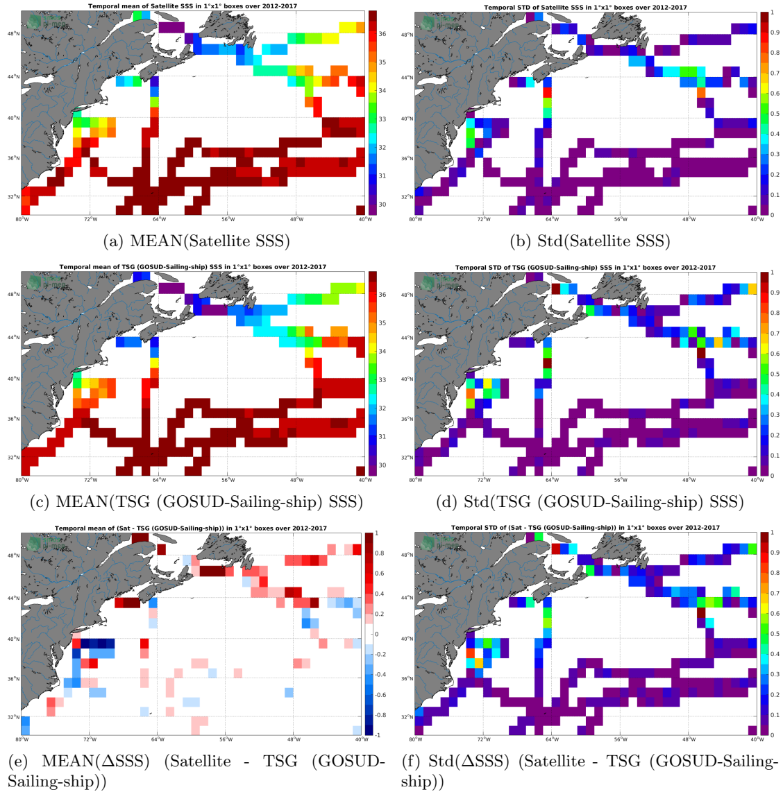
Figure 6: Temporal mean (left) and Std (right) of SSS from CCI SSS L4 Merged-OI v2.31 - 7-day running (ESA) (top), TSG (GOSUD-Sailing-ship) (middle), and of \Delta SSS (Satellite - TSG (GOSUD-Sailing-ship)). Only match-up pairs are used to generate these maps.
