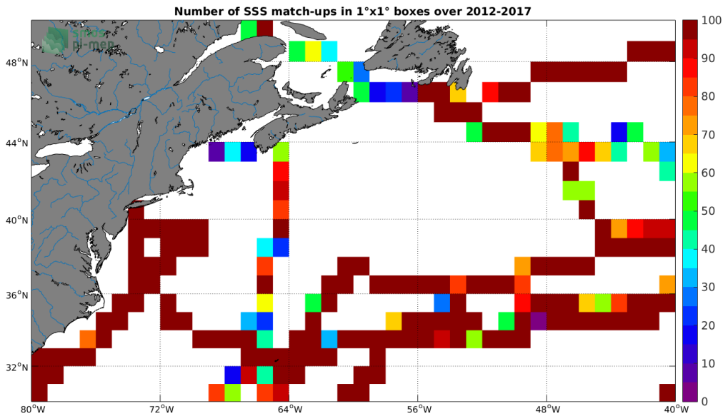
Figure 4: Number of SSS match-ups between TSG (GOSUD-Sailing-ship) SSS and the CCI SSS L4 Merged-OI v2.31 - 7-day running (ESA) SSS product for the Gulf Stream Pi-MEP region over 1^\circ \times 1^\circ boxes and for the full satellite product period.
