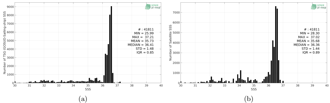
Figure 2: Histograms of SSS from TSG (GOSUD-Sailing-ship) (a) and CCI SSS L4 Merged-OI v2.31 - 7-day running (ESA) (b) considering all match-up pairs per bins of 0.1 over the Gulf Stream Pi-MEP region and for the full satellite product period.
