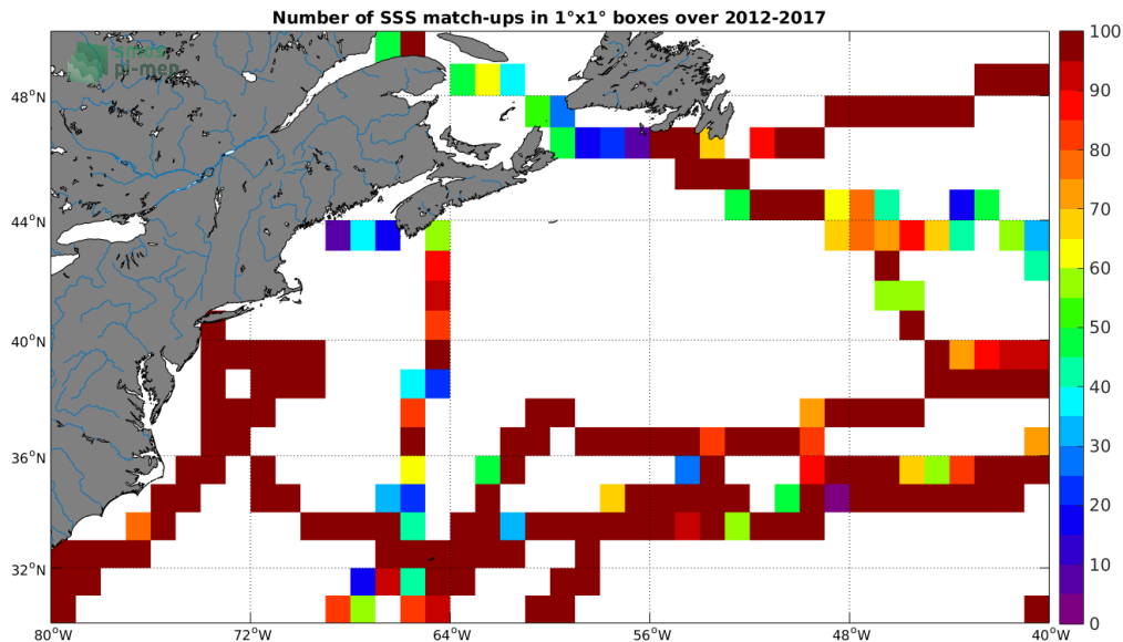
Figure 4: Number of SSS match-ups between TSG (GOSUD-Sailing-ship) SSS and the CCI L4 Merged-OI v2.31 - 7-day running (ESA) SSS product for the Gulf Stream Pi-MEP region over 1^\circ \times 1^\circ boxes and for the full satellite product period.
