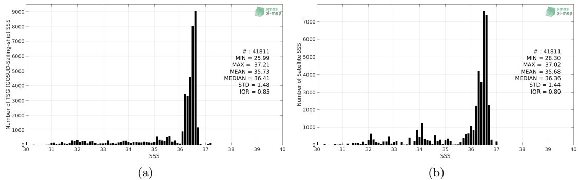
Figure 2: Histograms of SSS from TSG (GOSUD-Sailing-ship) (a) and CCI L4 Merged-OI v2.31 - 7-day running (ESA) (b) considering all match-up pairs per bins of 0.1 over the Gulf Stream Pi-MEP region and for the full satellite product period.
