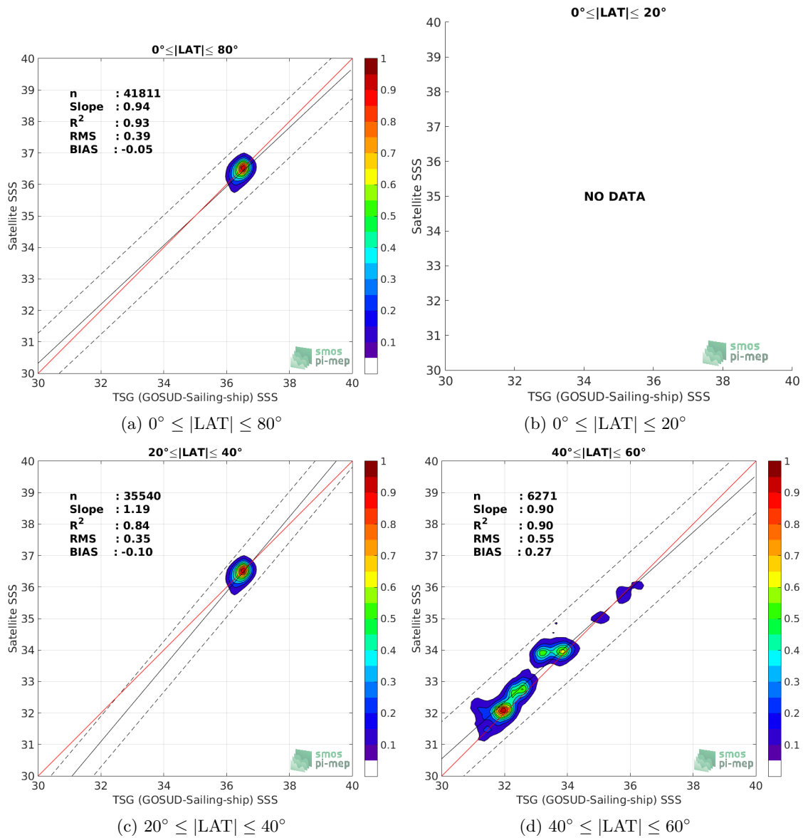
Figure 9: Contour maps of the concentration of CCI L4 Merged-OI v2.31 - 7-day running (ESA) SSS (y-axis) versus TSG (GOSUD-Sailing-ship) SSS (x-axis) at match-up pairs for different latitude bands. For each plot, the red line shows x=y . The black thin and dashed lines indicate a linear fit through the data cloud and the \pm 95\% confidence levels, respectively. The number match-up pairs n , the slope and R^2 coefficient of the linear fit, the root mean square (RMS) and the mean bias between satellite and in situ data are indicated for each latitude band in each plots.
