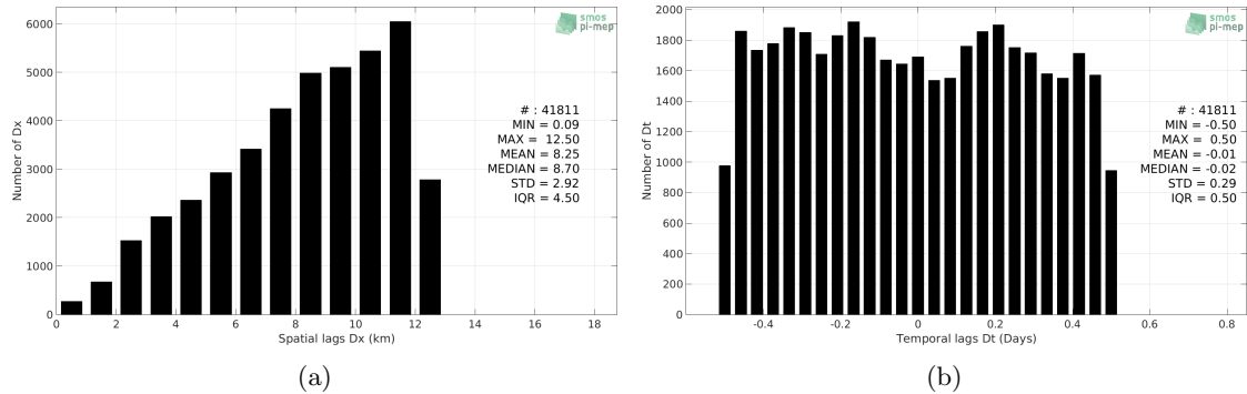
Figure 5: Histograms of the spatial (a) and temporal (b) lags between the time of the TSG (GOSUD-Sailing-ship) measurements and the date of the corresponding CCI L4 Merged-OI v2.31 - 7-day running (ESA) SSS product.
