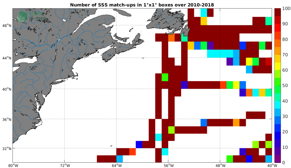
Figure 4: Number of SSS match-ups between TSG (GOSUD-Research-vessel) SSS and the CCI L4 Merged-OI v2.31 - 7-day running (ESA) SSS product for the Gulf Stream Pi-MEP region over 1^\circ \times 1^\circ boxes and for the full satellite product period.
