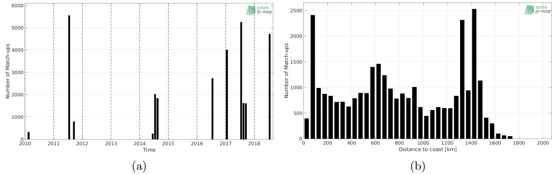
Figure 1: Number of match-ups between TSG (GOSUD-Research-vessel) and CCI L4 Merged-OI v2.31 - 7-day running (ESA) SSS as a function of time (a) and as function of the distance to coast (b) over the Gulf Stream Pi-MEP region and for the full satellite product period.
