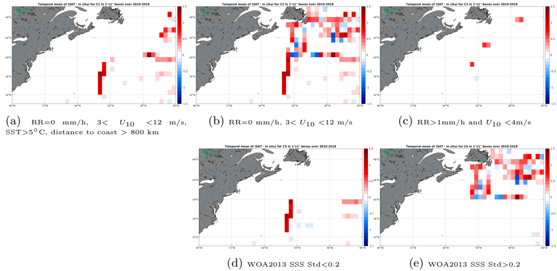
Figure 12: Temporal mean gridded over spatial boxes of size 1^\circ \times 1^\circ of \Delta SSS (CCI L4 Merged-OI v2.31 - 7-day running (ESA) - TSG (GOSUD-Research-vessel)) for 5 different subdatasets corresponding to:RR=0 mm/h, 3 < U_{10} < 12 m/s, SST >5^\circ\text{C} , distance to coast > 800 km (a), RR=0 mm/h, 3 < U_{10} < 12 m/s (b), RR >1 mm/h and U_{10} < 4 m/s (c), WOA2013 SSS Std <0.2 (d), WOA2013 SSS Std >0.2 (e).
