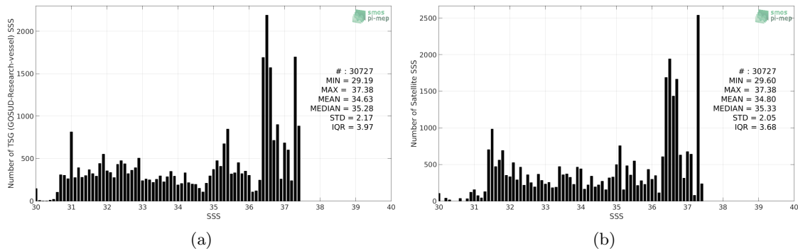
Figure 2: Histograms of SSS from TSG (GOSUD-Research-vessel) (a) and CCI L4 Merged-OI v2.31 - 7-day running (ESA) (b) considering all match-up pairs per bins of 0.1 over the Gulf Stream Pi-MEP region and for the full satellite product period.
