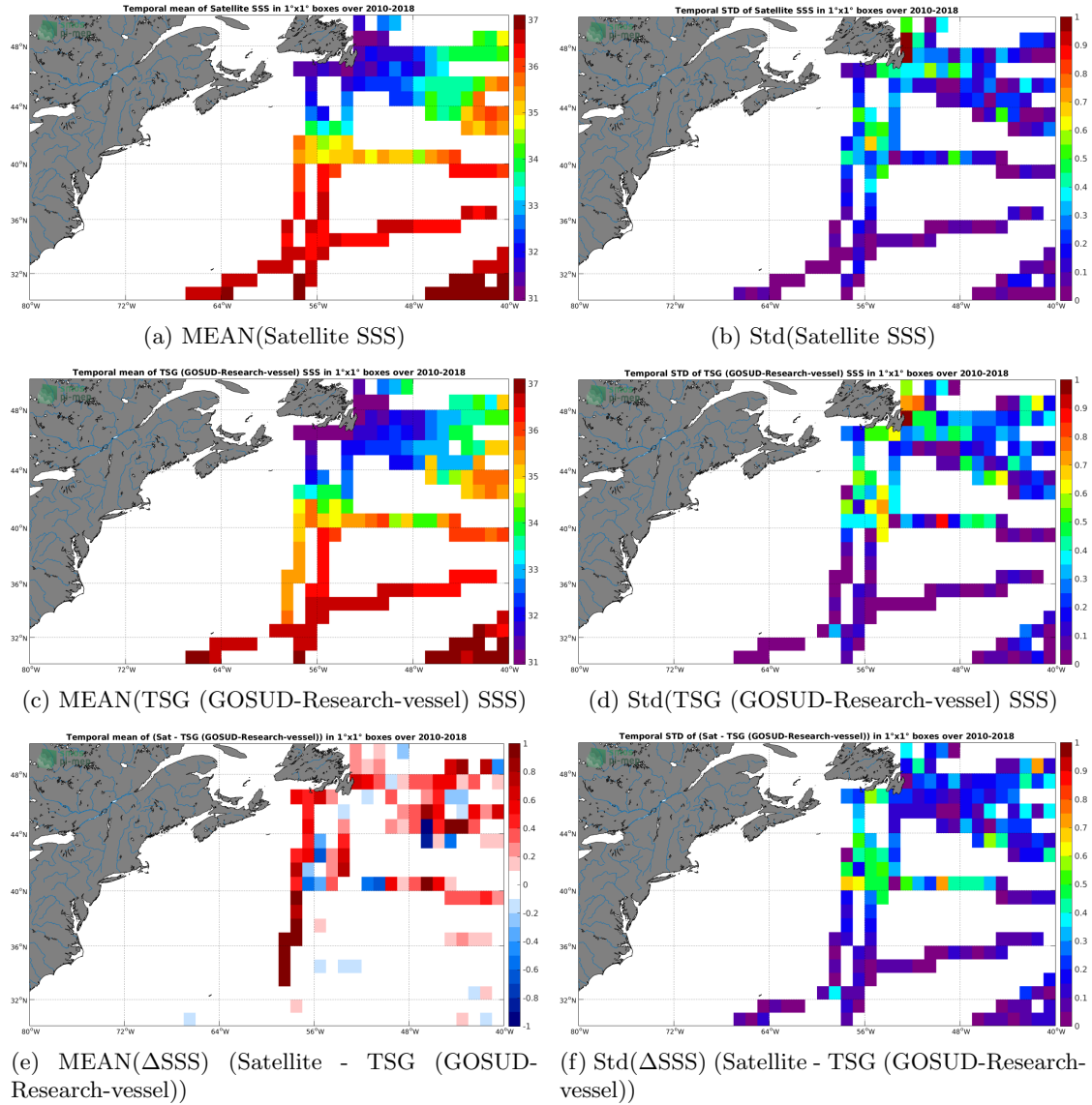
Figure 6: Temporal mean (left) and Std (right) of SSS from CCI L4 Merged-OI v2.31 - 7-day running (ESA) (top), TSG (GOSUD-Research-vessel) (middle), and of \Delta SSS (Satellite - TSG (GOSUD-Research-vessel)). Only match-up pairs are used to generate these maps.
