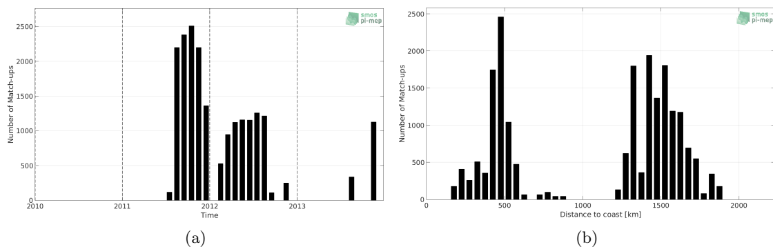
Figure 1: Number of match-ups between Surface drifters and CCI SSS L4 Merged-OI v2.31 - 7-day running (ESA) SSS as a function of time (a) and as function of the distance to coast (b) over the Gulf Stream Pi-MEP region and for the full satellite product period.
