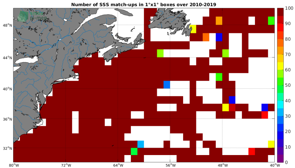
Figure 4: Number of SSS match-ups between TSG (SAMOS) SSS and the CCI L4 Merged-OI v2.31 - 30-day running (ESA) SSS product for the Gulf Stream Pi-MEP region over 1^\circ \times 1^\circ boxes and for the full satellite product period.
