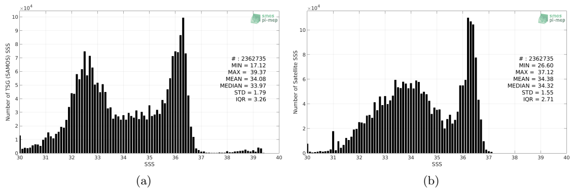
Figure 2: Histograms of SSS from TSG (SAMOS) (a) and CCI L4 Merged-OI v2.31 - 30-day running (ESA) (b) considering all match-up pairs per bins of 0.1 over the Gulf Stream Pi-MEP region and for the full satellite product period.
