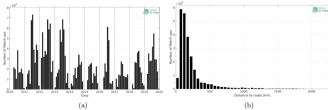
Figure 1: Number of match-ups between TSG (SAMOS) and CCI L4 Merged-OI v2.31 - 30-day running (ESA) SSS as a function of time (a) and as function of the distance to coast (b) over the Gulf Stream Pi-MEP region and for the full satellite product period.
