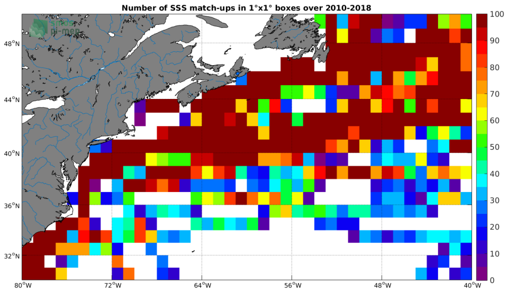
Figure 4: Number of SSS match-ups between TSG (LEGOS-DM) SSS and the CCI SSS L4 Merged-OI v2.31 - 30-day running (ESA) SSS product for the Gulf Stream Pi-MEP region over 1^\circ \times 1^\circ boxes and for the full satellite product period.
