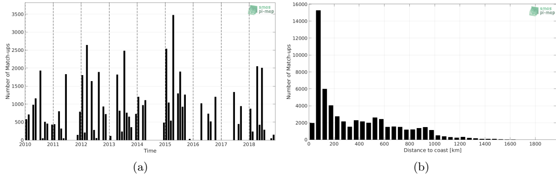
Figure 1: Number of match-ups between TSG (LEGOS-DM) and CCI SSS L4 Merged-OI v2.31 - 30-day running (ESA) SSS as a function of time (a) and as function of the distance to coast (b) over the Gulf Stream Pi-MEP region and for the full satellite product period.
