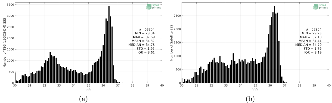
Figure 2: Histograms of SSS from TSG (LEGOS-DM) (a) and CCI SSS L4 Merged-OI v2.31 - 30-day running (ESA) (b) considering all match-up pairs per bins of 0.1 over the Gulf Stream Pi-MEP region and for the full satellite product period.
