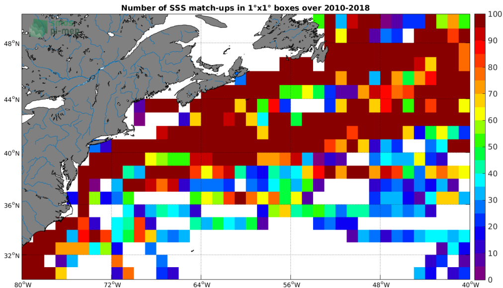
Figure 4: Number of SSS match-ups between TSG (LEGOS-DM) SSS and the CCI L4 Merged-OI v2.31 - 30-day running (ESA) SSS product for the Gulf Stream Pi-MEP region over 1^\circ \times 1^\circ boxes and for the full satellite product period.
