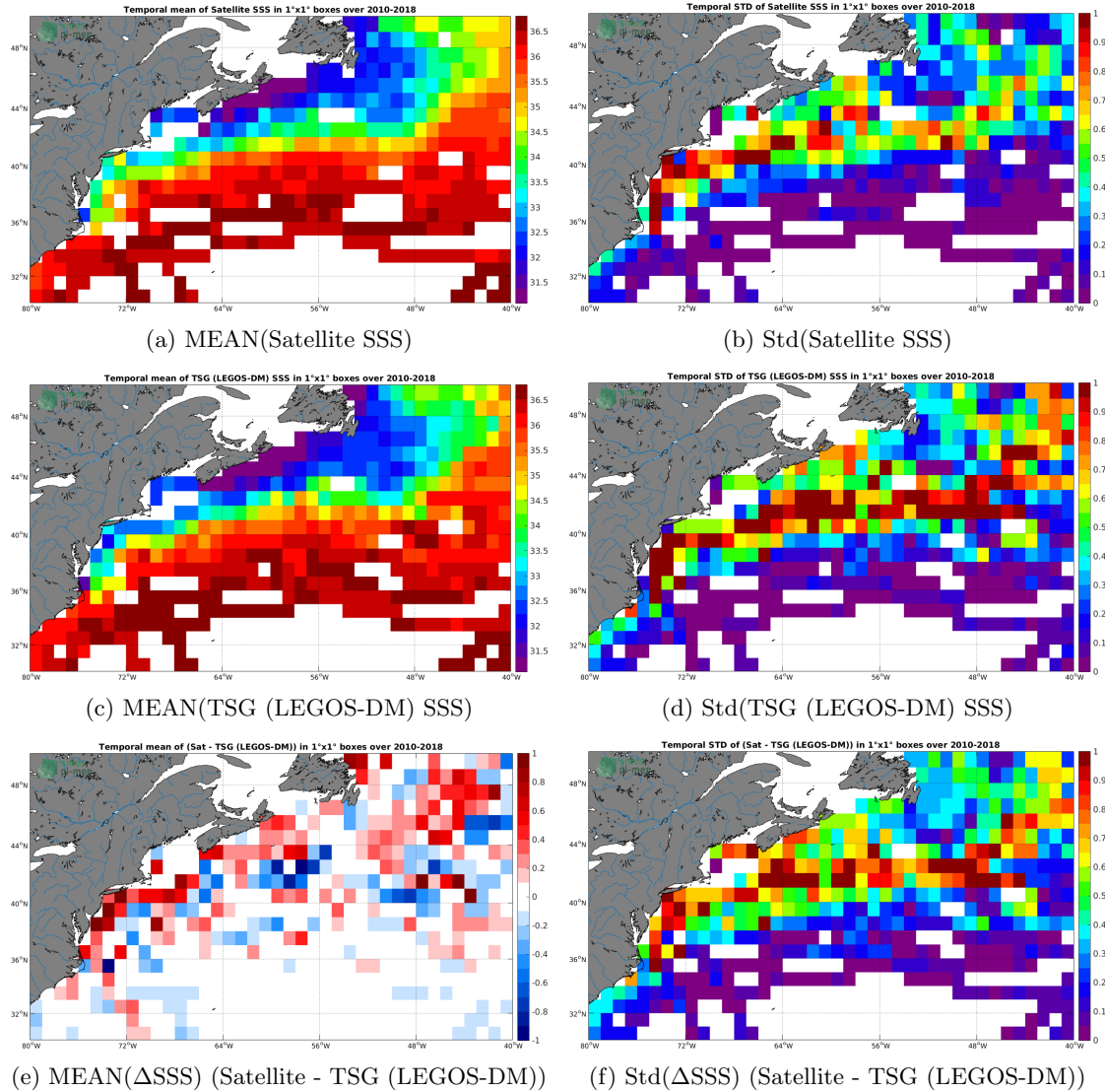
Figure 6: Temporal mean (left) and Std (right) of SSS from CCI L4 Merged-OI v2.31 - 30-day running (ESA) (top), TSG (LEGOS-DM) (middle), and of \Delta SSS (Satellite - TSG (LEGOS-DM)). Only match-up pairs are used to generate these maps.
