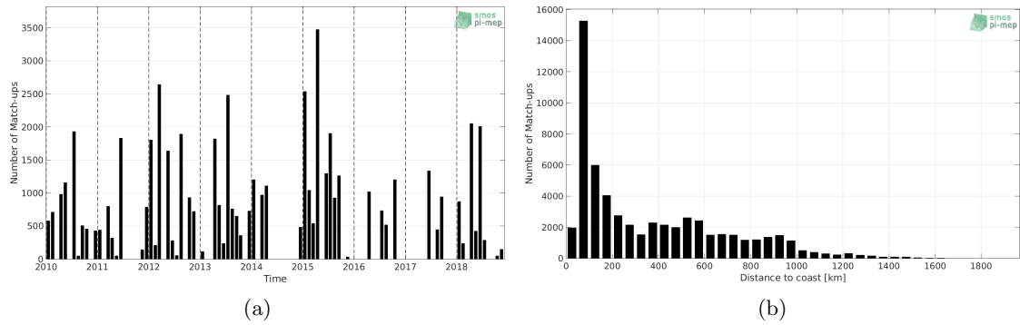
Figure 1: Number of match-ups between TSG (LEGOS-DM) and CCI L4 Merged-OI v2.31 - 30-day running (ESA) SSS as a function of time (a) and as function of the distance to coast (b) over the Gulf Stream Pi-MEP region and for the full satellite product period.
