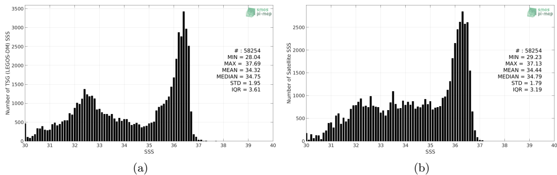
Figure 2: Histograms of SSS from TSG (LEGOS-DM) (a) and CCI L4 Merged-OI v2.31 - 30-day running (ESA) (b) considering all match-up pairs per bins of 0.1 over the Gulf Stream Pi-MEP region and for the full satellite product period.
